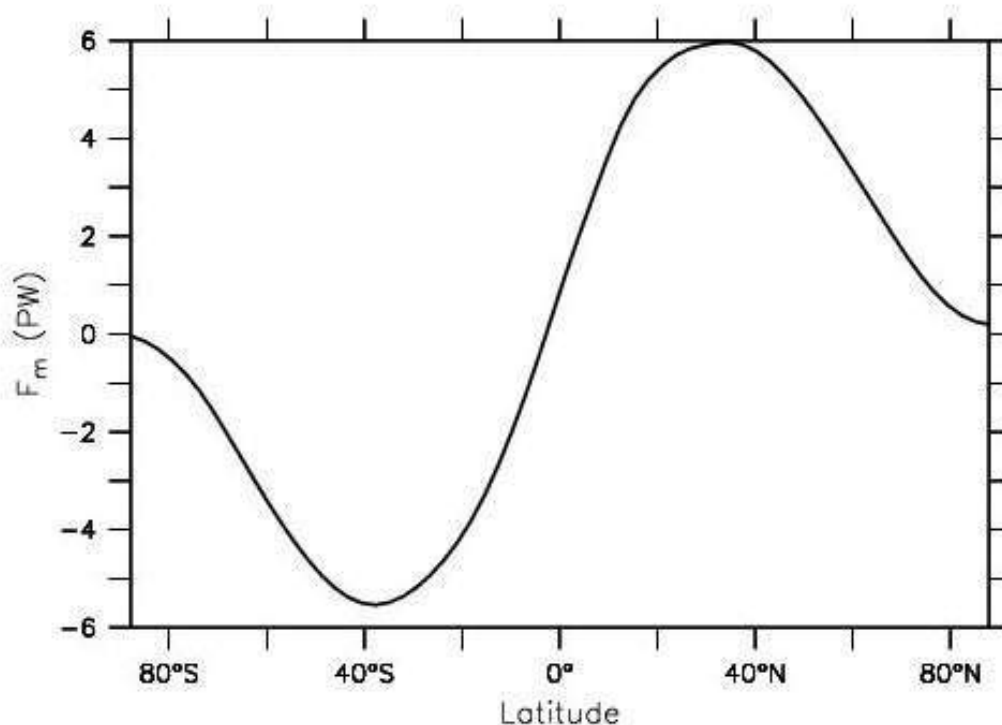
Figure 4: Meridional (northward is positive) heat transport in the climate system as a function of latitude implied from integration of the differences in the fluxes shown in Fig. 3. Units are peta watts (1 PW = 10^{15} W).
