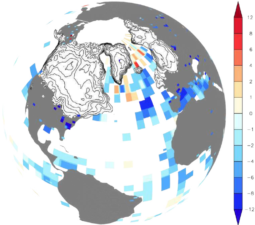
Figure 10: Reconstructions of ice sheets (contour lines show 500 m elevation differences) and surface temperature differences from modern (color scale in K) for the Last Glacial Maximum. From PAGES news .
