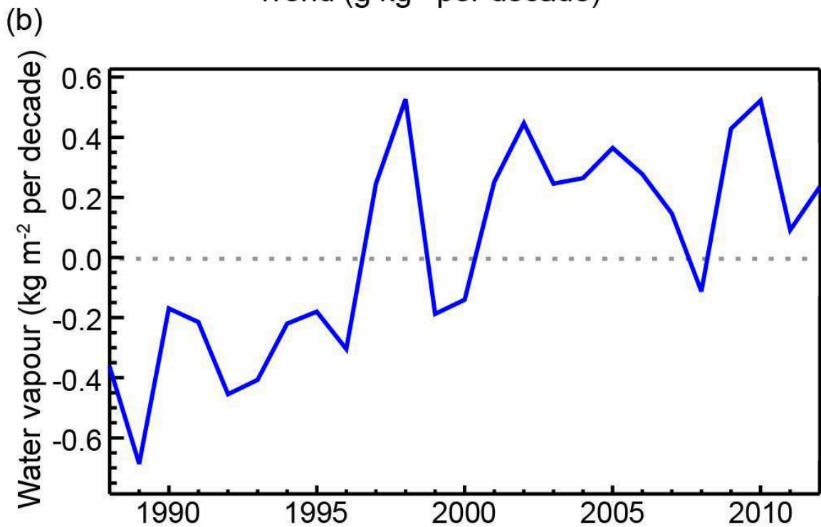
Figure 15. (a) Observed changes in surface specific humidity estimated from satellites. Dark shading indicates significant changes. (b) Changes in globally averaged water vapor content. From Harmann et al. (2013). Image from ipcc.ch .
