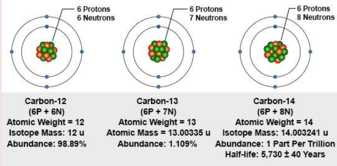
Figure B2.1: Illustration of the Atomic Structure of Carbon Isotopes. The nucleus consists of protons (red) and neutrons (green). It is surrounded by electrons (blue).
