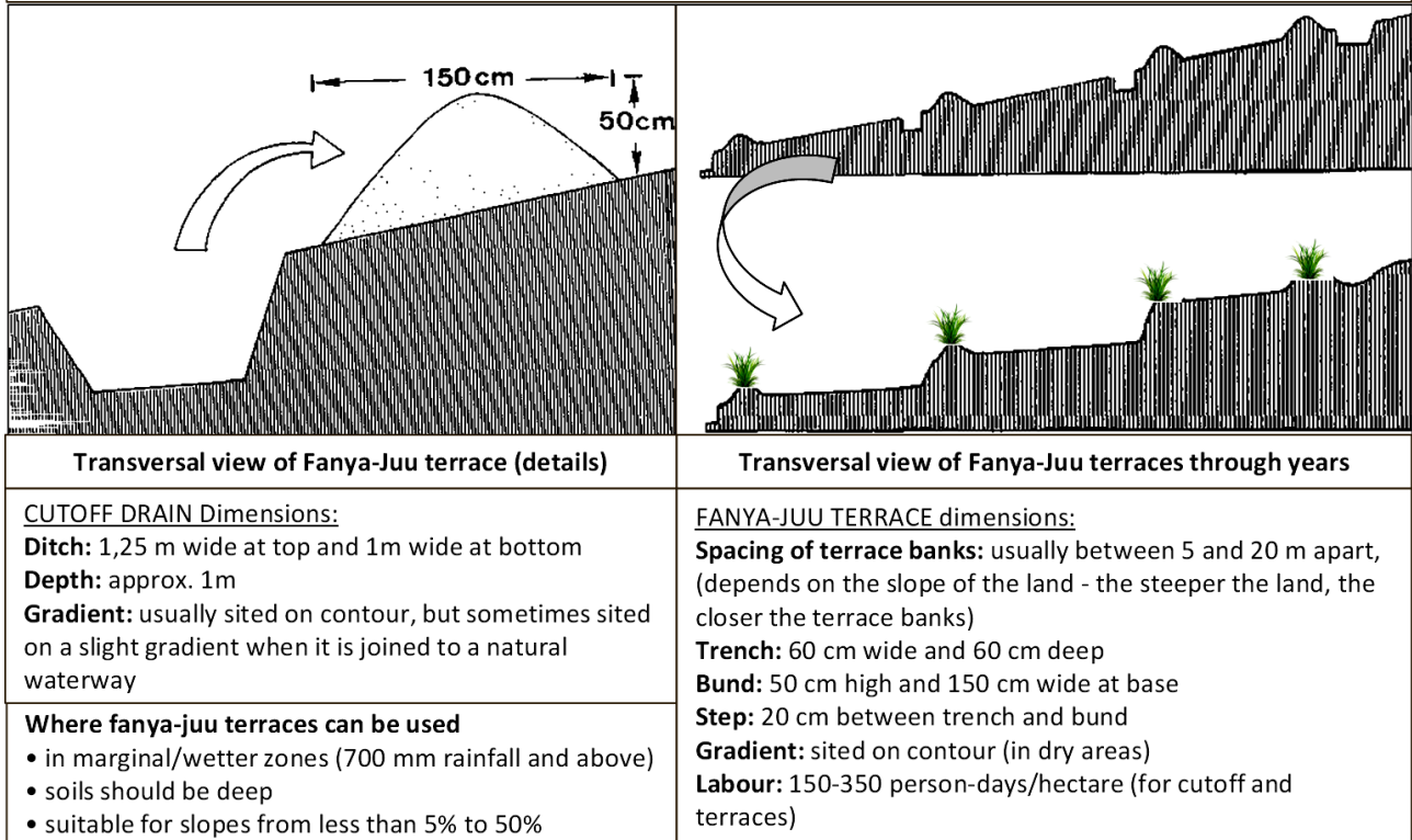
FIGURE 2-9 - FANYA-JUU TERRACES TECHNIQUES OF KENYA
