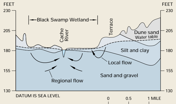
Figure 1-3. The Cache River in Arkansas provides an example of contributions to a river from regional and local ground-water flow systems. In addition, a small local ground-water flow system associated with a terrace discharges to the wetland at the edge of the flood plain. (Modified from Gonther, G.J., 1996, Ground-water flow conditions within a bottomland hardwood wetland, eastern Arkansas: Wetlands , v. 16, no. 3, p. 334–346.) (Used with permission.)
