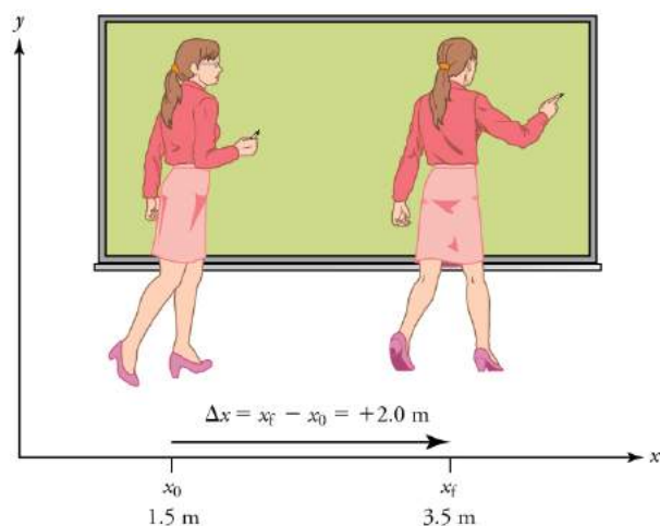
FIGURE 2.3 A professor paces left and right while lecturing. Her position relative to Earth is given by x . The +2.0 -m displacement of the professor relative to Earth is represented by an arrow pointing to the right.
