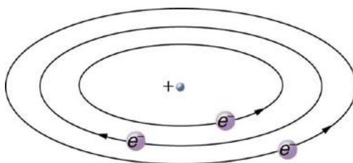
FIGURE 30.12 Rutherford’s planetary model of the atom incorporates the characteristics of the nucleus, electrons, and the size of the atom. This model was the first to recognize the structure of atoms, in which low-mass electrons orbit a very small, massive nucleus in orbits much larger than the nucleus. The atom is mostly empty and is analogous to our planetary system.
