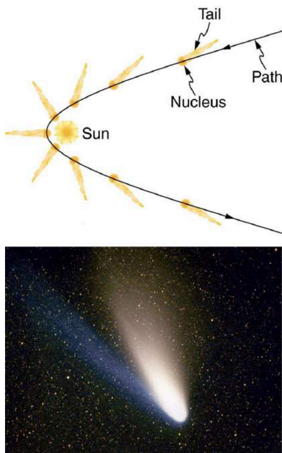
FIGURE 29.14 The tails of the Hale-Bopp comet point away from the Sun, evidence that light has momentum. Dust emanating from the body of the comet forms this tail. Particles of dust are pushed away from the Sun by light reflecting from them. The blue ionized gas tail is also produced by photons interacting with atoms in the comet material. (credit: Geoff Chester, U.S. Navy, via Wikimedia Commons)
