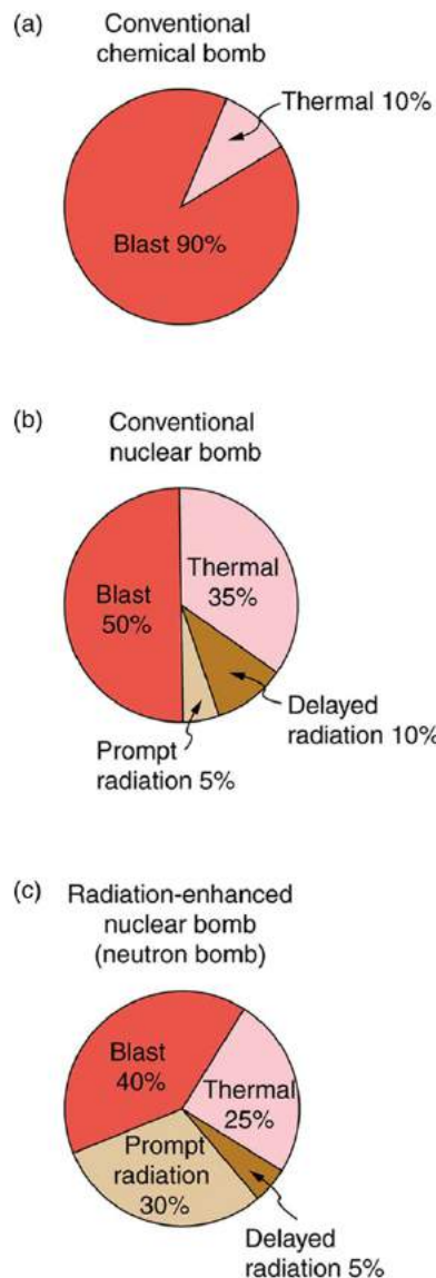
FIGURE 32.29 Approximate fractions of energy output by conventional and two types of nuclear weapons. In addition to yielding more energy than conventional weapons, nuclear bombs put a much larger fraction into thermal energy. This can be adjusted to enhance the radiation output to be more effective against troops. An enhanced radiation bomb is also called a neutron bomb.
