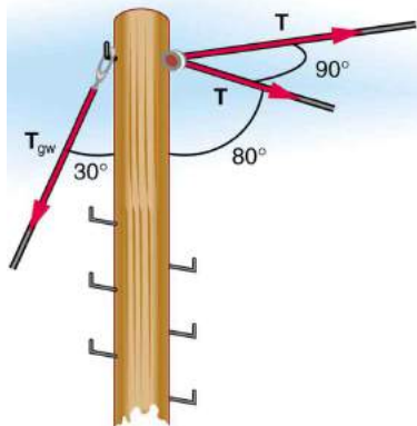
FIGURE 5.22 This telephone pole is at a 90^\circ bend in a power line. A guy wire is attached to the top of the pole at an angle of 30^\circ with the vertical.
