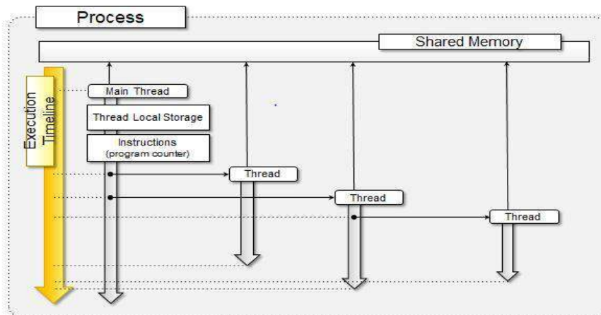
Fig20: Thread
