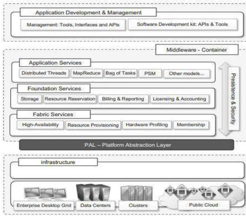
Fig 19: Services
