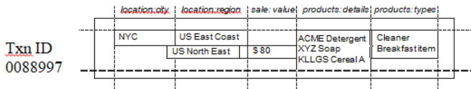
FIGURE 4.9. Data organization in a BigTable
