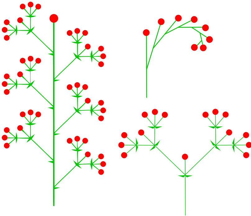
Figure 8.16. Model II inflorescences (from top to bottom): thyrus, dichasium and monochasium (cincinnus).
