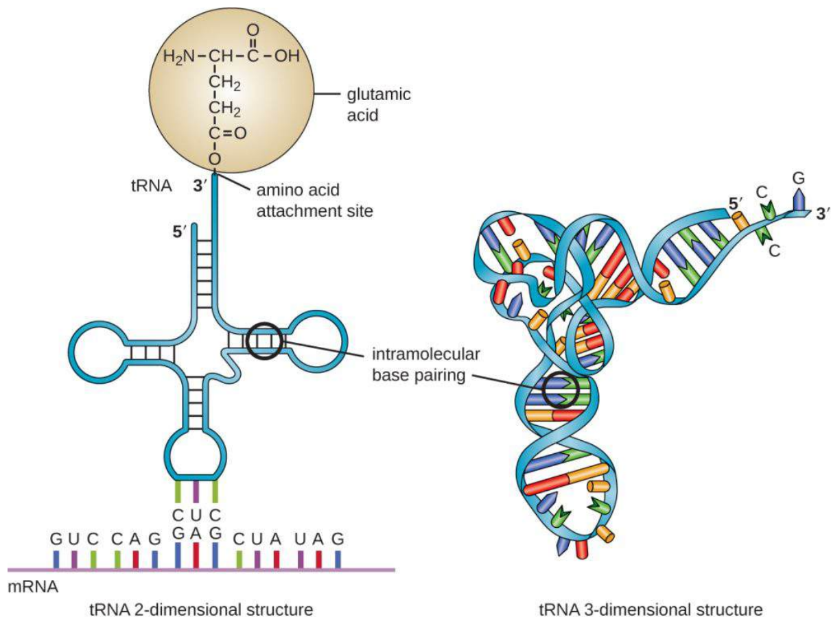
Figure 10 tRNA structure.
