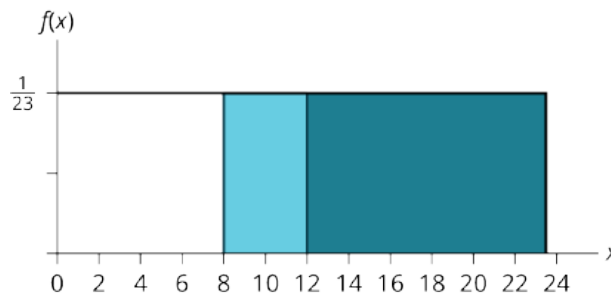
Figure 5.14 Darker shaded area represents P(x > 12) . Entire shaded area shows P(x > 8) .
