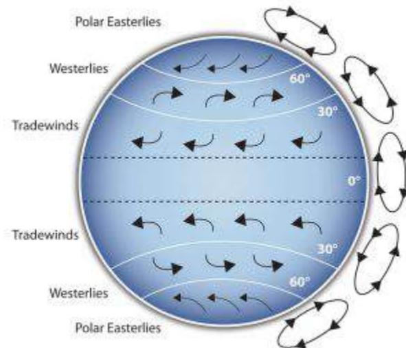
Figure 12.1 – Coriolis Effect
