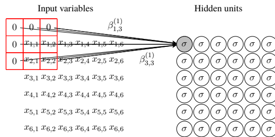
Figure 7.9: An illustration of zero-padding. If the region is partly is outside the image. With zero-padding, the size of the image can be preserved in the following layer.
