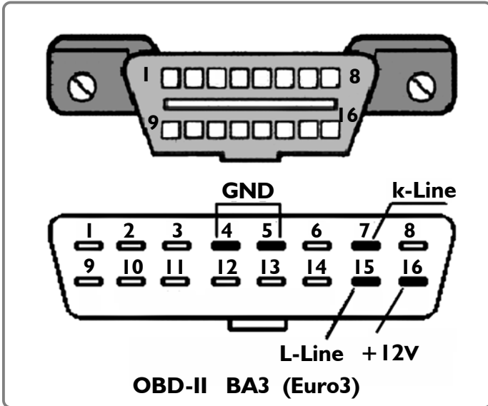
Figura 2-17 Conector trapezoidal de 16 pines
