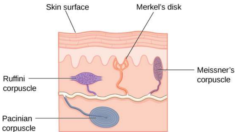
Figure SAP.24 There are many types of sensory receptors located in the skin, each attuned to specific touch-related stimuli.
