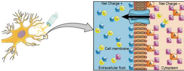
Figure BB.4 At resting potential, Na + (blue pentagons) is more highly concentrated outside the cell in the extracellular fluid (shown in blue), whereas K + (purple squares) is more highly concentrated near the membrane in the cytoplasm or intracellular fluid. Other molecules, such as chloride ions (yellow circles) and negatively charged proteins (brown squares), help contribute to a positive net charge in the extracellular fluid and a negative net charge in the intracellular fluid.
