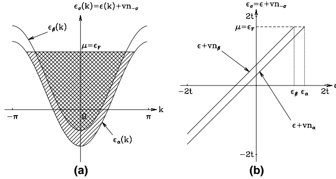
Figure 9.2: (a) Relative position of the two energy sub-bands \epsilon_\alpha(k) and \epsilon_\beta(k) for \Delta = n_\alpha - n_\beta > 0 . The shaded areas represent the filled portions of these bands by electrons. (b) Graphical definition of the limiting energies \epsilon_\alpha and \epsilon_\beta .
