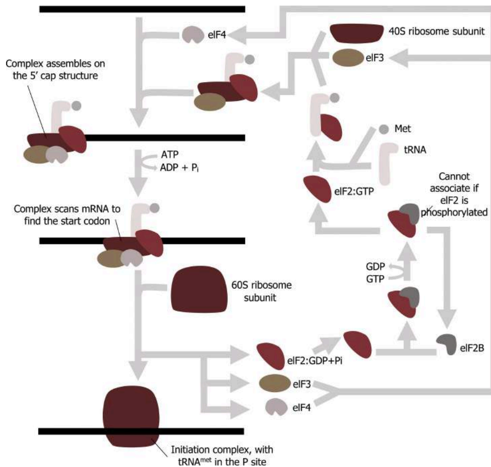
Figure 11.7: Summary of translational initiation. eIF4 recruits the small ribosomal subunit and other initiation factors to the mRNA. The charge Met-tRNA also binds the complex, and the large ribosomal subunit is recruited to the initiation complex. Once the large ribosomal subunit binds, the initiation factors can be released, and translation can proceed to elongation of the polypeptide chain.
