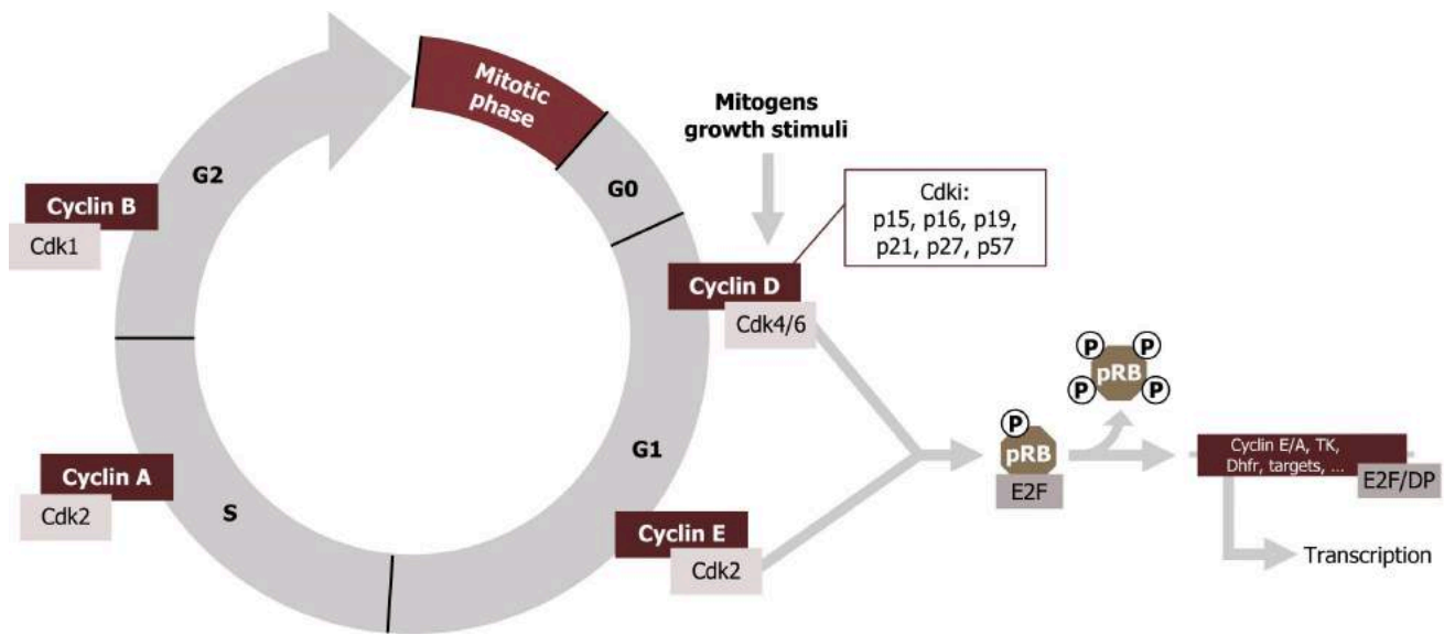
Figure 12.9: Summary of cell cycle checkpoints and the role of CDK inhibitors in halting cell cycle progress.
