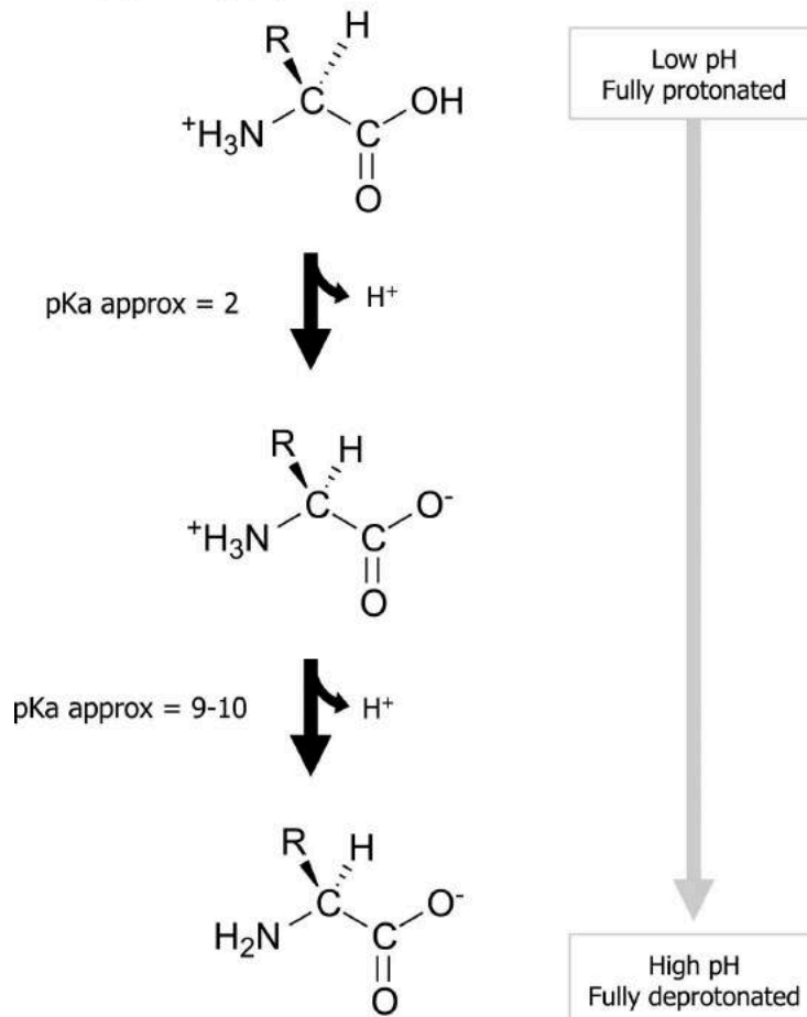
Figure 1.1: Basic structure of amino acids and ionization.
