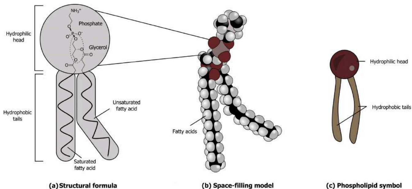
Figure 16.2: Structure of a phospholipid.
