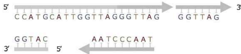
Figure 10.8: Summary of telomerase activity to fill the overhang on the lagging strand.
