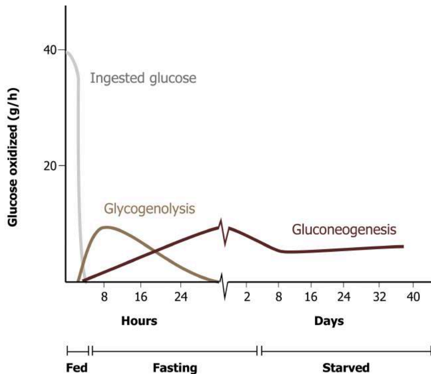
Figure 5.1: Glucose production by glycogenolysis and gluconeogenesis.
