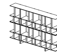
Double Horizontal Size: W2000xD316xH1280mm
