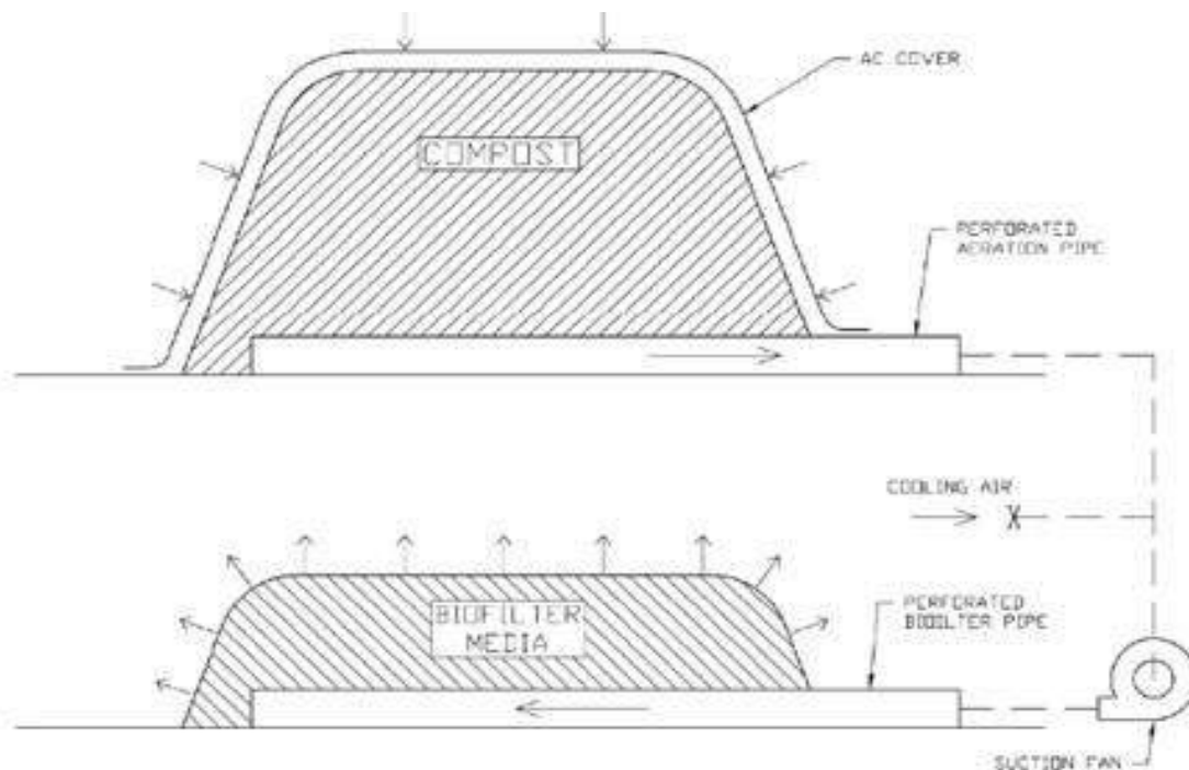
REACTOR COMPOSTING
