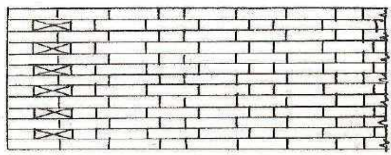
Elevation of wall in Flemish garden wall bond
