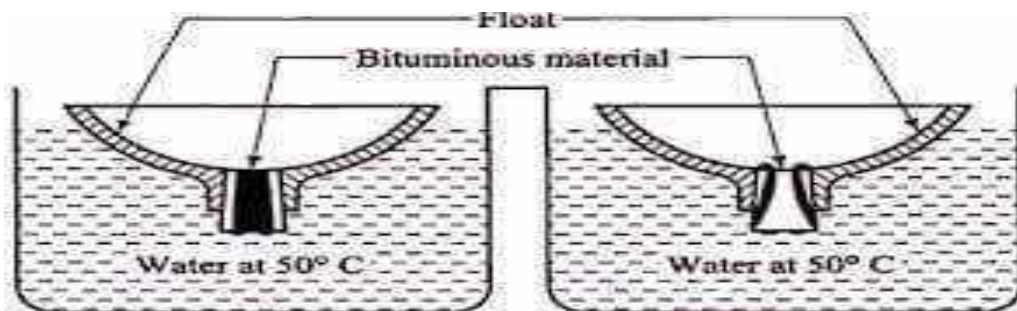
Float test FIG. 17-2
