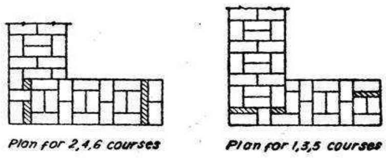
Two-bricks double flemish bond.
