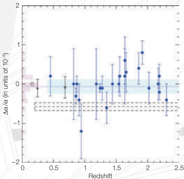
The variability of the fine structure constant is not yet proved and awaits the extreme sensitivity of the E-ELT.
