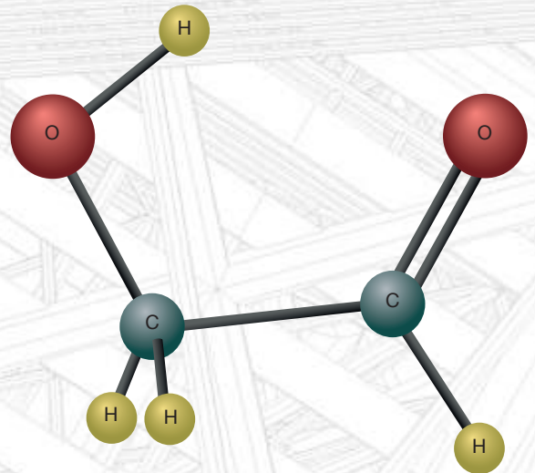
Glycolaldehyde
