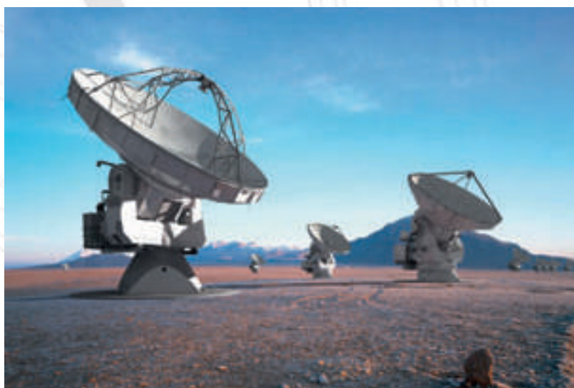
ALMA is the largest astronomical project in existence and will start observing the southern sky in 2011.
