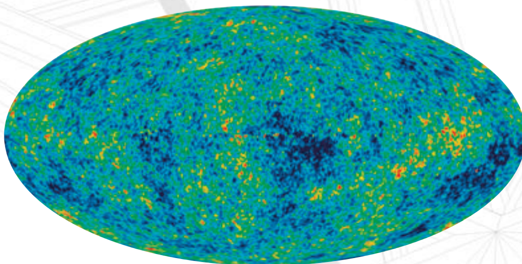
-200 T (μK) +200 WMAP 5-year
