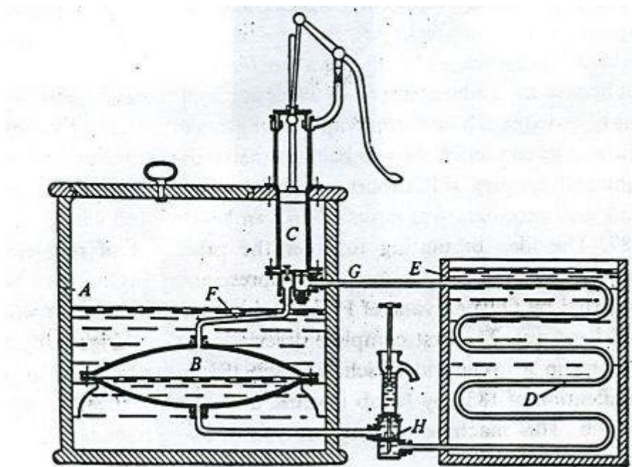
Fig. 1.1. Apparatus described by Jacob Perkins in his patent specification of 1834. The refrigerant (ether or other volatile fluid) boils in evaporator B taking heat from surrounding water in container A. The pump C draws vapour away and compresses it to higher pressure at which it can condense to liquids in tubes D, giving out heat to water in vessel E. Condensed liquid flows through the weight loaded valve H, which maintains the difference of pressure between the condenser and evaporator. The small pump above H is used for charging the apparatus with refrigerant.
