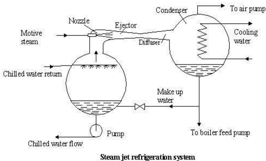
Fig.1.7. Schematic of a steam jet refrigeration system
