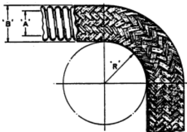
Figura 6-34 Jaqueta de fluorocarbono
