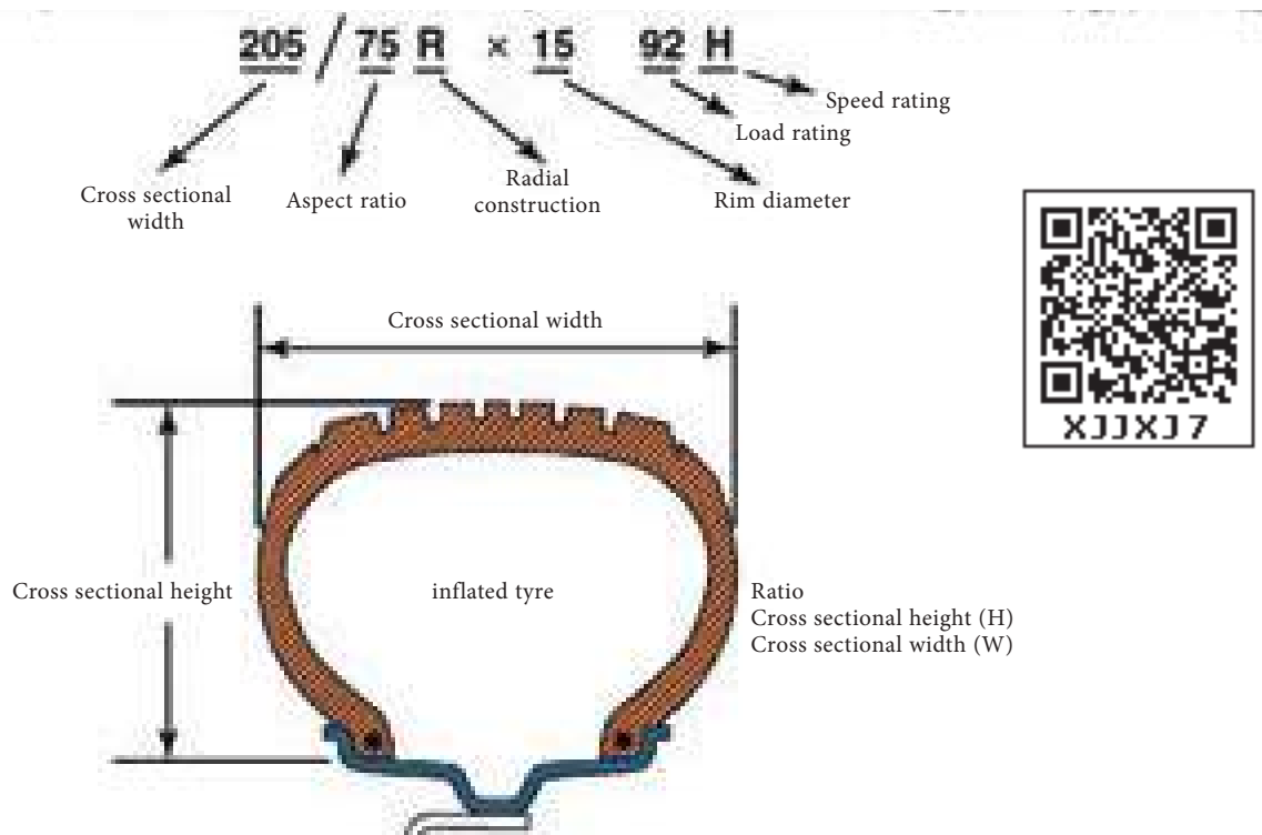
Figure 5.10.1 The tyre specifications.
