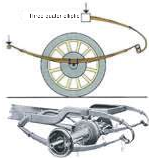
Figure 7.1.1.1 (c) Three quarter elliptic leaf spring
