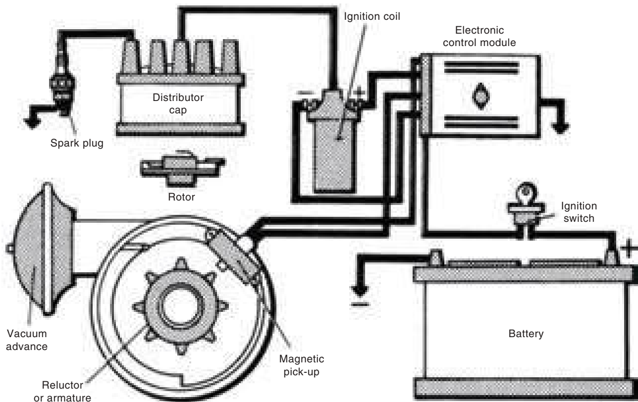
Figure 10.2.1.3 (c) Electronic ignition system
