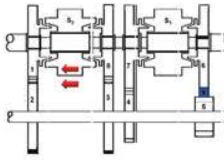
Figure 3.5.3.4 Third gear condition
