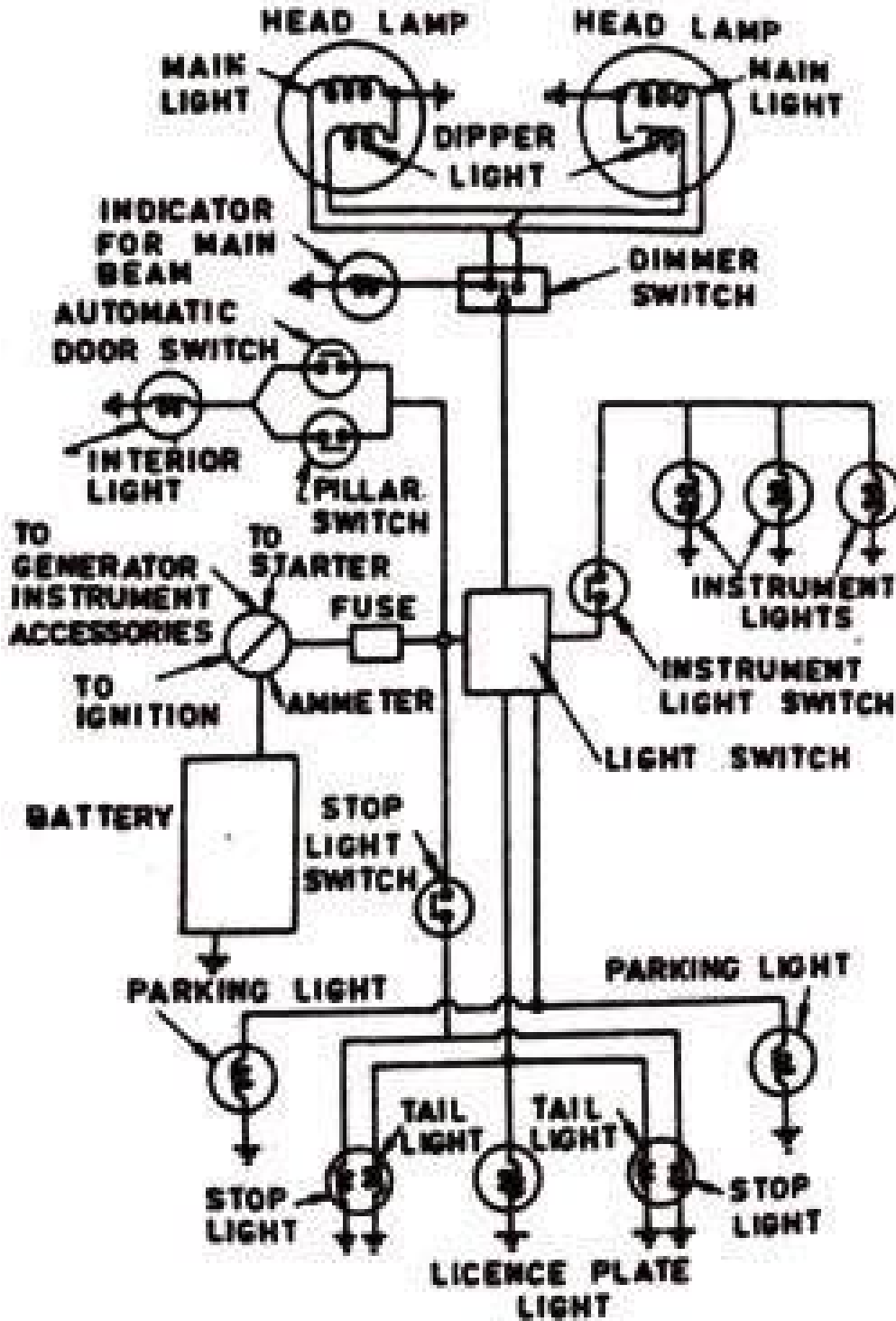
Figure 10.10.2 Lighting system
