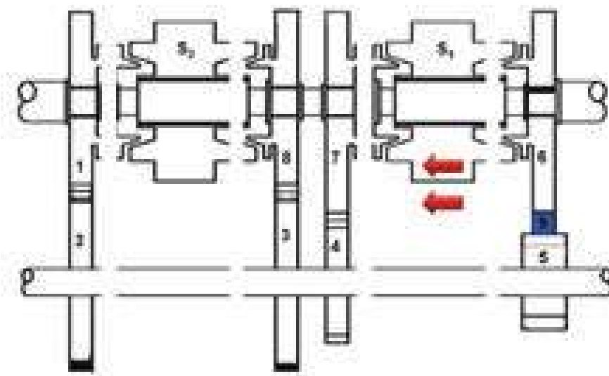
Figure 3.5.3.2 First gear condition
