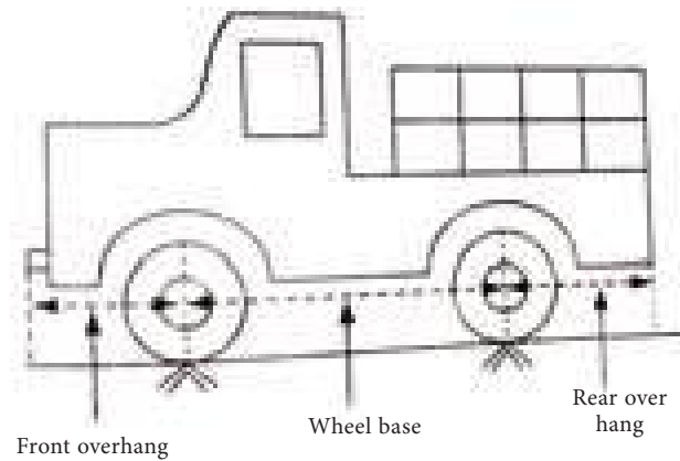
Figure 9.3.1 Wheel base
