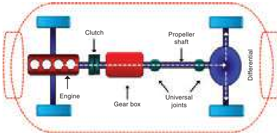
Figure 1.3.1 Front engine rear wheel drive
