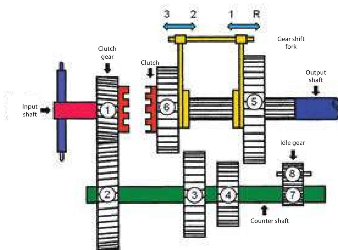
Figure 3.5.1 Sliding mesh gear box
