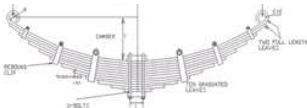
Figure 7.1.1 Leaf Spring
