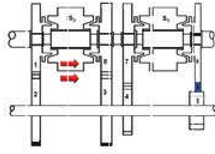
Figure 3.5.3.3 Second gear condition
