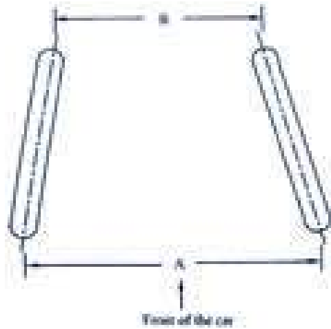
Figure 8.9.2.4 (b) Toe-out
