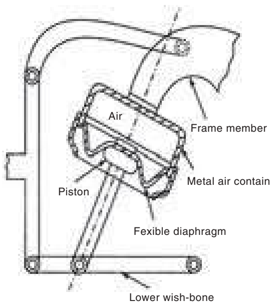
Figure 7.1.3 (2) Piston Type
