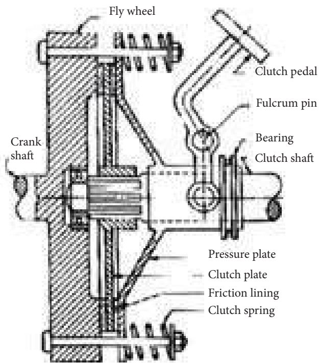
Figure 2.5.1 (c) Single plate clutch
