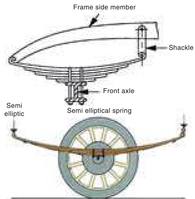
Figure 7.1.1.1 (b) Semi-elliptical leaf spring
