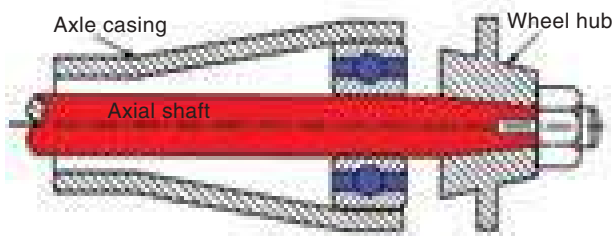
Figure 4.13.1 Semi-floating axle
