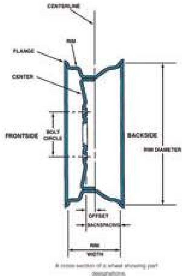
Figure 5.4 Wheel Dimensions
