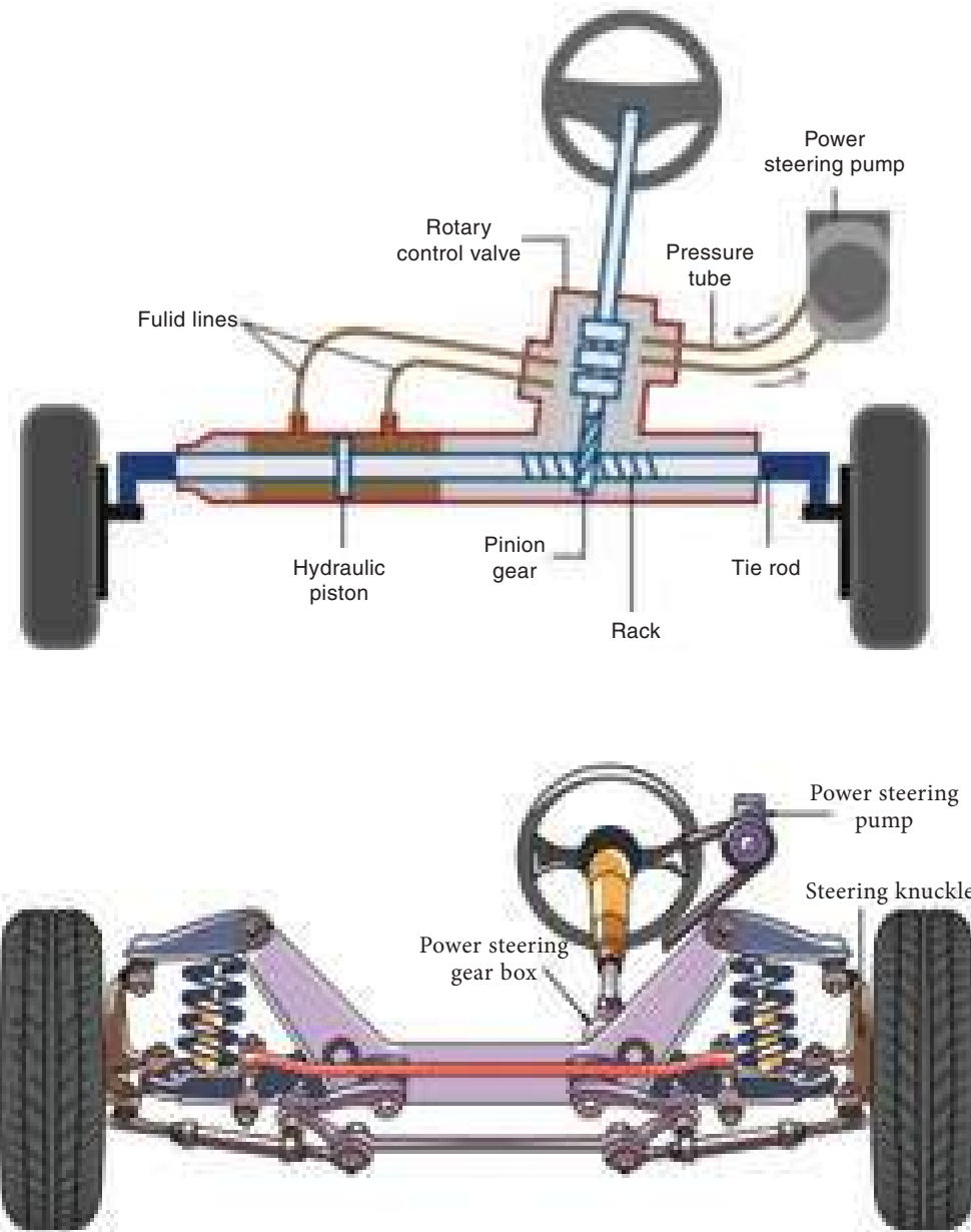
Figure 8.4 Power steering
