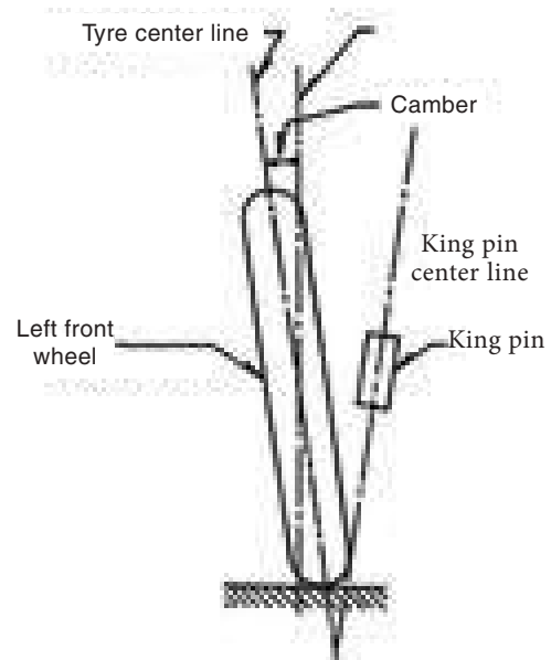
Figure 8.9.2.2 (b) Camber angle
