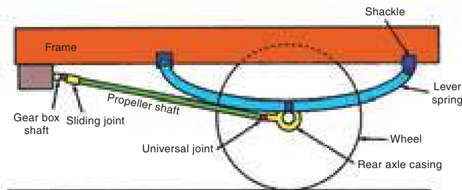
Figure 4.3.1 Hotchkiss drive
