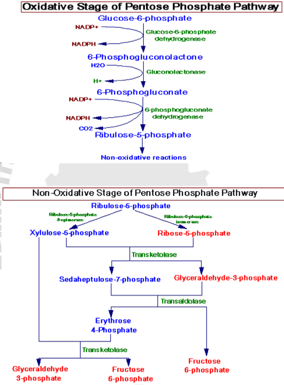
Fig 2.11 Oxidative and non –oxidative phases of HMP shunt
