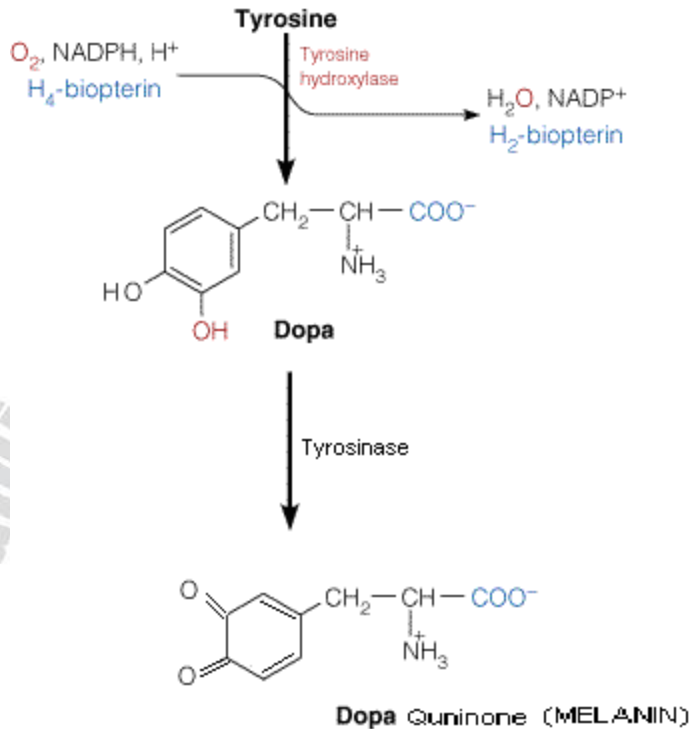
Fig 5.33 : Melanin Biosynthesis
