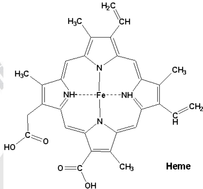
Fig 5.21: Structure of the heme prosthetic group (protophyrin IX) ring system.
