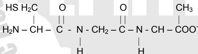
Fig 5.8: A tripeptide
