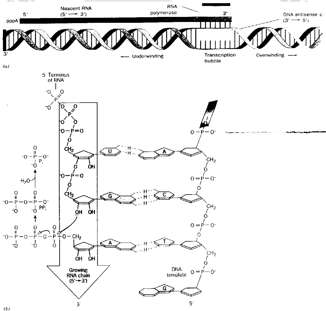
Fig 8.15 Transcription
