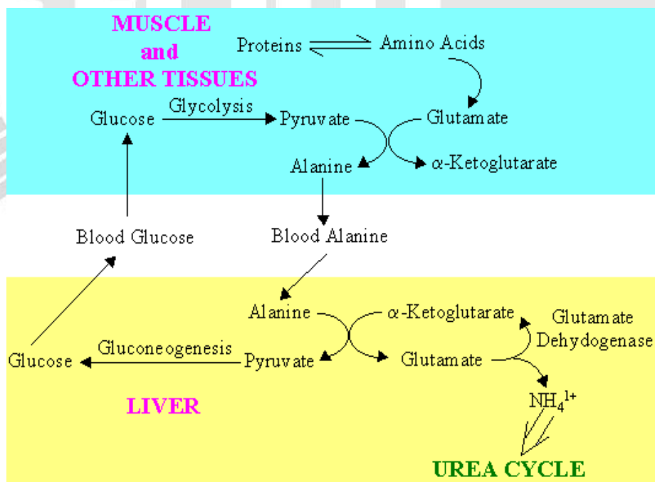
Fig 5.27: Glucose-Alanine Cycle
