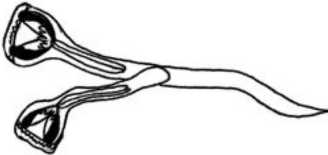
Mammonogamus laryngeus ( Syngamus trachea )
