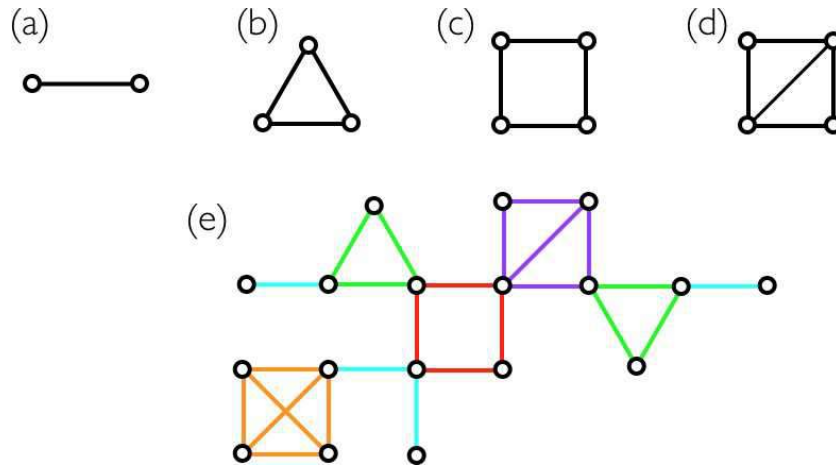
Figure 6.9: Connected versus irreducible clusters. Clusters (a) through (d) are irreducible in that they remain connected if any component site and its connecting links are removed. Cluster (e) is connected, but is reducible . Its integral c_\gamma may be reduced to a product over its irreducible components, each shown in a unique color.
