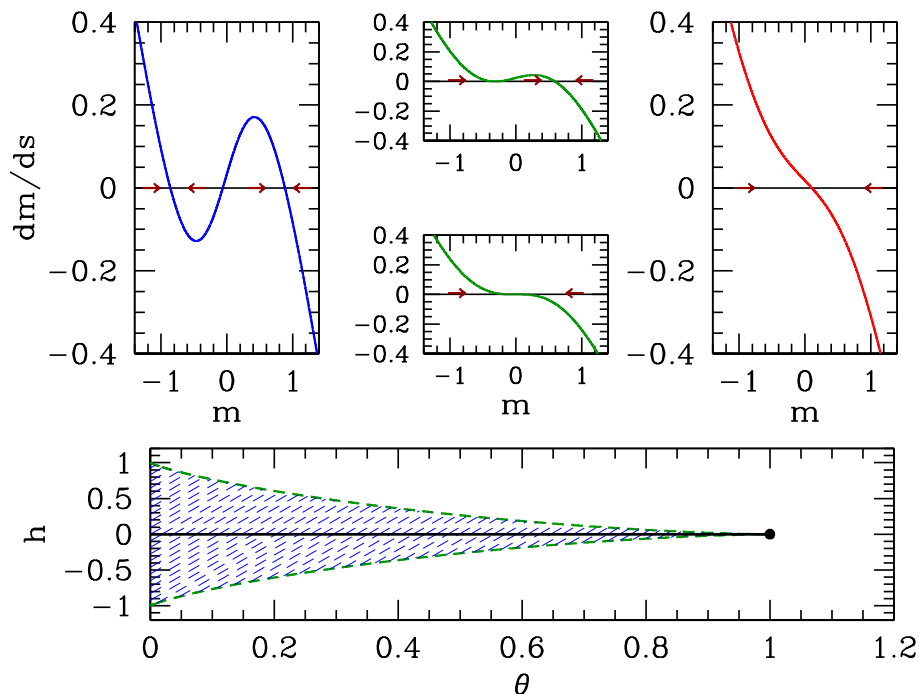
Figure 7.11: Dissipative magnetization dynamics \dot{m} = -f'(m) . Bottom panel shows h^*(\theta) from eqn. 7.65. For (\theta, h) within the blue shaded region, the free energy f(m) has a global minimum plus a local minimum and a local maximum. Otherwise f(m) has only a single global minimum. Top panels show an imperfect bifurcation in the magnetization dynamics at h = 0.0215 , for which \theta^* = 0.90 . Temperatures shown: \theta = 0.65 (blue), \theta = \theta^*(h) = 0.90 (green), and \theta = 1.2 . The rightmost stable fixed point corresponds to the global minimum of the free energy. The bottom of the middle two upper panels shows h = 0 , where both of the attractive fixed points and the repulsive fixed point coalesce into a single attractive fixed point (supercritical pitchfork bifurcation).
