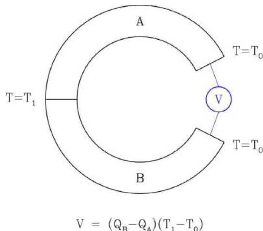
Figure 8.7: A thermocouple is a junction formed of two dissimilar metals. With no electrical current passing, an electric field is generated in the presence of a temperature gradient, resulting in a voltage V = V_A - V_B .
