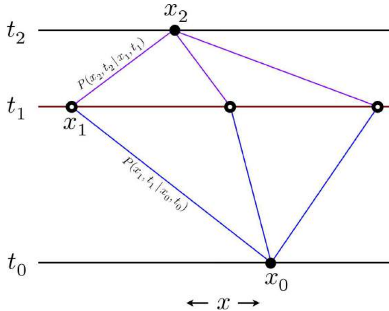
Figure 8.9: Interpretive sketch of the mathematics behind the Chapman-Kolmogorov equation.
