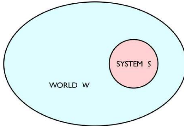
Figure 4.2: A system S in contact with a ‘world’ W . The union of the two, universe U = W \cup S , is said to be the ‘universe’.
