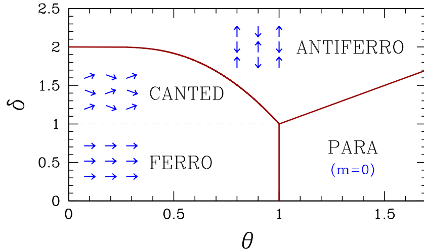
Figure 7.27: Mean field phase diagram for the model of eqn. 7.338 for the case \kappa = 1 .
