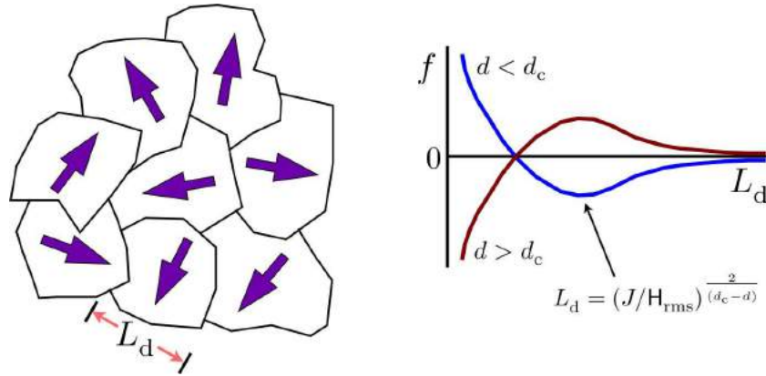
Figure 7.23: Left panel : Imry-Ma domains for an O(2) model. The arrows point in the direction of the local order parameter field \langle \hat{\mathbf{Q}}(\mathbf{r}) \rangle . Right panel : free energy density as a function of domain size L_d . Keep in mind that the minimum possible value for L_d is the lattice spacing a .
