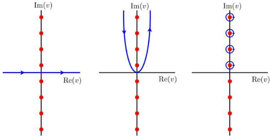
Figure 5.14: Deformation of the complex integration contour in eqn. 5.207.
