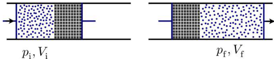
Figure 2.22: In a throttle, a gas is pushed through a porous plug separating regions of different pressure. The change in energy is the work done, hence enthalpy is conserved during the throttling process.
