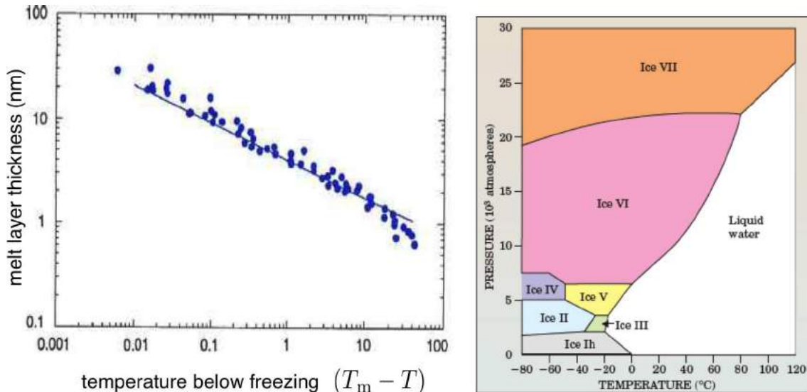
Figure 2.30: Left panel: data from R. R. Gilpin, J. Colloid Interface Sci. 77 , 435 (1980) showing measured thickness of the surface melt on ice at temperatures below 0^\circ\text{C} . The straight line has slope -\frac{1}{3} , as predicted by theory. Right panel: phase diagram of \text{H}_2\text{O} , showing various high pressure solid phases. (Source : Physics Today , December 2005).
