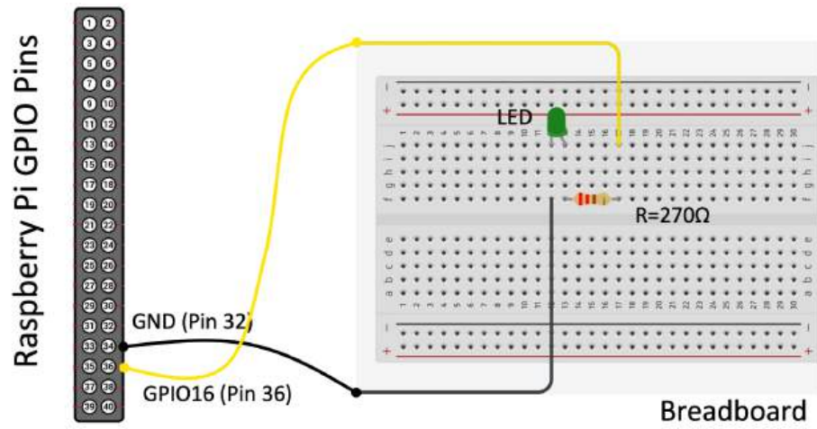
Figure 1.9: LED wiring
