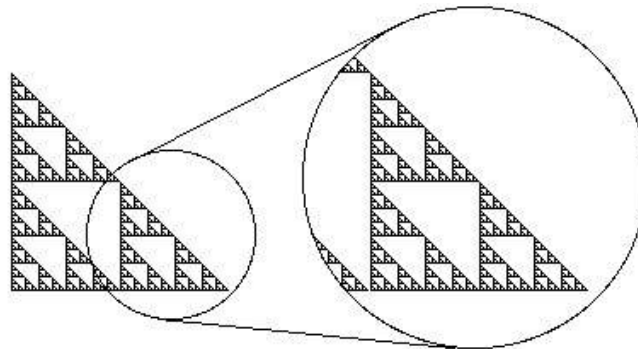
Figure 4.3: Sierpinski Triangle
