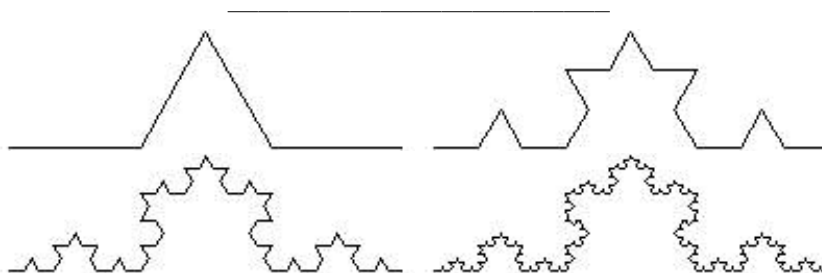
Figure 4.15: Approximations to the Koch Curve
