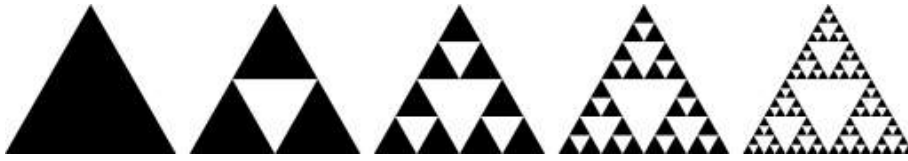
Figure 4.16: Approximations to the Sierpinski Triangle
