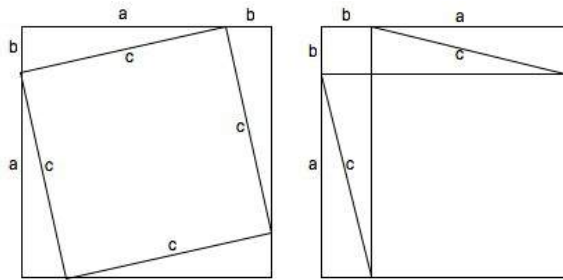
Figure 5.4: Another proof of Pythagoras's Theorem.
