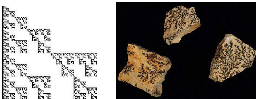
Figure 4.4: Some Dendrites
