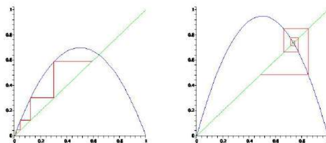
Figure 4.39: Cobwebs for f(x) = cx(1-x) with c = 2.8, 3.8 respectively. The first cobweb spirals away from the unstable fixed point 0. To see what happens to it, look at the similar example 2 in Figure 4.35. The second cobweb spirals away from the unstable fixed point a = 1 - 1/3.8 = 14/19 . To see what happens to it, look at example 2 in Figure 4.36.
