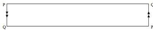
Figure 5.27: Mobius band identification diagram.
