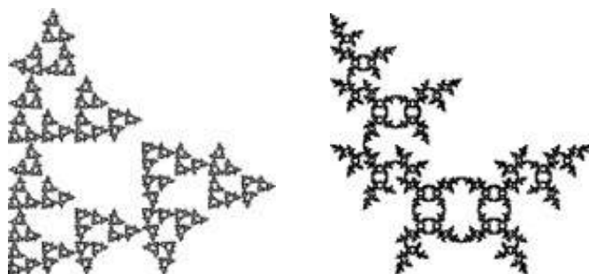
Figure 4.5: More Fractals
