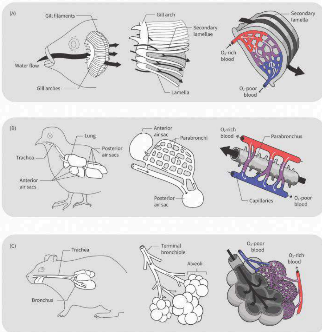
Comparison of gas exchange in fish gills, bird parabronchi, and mammalian lung (A) The gills of teleost fish consists of gill arches that support gill filaments. Gill filaments have a number of gill lamellae that deliver water to the capillary network in the gill arches. Blood flow through the capillaries of the secondary lamella is arranged in a counter-current pattern relative to the flow of the water through the gills. (B) In birds, a series of flexible air sacs work together with the lung. Within the lung, there are parallel small tubes called the parabronchi. Blood flow through the air capillaries is arranged in a cross-current pattern relative to the air flow across the parabronchi. (C) Air enters the mammalian lung via the mouth and nares, and then enters the trachea. The trachea branches into primary bronchi, which branches into successively smaller tubes. The bronchioles, the smallest tubes, terminate in sacs called alveoli where gas exchange occurs.
