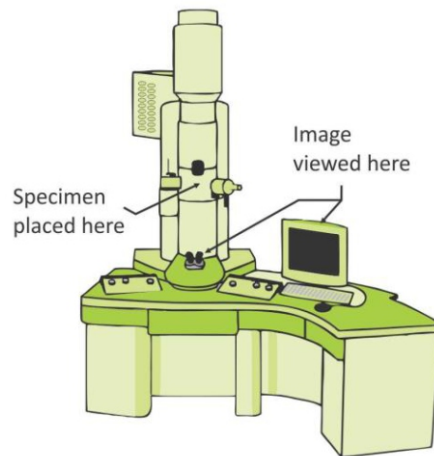
Figure 3.3: Electron microscope
