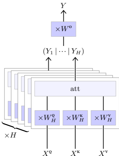
Figure 4.12: The Multi-head Attention layer applies for each of its h = 1, \dots, H heads a parametrized linear transformation to individual elements of the input sequences X^Q, X^K, X^V to get sequences Q, K, V that are processed by the attention operator to compute Y_h . These H sequences are concatenated along features, and individual elements are passed through one last linear operator to get the final result sequence Y .
