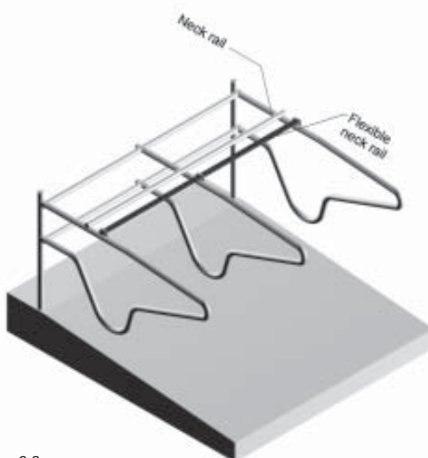
Figure 9.3. Flexible neck rail.
