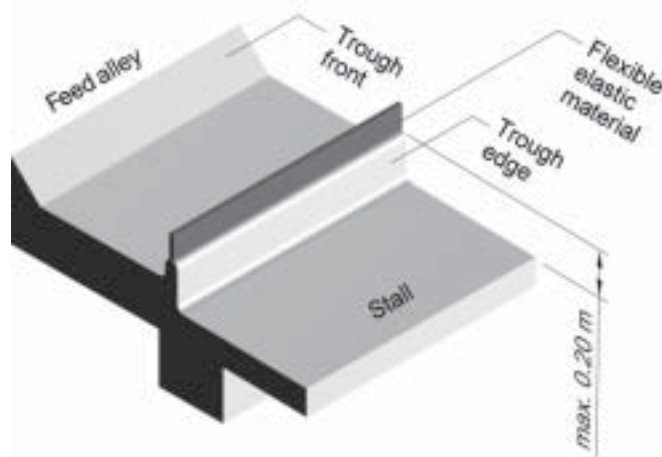
Figure 9.26 Trough design (principle construc- tion in tied-up housing system).
