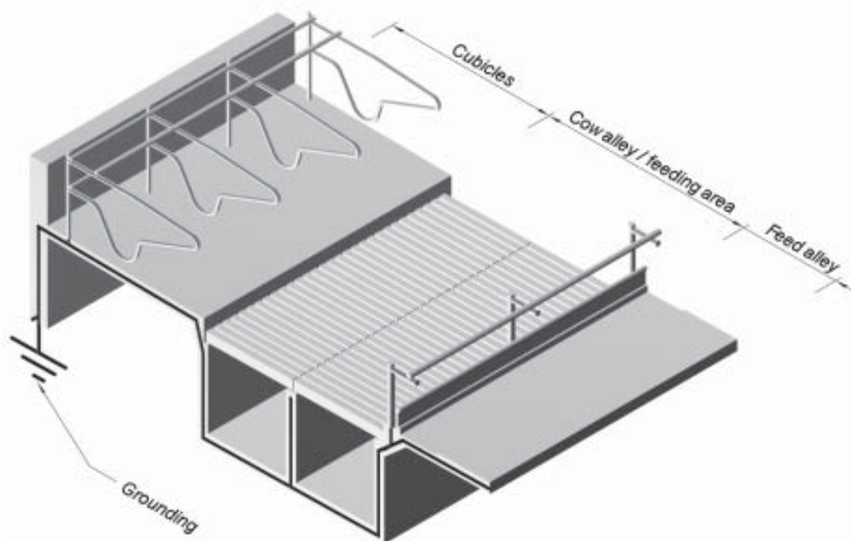
Figure 6.5. Example of equipotential bonding in cubicle housing system.
