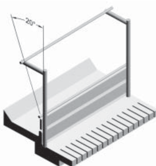
Figure 9.12. Design of feeding rack with neck rail.
