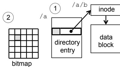
Figure 6.9: File, directory, bitmap
