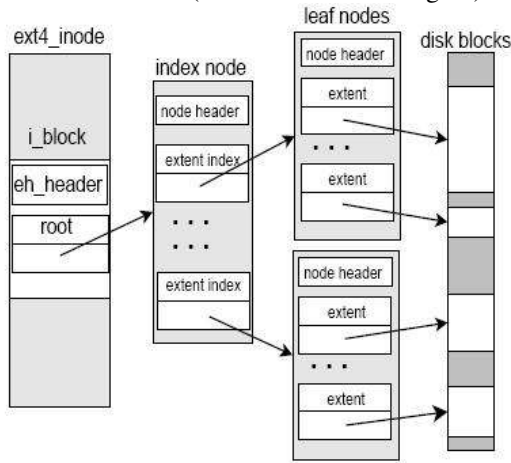
Figure 6.7: Ext4 on-disk structure
