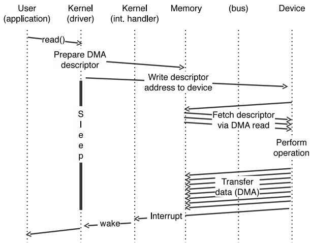
Figure 5.8: Driver Architecture
