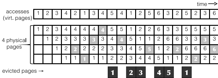
Figure 4.22: FIFO cleaning
