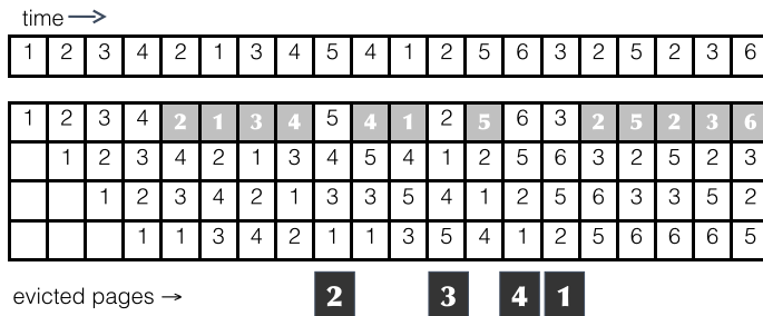
Figure 4.23: LRU cleaning
