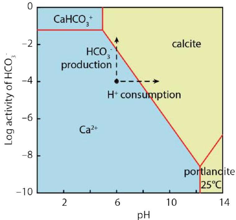
Figure 12.3 Variation in calcium speciation with bicarbonate activity and pH. Calcium is thermodynamically favored to exist as dissolved ions in the regions shaded blue and within minerals in the regions shaded yellow. The scatter point and dashed lines illustrate how bicarbonate production and hydrogen ion consumption by microbial reactions can cause calcite to become supersaturated in a solution with a temperature of 25°C. At the scatter point, the solution has a pH of 6 and contains -2 and -4 log activities of calcium and bicarbonate, respectively. From there, microbial reactions can cause calcite to saturate by increasing pH to just under 7 or by increasing the log activity of bicarbonate to just under -2. Many microbial reactions can cause both changes, creating a diagonal reaction path to saturation. Further increases in bicarbonate activity and/or pH would work to progressively supersaturate calcite, increasing the likelihood of precipitation. This activity diagram was calculated with The Geochemist's Workbench software (Bethke, 2018). https://commons.wikimedia.org/wiki/File:Calcium_speciation.png
