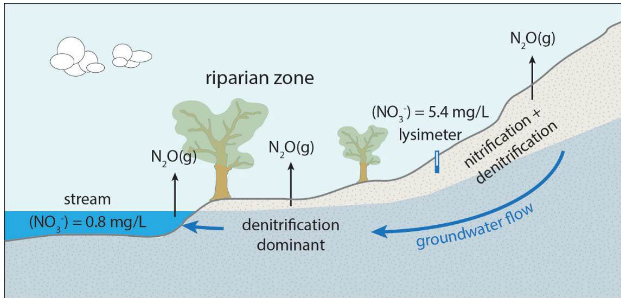
Figure 13.7 Schematic illustration of the distribution of nitrous oxide ( N_2O ) sources in one of the watersheds studied by Davidson and Swank (1986) and Davidson et al. (1986). Both nitrification and denitrification occurred in the soils at the study area, but nitrification was most important in well-drained upslope areas and denitrification was most important in poorly drained areas in the riparian zone, the interface between the terrestrial and aquatic ecosystems. Concentrations of nitrate measured in the stream and in soil water collected from a lysimeter are shown. The difference in nitrate concentrations between those sampling locations is consistent with nitrate removal by denitrification as subsurface water (groundwater and soil water) flows toward the stream. This figure is based on figure 5 of Davidson and Swank (1986). Image source: https://commons.wikimedia.org/wiki/File:Nitrous_oxide_sources.jpg
