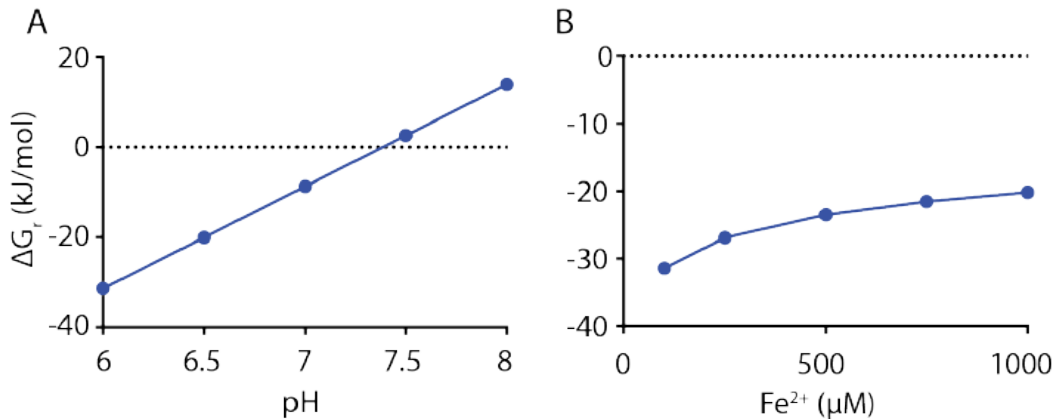
Figure 8.2 Variation in the Gibbs free energy yield of hematite reduction (reaction 11) in response to variation in (A) pH and (B) ferrous iron concentration. Note that (B) plots ferrous iron concentration but the free energy calculation was carried out with ferrous iron activities corresponding to those concentrations. https://commons.wikimedia.org/wiki/File:Energy_yield_of_iron_reduction.png
