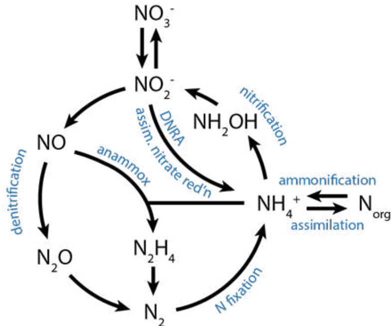
Figure 5.3 Microbial contributions to the nitrogen cycle. Figure after Fig. 1 of Jetten (2008). Microbial reactions are identified in blue font. N_{org} represents nitrogen in organic compounds.
