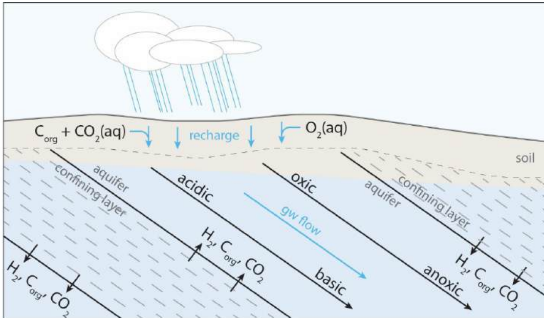
Figure 14.1 General trends in groundwater (gw) chemistry along flow. This simple conceptual model is based on trends observed in coastal plain aquifers in South Carolina, USA (Chapelle and Lovley, 1992; Lovley and Goodwin, 1988; McMahon and Chapelle, 1991; Park et al., 2009, 2006). According to the model, organic matter degradation is concentrated in the overlying soil and within fine-grained confining layers in the subsurface. These reactions help supply acid and potential electron donors to the groundwater by producing carbon dioxide ( \text{CO}_2(\text{aq}) ), dissolved organic compounds ( \text{C}_{\text{org}} ), and dihydrogen ( \text{H}_2 ). As the groundwater flows away from the recharge area, its pH evolves from acidic to basic because, within the aquifer, microbial reactions and mineral buffering reactions occur that consume hydrogen ions. The groundwater also tends to become increasingly anoxic, as aquifer aerobes deplete the groundwater's initial supply of oxygen and groups of anaerobes become active. https://commons.wikimedia.org/wiki/File:Evolution_of_groundwater_chemistry.jpg
