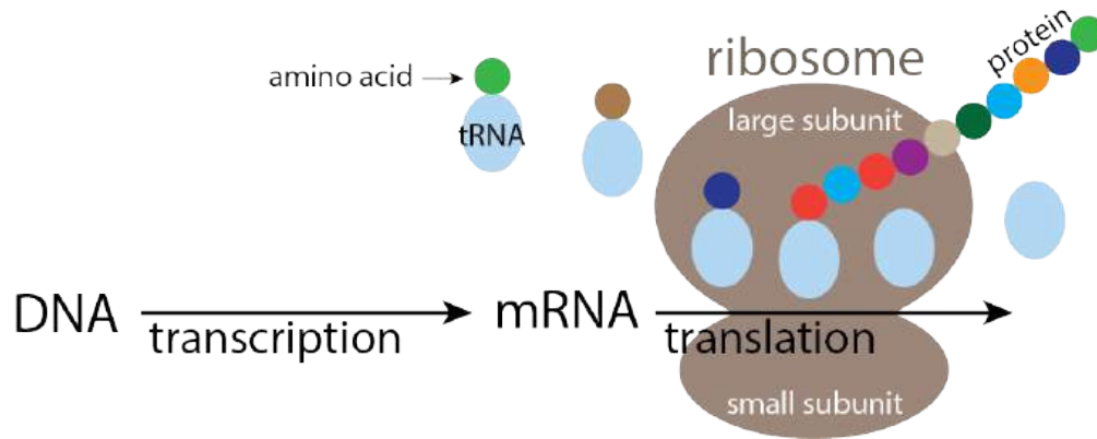
Figure 2.4 Overview of biological information flow. https://commons.wikimedia.org/wiki/File:Biological_information_flow.tif
