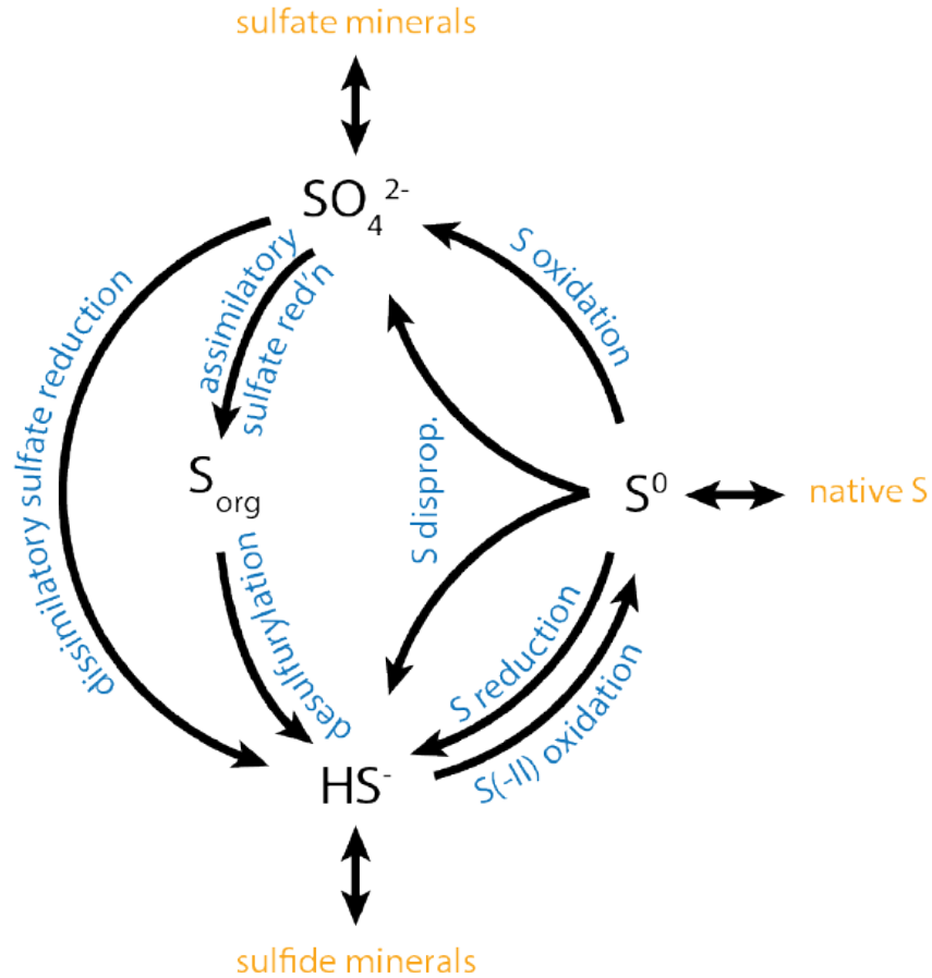
Figure 5.7 Microbial contributions to the global sulfur cycle. Microbial reactions are labeled in blue font and solid phases are in orange font. \text{S}_{\text{org}} represents sulfur in organic compounds. For simplicity, elemental sulfur ( \text{S}^0 ) represents one of several sulfur compounds with oxidation state between -2 and +6 that can form during sulfide oxidation. At least some of these intermediate sulfur species can be disproportionated into sulfate and sulfide. Figure based on figure 1 of Barton et al. (2014) and figure 2 of Muyzer and Stams (2008). https://commons.wikimedia.org/wiki/File:Microbial_sulfur_cycle.png
