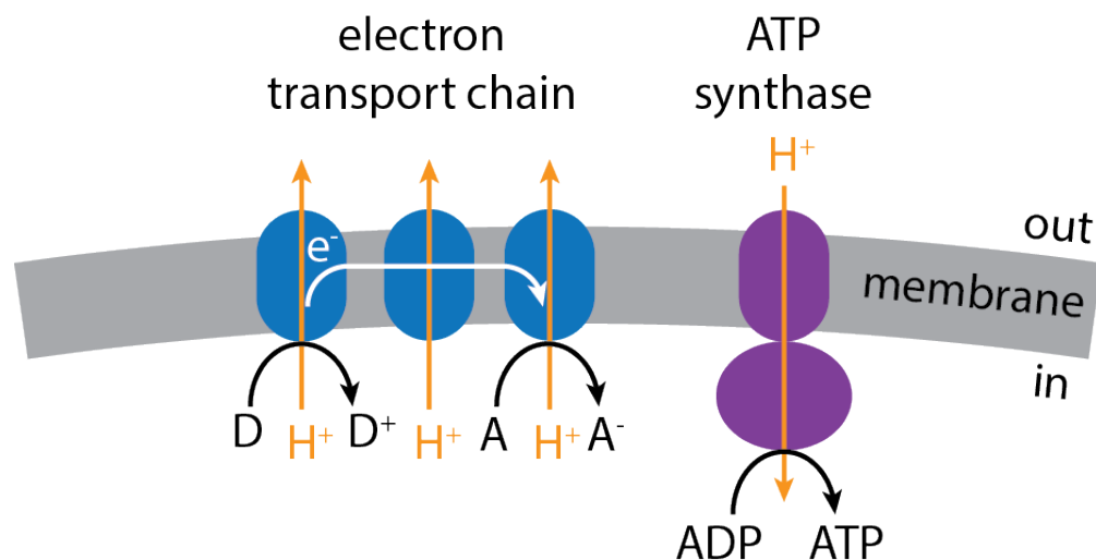
Figure 4.2 Generalized model of the electron transport chain. D and D^+ represent reduced and oxidized forms, respectively, of an electron donor or carrier, whereas A and A^- represent oxidized and reduced forms, respectively, of an electron acceptor. Electrons are transferred from the donor to the acceptor along three proteins. As the electrons move along the proteins, hydrogen ions are pumped outside of the membrane. Hydrogen ions move back to the interior at ATP synthase, allowing the enzyme to catalyze phosphorylation of ADP. Note that the make-up and configuration of the electron transport chain varies among metabolic groups. This figure is based on figure 1 of Jin and Bethke (2002).
