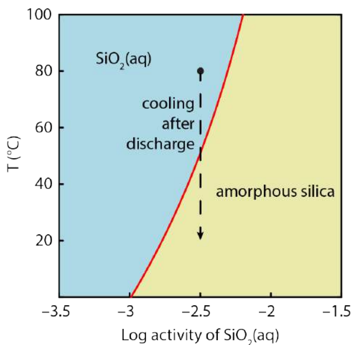
Figure 12.4. Variation in amorphous silica stability with temperature and dissolved silica activity. Amorphous silica is undersaturated in the region shaded blue and supersaturated in the region shaded yellow. The scatter point and dashed line illustrate how cooling of hot spring water with -2.5 log activity of dissolved silica ( \sim 200 mg L^{-1} ) can cause amorphous silica to become supersaturated. At the scatter point, the water has a temperature of 80^{\circ}C . From that point, cooling to about 55^{\circ}C causes amorphous silica to saturate. Further cooling causes amorphous silica to become increasingly supersaturated. In addition to cooling, other drivers of silica supersaturation in hot spring systems can include evaporation, changes in pH, and other factors (Guidry and Chafetz, 2002). This temperature-activity diagram was calculated with The Geochemist's Workbench software (Bethke, 2018). https://commons.wikimedia.org/wiki/File:Silica_speciation.png
