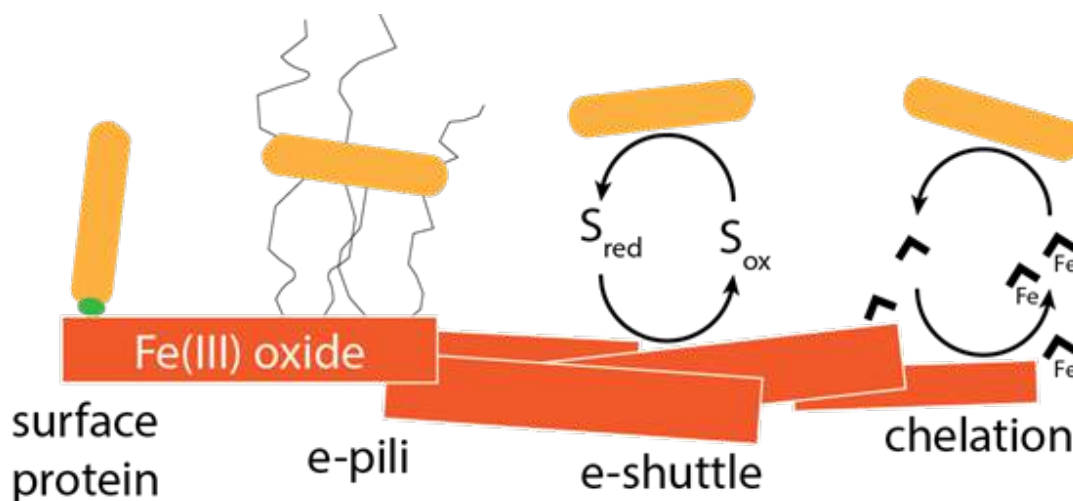
Figure 5.5 Potential strategies for extracellular electron transfer. The surface protein is represented by the green oval. S_{red} and S_{ox} represent reduced and oxidized electron shuttle compounds, respectively. Figure based on figure 1 of Galnick and Newman (2007) and figure 4 of Lovley and Holmes (2021).
