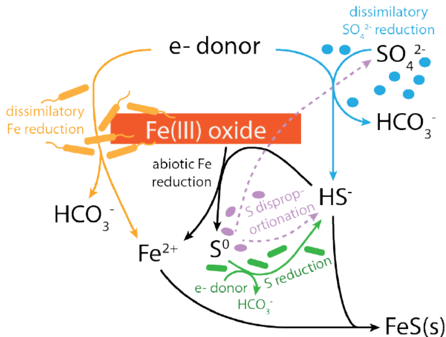
Figure 10.3 Conceptual model of potential interactions between iron reducers and microorganisms associated with the sulfur cycle. Elemental sulfur (S 0 ) represents one of several possible intermediate sulfur compounds, some of which can be disproportionated to sulfate and sulfide or used as an electron acceptor and reduced to sulfide.
