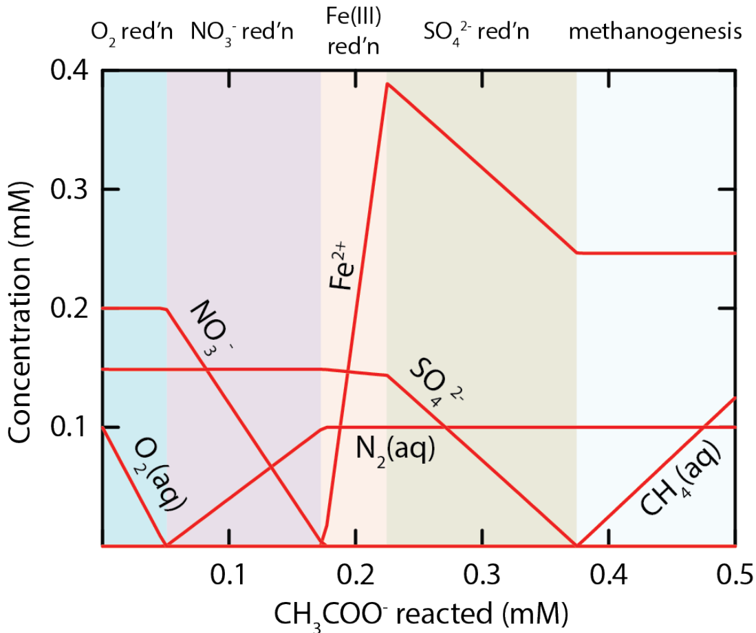
Figure 8.3 Redox zonation illustrated using reaction path modeling. The model simulates titration of a closed system with acetate. The system initially contains oxygen, nitrate, ferrihydrite ( \text{Fe}(\text{OH})_3 ), and sulfate as potential acceptors of electrons liberated by acetate oxidation. As acetate is added, electron acceptors are depleted in order of decreasing free energy yield.
