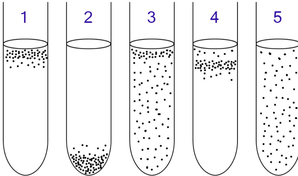
Figure 6.2 Schematic illustration of categories of microorganisms based on oxygen tolerance. The tubes show liquid cultures of microorganisms with a gradient from high dissolved oxygen concentration near the interface between gas and liquid to anoxic conditions at the bottom of the tube. Tube 1: Obligate aerobes concentrate near the interface between water and gas where dissolved oxygen concentration is highest. Tube 2: Obligate anaerobic microorganisms gather at the bottom to limit exposure to dissolved oxygen, but they are located throughout the tube. Tube 3: Facultative aerobes gather mostly at the top, where they can best take advantage of dissolved oxygen. Tube 4: Microaerophiles gather near the top of the tube but not at the interface. Tube 5: Aerotolerant anaerobes are not affected by oxygen and disperse throughout the tube.
