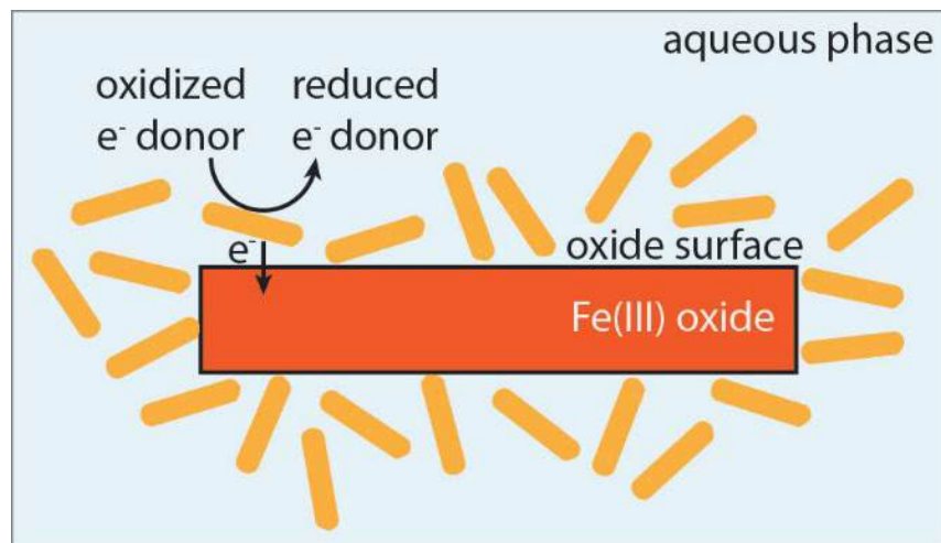
Figure 9.6 Schematic illustration of microbial reduction of crystalline ferric iron. The microorganisms exist within the aqueous phase and possibly attached to the surface of the oxide mineral. They can transfer the electrons to solid-phase ferric iron using a variety of strategies, as described in Chapter 5. Unless they cause the mineral to dissolve, the electrons must pass through the interface between the solid and aqueous phases. The size of that interface varies with the surface area of the oxide crystal. Thus, oxide surface area can influence the rate of the reaction.
