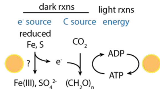
Figure 4.3 Summary of light and dark reactions (rxns) used by (A) oxygenic and (B) anoxygenic photoautotrophs. The question mark next to the sun in 4.3B indicates that only some anoxygenic phototrophs use oxygen in their dark reactions. Biomass is represented by the general formula for a carbohydrate ( (CH_2O)_n ). This figure is based on Figure 17.2 of Madigan et al. (2003). https://commons.wikimedia.org/wiki/File:Photoautotrophy.png
