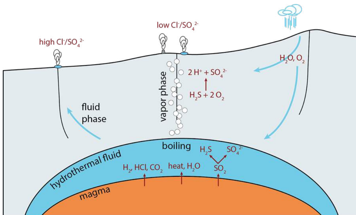
Figure 7.3 Conceptual diagram showing sources of water and solutes in a terrestrial hydrothermal system. The diagram depicts groundwater circulation driven by shallow magma at an extensional setting or hot spot. The heated water contains dissolved magmatic gas, including sulfur dioxide ( SO_2 ), which can disproportionate into sulfide and sulfate in high temperature aqueous solutions. As the solutions flow toward the surface along faults and joints, decompression boiling can liberate a gas phase enriched in sulfide. As the vapor approaches the surface, exposure to oxic groundwater can cause the sulfide to oxidize, producing sulfate and acid. Springs that primarily receive vapor phase inputs tend to be acidic with low concentration of chloride relative to sulfate. Springs that primarily receive fluid phase inputs tend to have near neutral to basic pH with high concentrations of chloride relative to sulfate. This figure and accompanying text are modified from figure 1 of Colman et al. (2019). https://commons.wikimedia.org/wiki/File:Hydrothermal_system.png
