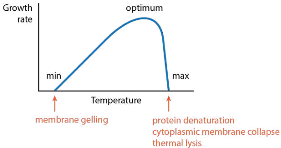
Figure 6.1 Influence of temperature on growth rate for an individual species. Figure based on 6.16 of Madigan et al. (2003). https://commons.wikimedia.org/wiki/File:Temperature_and_growth_rate.png
