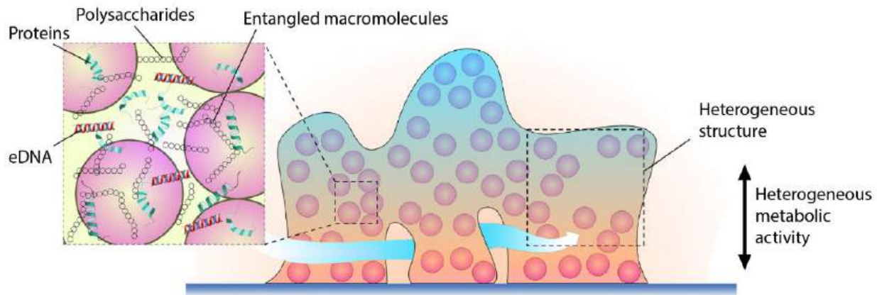
Figure 3.5 Heterogenous composition of microbial biofilm. Biofilms are composed of microorganisms encased within their extracellular polymeric substances (EPS). Compositional gradients in species composition and distribution occur alongside gradients in nutrient supply and redox conditions. Numerous components are found within the matrix, including polysaccharides, proteins, and environmental DNA (eDNA). Entanglement of these components helps provide cohesion. Image modified from Boudarel et al., (2018).
