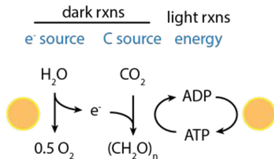
Figure 4.3 Summary of light and dark reactions (rxns) used by (A) oxygenic and (B) anoxygenic photoautotrophs. The question mark next to the sun in 4.3B indicates that only some anoxygenic phototrophs use oxygen in their dark reactions. Biomass is represented by the general formula for a carbohydrate ( (CH_2O)_n ). This figure is based on Figure 17.2 of Madigan et al. (2003). https://commons.wikimedia.org/wiki/File:Photoautotrophy.png
