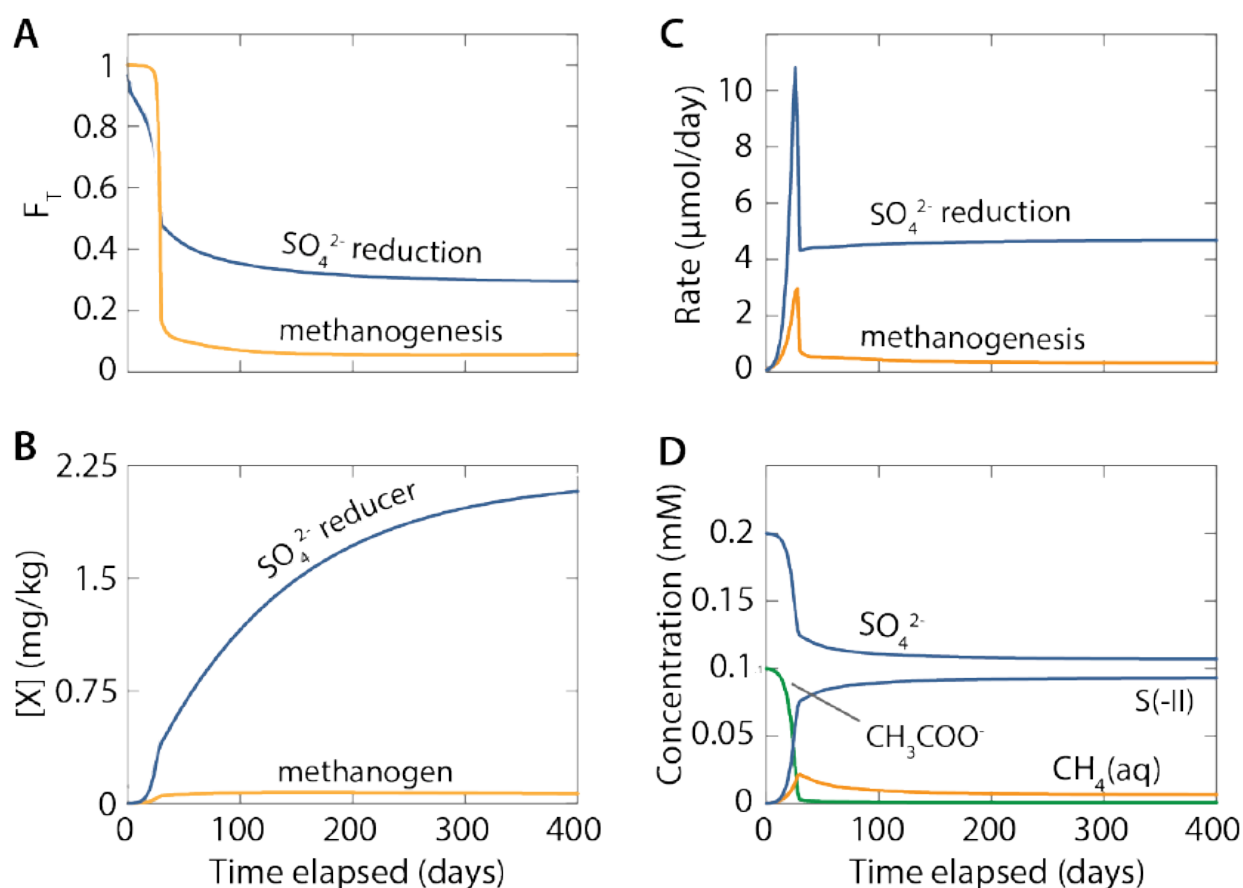
Figure 9.5. Results of a kinetic reaction path model of sulfate reduction and methanogenesis. Graphs show variation over time in (A) thermodynamic potential factors ( F_T ), (B) biomass abundances [X], (C) reaction rates, and (D) concentrations of sulfate ( \text{SO}_4^{2-} ), sulfide (S(-II)), acetate ( \text{CH}_3\text{COO}^- ), and methane ( \text{CH}_4 ). Reaction rates and population dynamics were simulated according to the Jin and Bethke rate law (2007, 2005, 2003, 2002) using kinetic parameters from Jin and Roden (2011). The model was calculated using the flush configuration in the React module of The Geochemist's Workbench. Additional details about the model are provided in the main text. https://commons.wikimedia.org/wiki/File:SRM_methanogen_model_results.png
