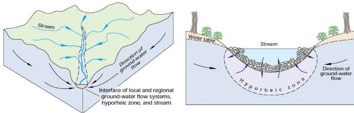
Figure 14.3 Schematic illustration of groundwater and surface waters coming together within streambeds from Winter et al. (Winter et al., 1998). Exchanges between surface water and groundwater are temporally and spatially variable and can be driven by stream meandering, abrupt changes in streambed slope, changes in the elevation of the water table, and variation in the height of water within the stream channel (i.e., stage). Image source: https://pubs.er.usgs.gov/publication/cir1139
