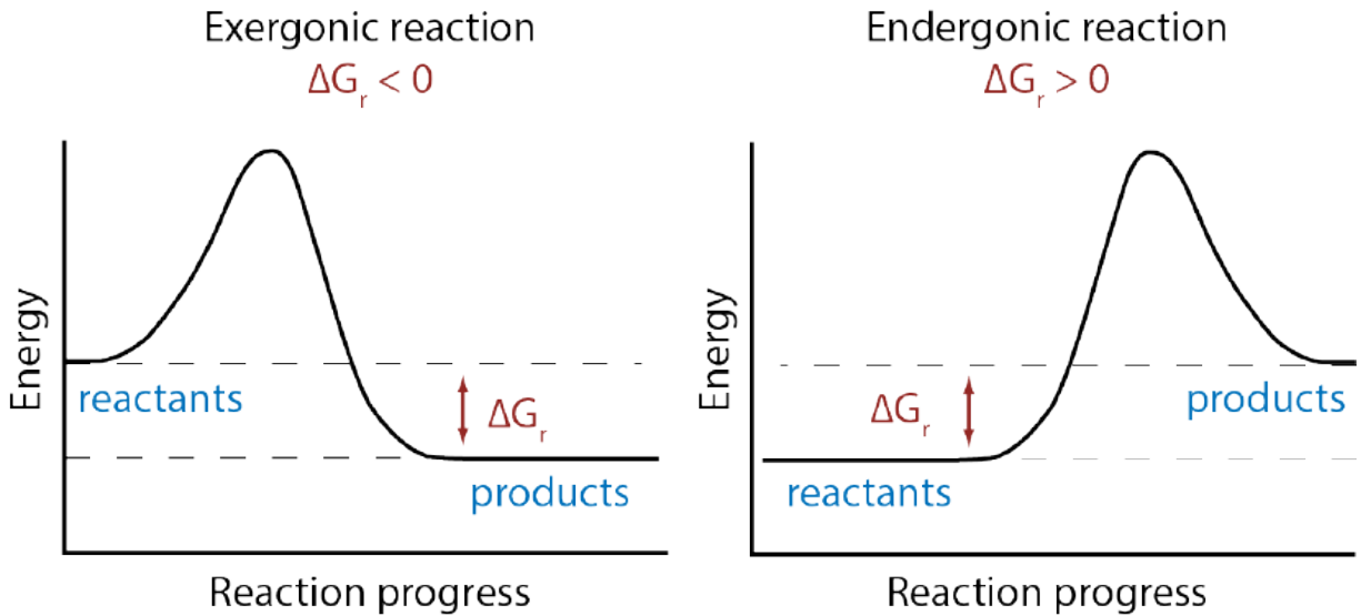
Figure 8.1 Variation in free energy during an exergonic and endergonic reaction according to transition-state theory. https://commons.wikimedia.org/wiki/File:Gibbs_free_energy_changes.png
