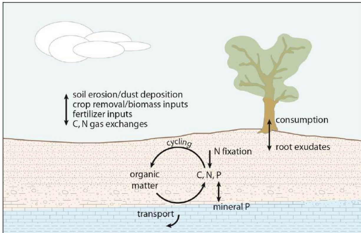
Figure 7.1 Simple conceptual diagram of the carbon, nitrogen, and phosphorus (C,N,P) budgets in the shallow terrestrial subsurface. Organisms recycle nutrients when they degrade organic matter and form new organic compounds. Nutrients can also be added externally or removed from the soil, as shown in the figure. The tree represents plants in general, not just woody vegetation. Root exudates from plants include sugars, amino acids, and organic acids (Canarini et al., 2019). Dust can serve as a major nutrient source for soil, particularly where nutrients have been depleted from the underlying bedrock by intense weathering (Aciego et al., 2017; Pett-Ridge, 2009). Fertilizer inputs include both chemical fertilizers as well as animal wastes. Subsurface transport represents leaching of nutrients and other compounds as water passes through soil. Mineral phosphorus represents primary and secondary phosphate minerals as well as phosphorus that is adsorbed to mineral surfaces.
