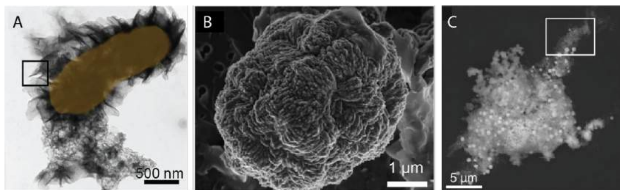
Figure 12.7 Examples of sulfide biominerals: (A) mackinawite encrusting a microbial cell, (B) pyrite spherule, and (C) pyrite spherules within a mackinawite aggregate. Minerals in (A) and (B) formed in cultures containing Desulfovibrio and Sulfurospirillum species from lake water. The minerals in (C) formed in cultures of Desulfovibrio desulfuricans . Boxes in (A) and (C) were used for purposes in the original publications and are not relevant here. Image sources: (A) and (B) Berg et al. (2020), (C) Duverger et al. (2020).
