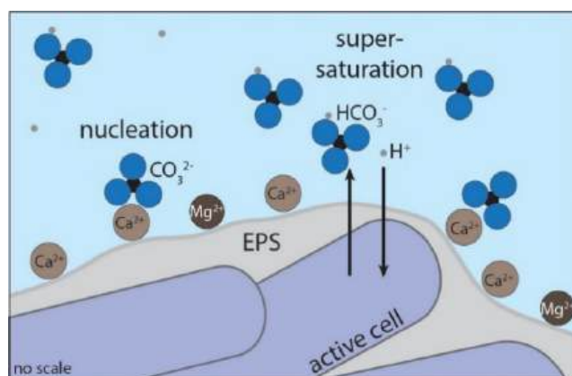
Figure 11.2 Schematic illustration of biomineralization mechanisms. Microorganisms can cause a mineral to form by changing the chemistry of a solution such that the mineral become supersaturated (see Box 11.1) and by forming biomass that provides nucleation surfaces. As an example, microorganisms can promote carbonate precipitation by producing bicarbonate and consuming hydrogen ions, which would help drive the minerals to supersaturation, and by producing biomass that complexes metals such as calcium and magnesium, which then serve as nucleation sites. That biomass can include extracellular polymeric substances (EPS), as depicted, as well as the cells themselves. Note that the figure is not to scale and that the relative size of ions is greatly exaggerated. https://commons.wikimedia.org/wiki/File:Biomineralization.jpg
