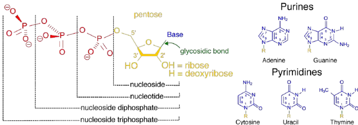
Figure 2.2 Chemical structure of nucleotides and nucleosides. Public domain. https://commons.wikimedia.org/wiki/File:Nucleotides.png
