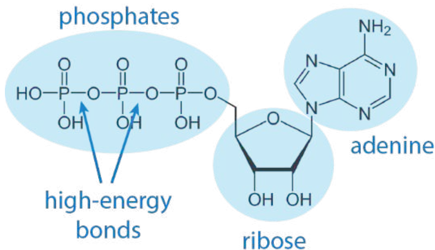
Figure 4.1 Adenosine triphosphate (ATP) molecule with regions highlighted to show adenine, ribose, phosphate molecules, and the high-energy bonds between phosphate molecules. ATP illustration source: https://commons.wikimedia.org/wiki/File:Adenosintriophosphat_protoniert.svg
