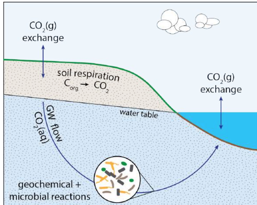
Figure 13.6 Schematic illustration of potential fates of carbon dioxide produced by organic matter oxidation ( C_{org} ) during soil respiration. Carbon dioxide produced by soil respiration can reach the atmosphere directly from the soil. It may also be transported by groundwater flow to adjacent surface water bodies, where it can then be emitted. Image: https://commons.wikimedia.org/wiki/File:Fates_of_soil_CO2.png
