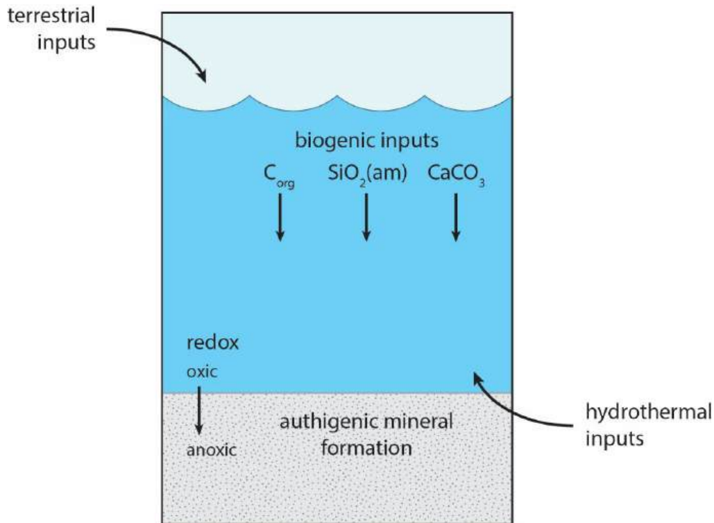
Figure 12.8 Schematic illustration of major inputs and reactions that guide marine sediment composition. Terrestrial sediment inputs include dust and river sediment. Hydrothermal inputs are fluids with reduced elements that can serve as energy sources for vent microbial communities. Redox zones develop in marine sediment as microorganisms couple oxidation of organic matter with available electron acceptors. Authigenic minerals form in response to those redox reactions and reactions between reactive sediment inputs, including organic matter ( C_{\text{org}} ), amorphous silica ( \text{SiO}_2(\text{am}) ), and calcium carbonate ( \text{CaCO}_3 ).
