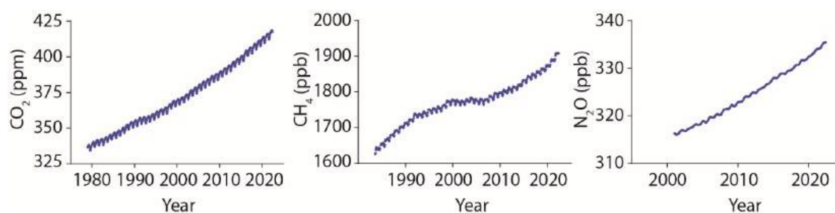
Figure 13.3 Variation with time in the abundance of carbon dioxide (CO 2 ), methane (CH 4 ), and nitrous oxide (N 2 O) in the atmosphere. Values are globally-averaged monthly means determined from marine surface sites. Units are mole fractions expressed as parts per million (ppm) for carbon dioxide and parts per billion (ppb) for methane and nitrous oxide. Note that x-axes differ in scale for each graph. Data plotted are available from the U.S. National Oceanic and Atmospheric Administration ( https://gml.noaa.gov/ccgg/ ). Image: https://commons.wikimedia.org/wiki/File:Greenhouse_gas_trends.jpg
