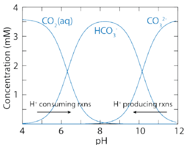
Figure 13.5 Variation with pH in the proportions of dissolved inorganic carbon species. Reactions that consume hydrogen ions lower hydrogen ion activity and thus increase pH. As such, they work to transform dissolved carbon dioxide ( \text{CO}_2(\text{aq}) ) into bicarbonate ( \text{HCO}_3^- ) and carbonate ( \text{CO}_3^{2-} ). Reactions that produce hydrogen ions do the opposite. Species distributions shown in this figure were calculated using the React module of The Geochemist's Workbench software for a solution with an ionic strength of 20 mmolal and an initial carbon dioxide gas fugacity of 0.1.
