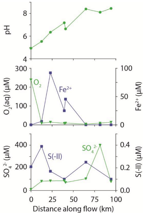
Figure 14.2 Variation along flow in groundwater pH and concentrations of oxygen ( O_2 ), ferrous iron ( Fe^{2+} ), sulfate ( SO_4^{2-} ), and sulfide ( S(-II) ) in the Middendorf aquifer as measured by Park et al. (2006). Concentrations were below their detection limit for ferrous iron ( 0.2 \mu M ) and sulfide ( 0.1 \mu M ) for three and two samples, respectively. For those samples, detection limit concentrations are plotted. In addition, sulfide concentration was not determined for two samples, for which no scatter points are shown.
