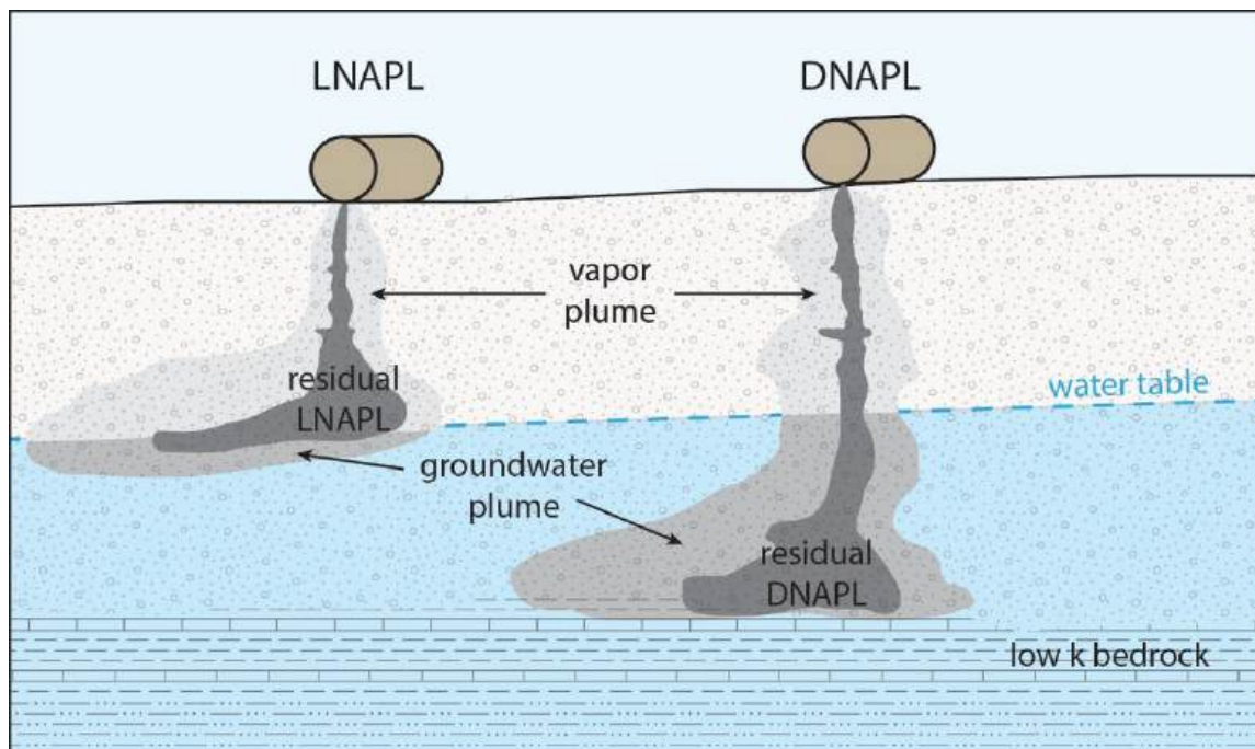
Figure 14.9 Schematic illustration of the spreading of light non-aqueous phase liquid (LNAPL) and dense non-aqueous phase liquid (DNAPL) in the subsurface. LNAPLs are less dense than water and thus can accumulate at the water table. In contrast, DNAPLs are denser than water and thus can sink below the water table until they encounter a low permeability ( k ) surface. Both LNAPLs and DNAPLs volatilize and dissolve, creating vapor and groundwater plumes, respectively.
