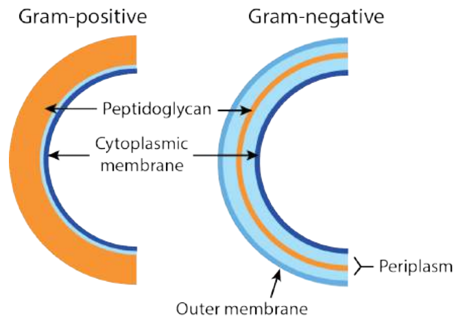
Figure 3.3 Schematic illustration of the structure of Gram-positive and Gram-negative bacterial cell walls. https://commons.wikimedia.org/wiki/File:Bacterial_cell_walls.jpg
