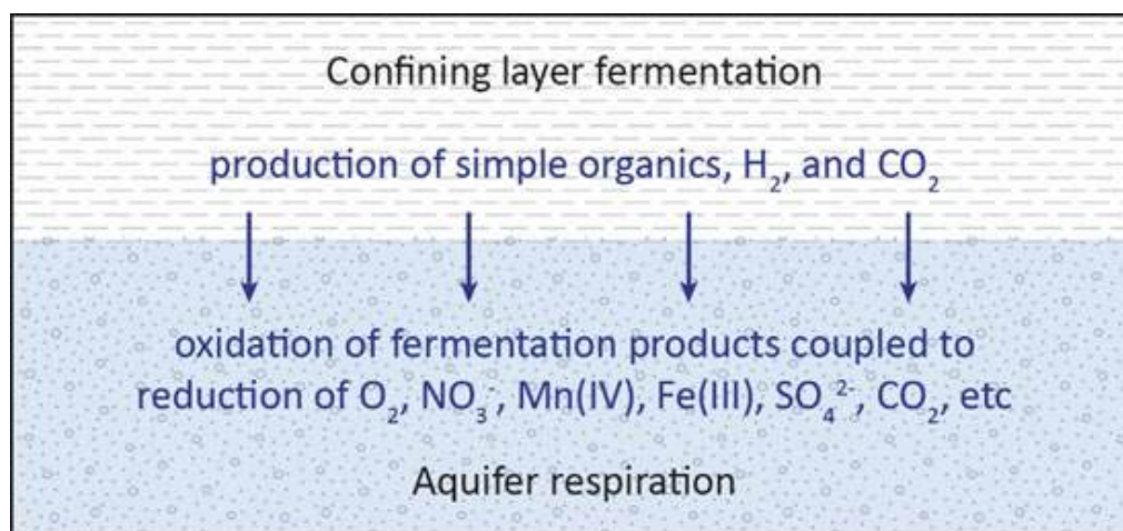
Figure 7.2 Conceptual diagram illustrating microbial respiration in aquifers fueled by fermentation of organic matter in fine-grained organic-rich confining layers. https://commons.wikimedia.org/wiki/File:Aquifer_microbiology.jpg
