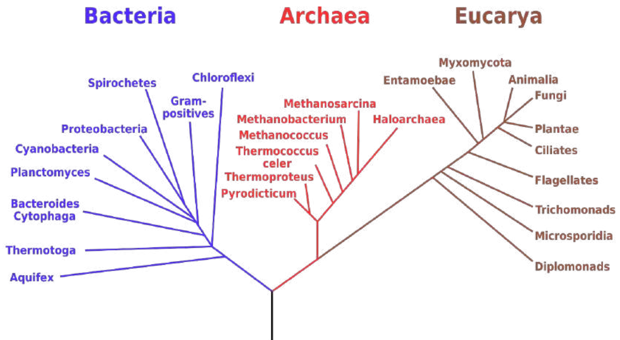
Figure 2.1 Phylogenetic tree based on the 16S ribosomal RNA (rRNA) gene. The tree shows the three domains of life (Bacteria, Archaea, and Eukarya or Eucarya) and approximate evolutionary distances between them. Groups of organisms listed are not uniform in taxonomic level. Image credit: Eric Gaba. Public domain.
