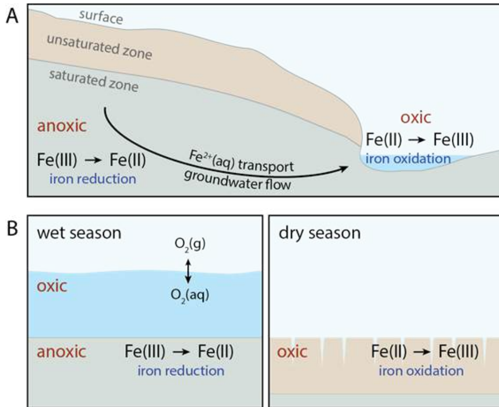
Figure 6.3 Schematics showing examples of ways (A) transport and (B) environmental change can serve as environmental controls on microbial populations involved in iron cycling. Part (A) depicts microbial reduction of ferric iron ( \text{Fe(III)} ) within an anoxic zone of an aquifer. The ferrous iron ( \text{Fe(II)} ) produced by iron reduction is relatively soluble. As such, some of it can be transported by groundwater flow to a discharge zone at the surface, where oxygen is available and iron oxidation can occur. The iron oxides shown in Figure 5.6 appear to have formed because of this very situation. Part (B) depicts the impact of seasonal variation in precipitation as a control on the water saturation and redox state of a wetland soil. During the wet season, water limits the oxygen supply at depth, allowing microbes to use ferric iron minerals as electron acceptors in the soil. During the dry season, the soil dries, exposing formerly anoxic portions of the soil to oxygen. As a result, ferrous iron ( \text{Fe(II)} ) produced in the wet season can then be oxidized. https://commons.wikimedia.org/wiki/File:Biogeochemical_cycle_turn_over.jpg
