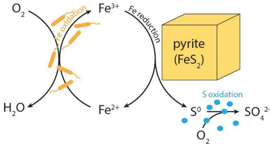
Figure 14.8 Schematic illustration pyrite weathering under acidic conditions (e.g., below pH 4.5) by iron- and sulfur-oxidizing microorganisms. Elemental sulfur (S 0 ) represents one of multiple intermediate sulfur species that can be produced by sulfide oxidation. In addition to oxygen (O 2 ), iron-oxidizing microorganisms can also couple ferrous iron oxidation to nitrate reduction. This figure is based on figure 3 of Newsome and Falagán (2021). Image source: https://commons.wikimedia.org/wiki/File:AMD_conceptual_model.jpg
