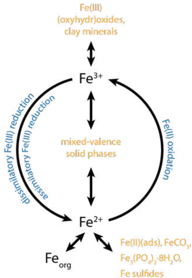
Figure 5.4. Microbial contributions to the global iron cycle. Microbial reactions are labeled in blue font and solid phases are in orange font. Fe_{org} represents iron in organic compounds, Fe(II)ads is adsorbed ferrous iron whereas FeCO_3 and Fe_3(PO_4)_2 \cdot 8H_2O are chemical formulas for siderite and vivianite, respectively. This figure is based on figure 1 of Schröder et al. (2003). https://commons.wikimedia.org/wiki/File:Microbial_iron_cycle.png
