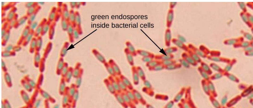
Figure 3.4 Image showing endospores within rod-shaped bacteria. https://commons.wikimedia.org/wiki/File:OSC_Microbio_02_04_Endospores.jpg
