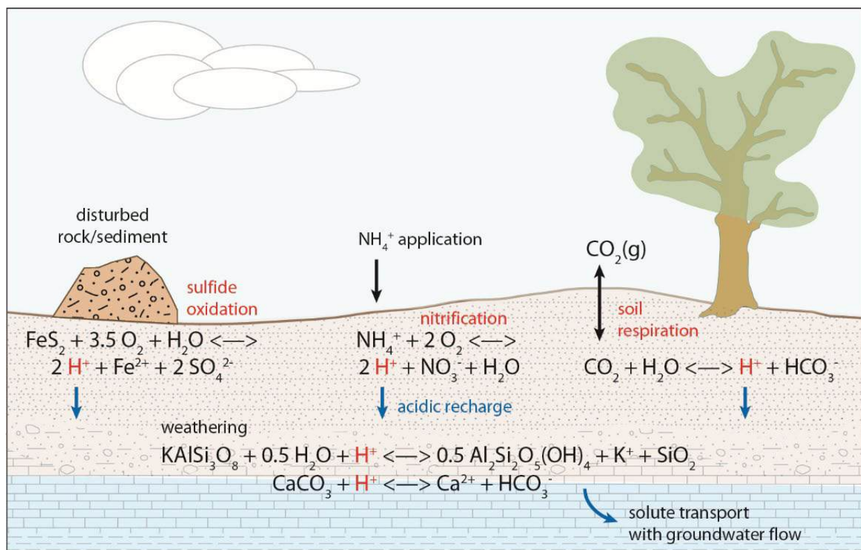
Figure 11.3 Conceptual diagram of weathering in the subsurface driven by acid production in an overlying soil. Some of the acid generated in soil may be neutralized by mineral weathering reactions in the soil and unsaturated zone. The acid that is not neutralized there may react with the aquifer matrix. Two example weathering reactions are shown, one in which potassium feldspar ( KAlSi_3O_8 ) reacts with acid to produce kaolinite ( Al_2Si_2O_5(OH)_4 ) and aqueous potassium and silica, and the other in which calcium carbonate ( CaCO_3 ) reacts with acid to produce aqueous calcium and bicarbonate. Solutes generated by these reactions can be transported by groundwater flow to nearby surface water bodies or into the deep subsurface.
