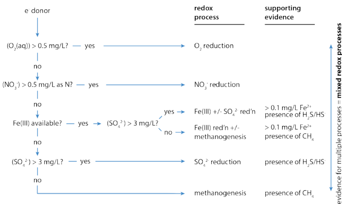
Figure 8.4 Flowchart for evaluating the dominant redox process in an aqueous system using water chemistry data. As described in the text, this framework is modified from that presented in McMahon and Chapelle (2008). https://commons.wikimedia.org/wiki/File:Redox_framework.png
