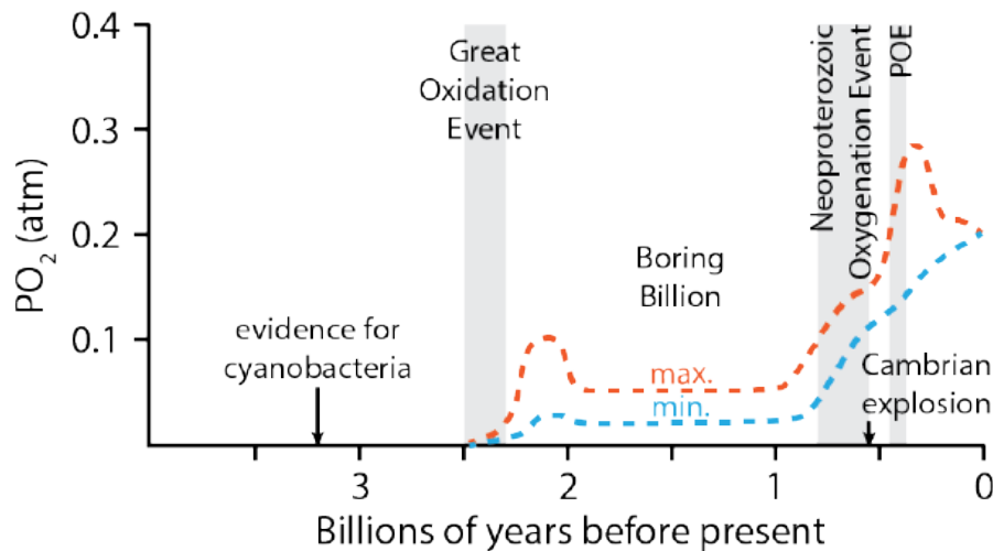
Figure 13.1 Estimated variation in the partial pressure of oxygen in the atmosphere over the past four billion years. Oxygen levels are reproduced from Bekker and Holland (2012). Research by Satkoski et al. (2015) indicates cyanobacteria were active by at least 3.2 billion years ago. The Great Oxidation Event is shown in the figure to have occurred from 2.5 to 2.3 billion years, although the literature varies on the specific time range. POE refers to the Paleozoic Oxygenation Event. A recent reconstruction by Mills et al. (2023) provides a more detailed look at variation in atmospheric oxygen levels during the Phanerozoic. https://commons.wikimedia.org/wiki/File:Oxygen_vs_time.png
