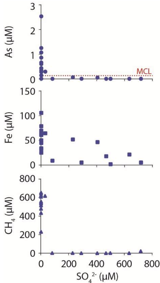
Figure 14.6 Variation with sulfate concentration in total dissolved arsenic, iron, and methane concentrations in the Mahomet aquifer. Data plotted are from Kirk et al. (2004). Given the pH of the groundwater samples, dissolved iron is expected to be nearly entirely composed of ferrous iron because ferric iron has low solubility at near neutral pH. The plot with arsenic includes a dotted red horizontal line corresponding to the US EPA maximum contaminant level (MCL) for public drinking water supplies ( 10 \mu\text{g}/\text{L} = 0.133 \mu\text{M} ). For samples with concentrations below the detection limits of the methods used for the study, detection limit values are plotted. https://commons.wikimedia.org/wiki/File:Mahomet_aquifer_geochemistry_results.jpg
