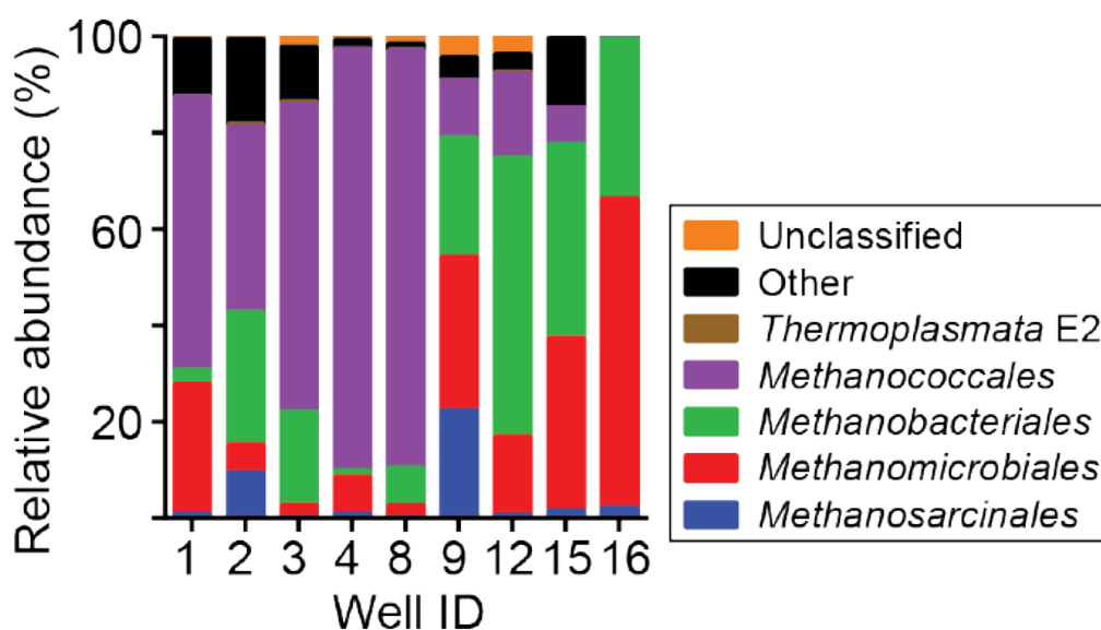
Figure 2.5 Results of 16S rRNA gene analysis by Kirk et al. (2015). Results are only shown for sequences that classified within orders of Archaea, and only classes with average relative abundance greater than 2% are specifically identified.
