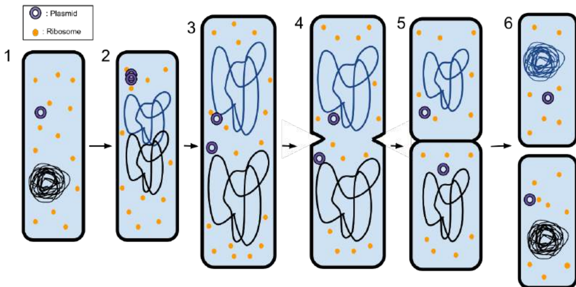
Figure 3.7 Binary fission in a bacterial or archaeal cell. (1) The initial cell contains tightly coiled DNA. (2) The cell's DNA is replicated and then (3) pulled into separate ends of the elongating cell. (4) A new cell wall starts to grow and then (5) fully develops, allowing the cells to separate (6). Image source: https://en.wikipedia.org/wiki/Fission_(biology)
