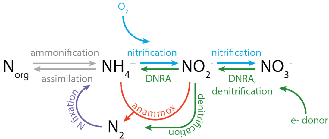
Figure 10.2 Conceptual model of potential interactions among nitrogen cycling microorganisms. This figure is based on figure 5 of Kuenen (2020) and represents a linear version of the nitrogen cycle figure in Chapter 5 (Fig. 5.3). https://commons.wikimedia.org/wiki/File:N_cyclers_and_anammox.png
