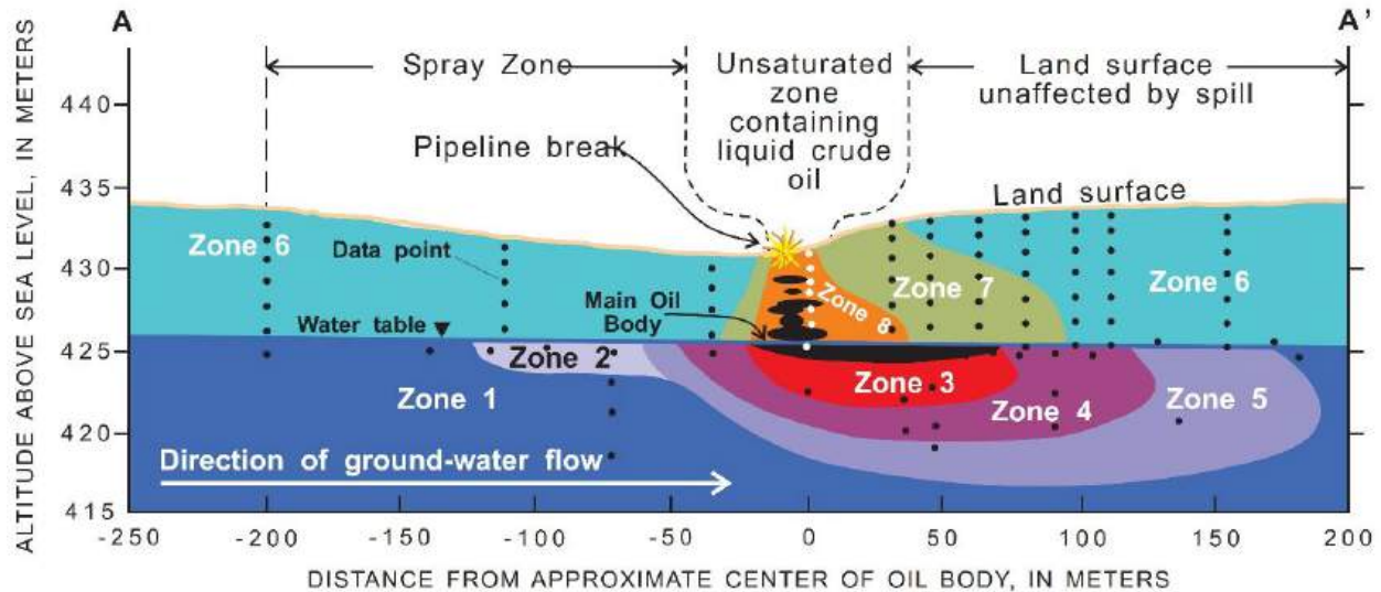
Figure 14.12 Subsurface geochemical zones identified in groundwater and the unsaturated zone at the Bemidji north oil pool site. This figure was taken from USGS Fact Sheet 084-98 (Delin et al., 1998).
