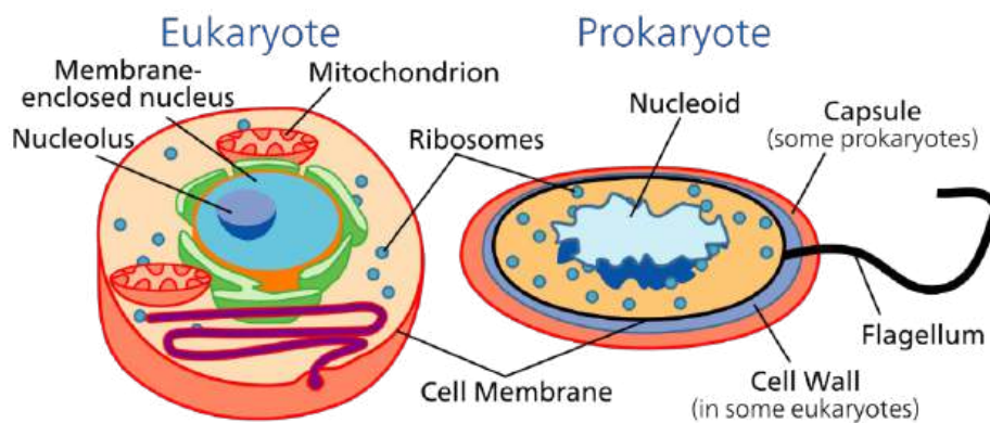
Figure 3.1 Comparison of eukaryotic and prokaryotic (bacterial and archaeal) cells. Figure is not to scale. Image is public domain. Source: https://en.wikipedia.org/wiki/Cell_(biology)
