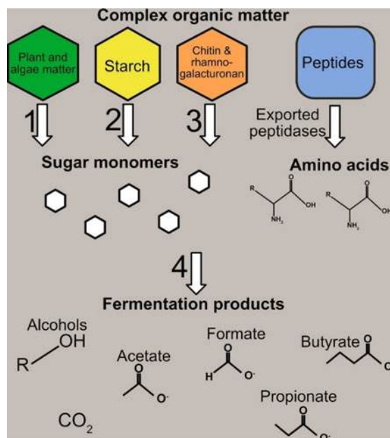
Figure 5.2 Illustration of organic matter degradation pathways investigated by Zinke et al. (2019) in Baltic Sea sediment. Complex polysaccharides are broken down into sugar and amino acid monomers, which can then be fermented into relatively simple organics (alcohols, acetate, formate, propionate, butyrate), H 2 , and CO 2 .
