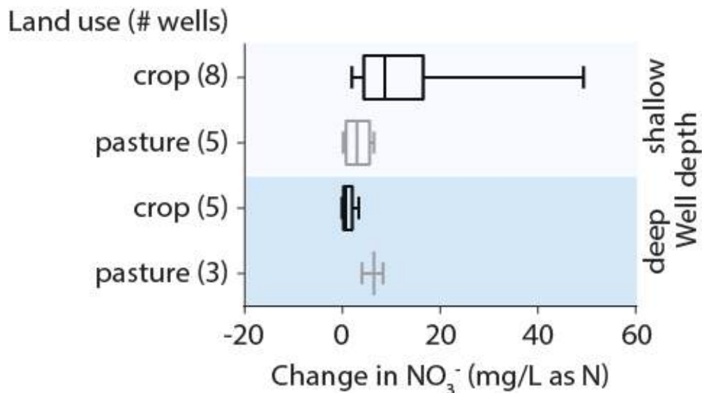
Figure 14.5 Box plot showing changes in nitrate concentration between the 1970s and 2016 based on data from Lane et al. (2020). Boxes show the quartiles and whiskers show the range of values. Shallow wells have an average depth of 22 m and are screened just below the water table in aquifer. Deep wells have an average depth of 41 m are screened near the aquifer base. Wells were sampled in areas used for crops and pastures, with the number of wells in each land use and depth category listed in parentheses.
