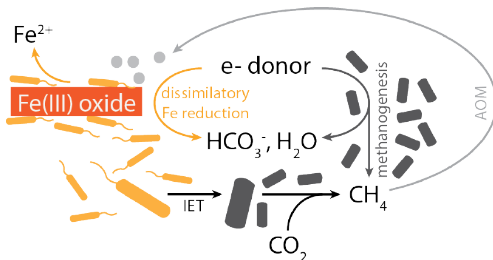
Figure 10.4 Conceptual model of potential interactions between iron reducers, methanogens, and anaerobic methanotrophic (ANME) archaea. The iron (Fe) reducers can compete with methanogens or interact syntrophically via interspecies electron transfer (IET). Where ferric iron and methane are available, it provides a potential opportunity for anaerobic oxidation of methane (AOM) by anaerobic methanotrophic (ANME) archaea.
