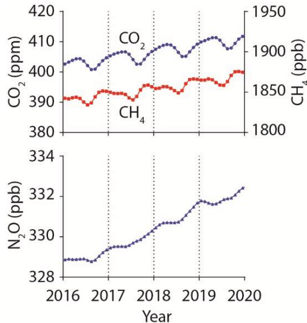
Figure 13.4 Variation in atmospheric concentrations of the abundance of carbon dioxide ( \text{CO}_2 ), methane ( \text{CH}_4 ), and nitrous oxide ( \text{N}_2\text{O} ) from 2016 to 2020. Dotted vertical lines coinciding with January 1 each year are included to highlight the seasonality of trends in concentrations of each gas. Scatter points are globally-averaged monthly means determined for marine surface sites. Units are mole fractions expressed as parts per million (ppm) for carbon dioxide and parts per billion (ppb) for methane and nitrous oxide. Data plotted are available from the U.S. National Oceanic and Atmospheric Administration ( https://gml.noaa.gov/ccag/ ). Image: https://commons.wikimedia.org/wiki/File:Greenhouse_gases_seasonal_cycles.jpg
