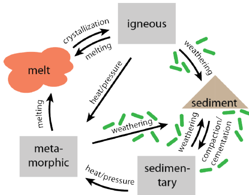
Figure 12.1 Diagram of the rock cycle. Microbial cells are included on the portions that are directly impacted by microbes. By affecting properties of sediments and sedimentary rocks, microorganisms in turn affect the feedstock for metamorphic and igneous processes. Thus, the fingerprints of microbial activity extend across the rock cycle. Note that, in addition to weathering, other processes involved in converting rocks to sedimentary deposits include erosion, transport, and deposition.
