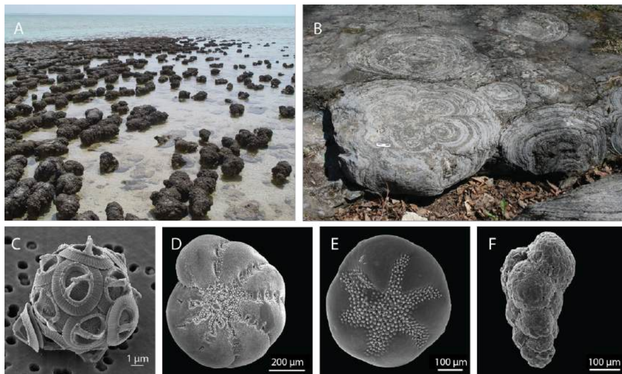
Figure 12.2 Examples of carbonate biomineralization. Image (A) shows modern marine stromatolites in Shark Bay, Western Australia, (B) shows ancient stromatolites in the Cambrian Hoyt Limestone, exposed at Lester Park, near Saratoga Springs, New York, (C) a coccolith was formed by Gephyrocapsa oceanica , and (D - F) benthic foraminifera collected from Long Island Sound.
