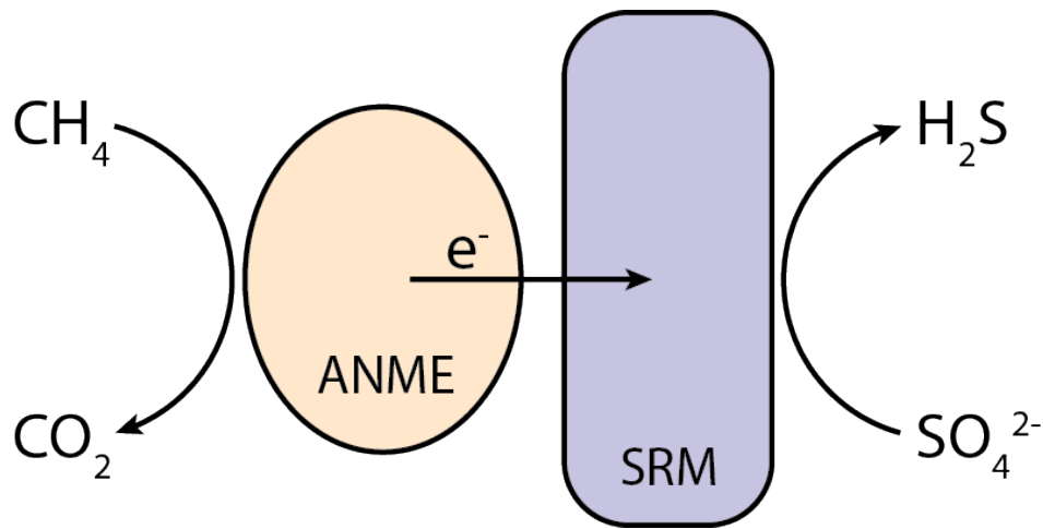
Figure 7.4 Conceptual model of interspecies electron transfer between anaerobic methanotrophs (ANME) and sulfate reducing microorganisms (SRM). This figure is based on figure 3 of Lovley (2017). https://commons.wikimedia.org/wiki/File:Electroactive_microbiology.png
