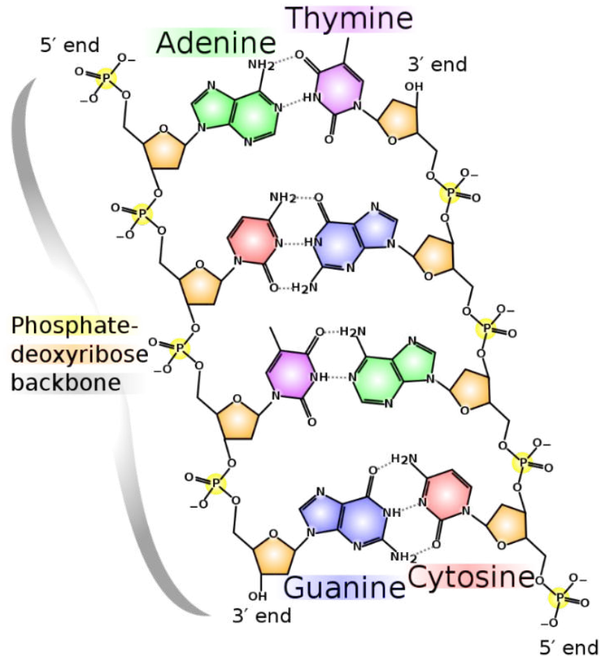
Figure 2.3 Chemical structure of DNA. Bonds between the sugar and phosphate groups of each nucleotide form the phosphate-deoxyribose backbone of each DNA strand. Hydrogen bonds between each base, shown as dotted lines, link the two strands of DNA together. Image by Madeleine Price Ball https://commons.wikimedia.org/w/index.php?curid=1848174
