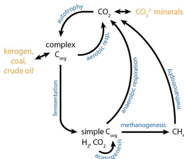
Figure 5.1 Microbial contributions to the global carbon cycle. Microbial reactions are labeled in blue font and solid phases are in orange font. C_{org} represents carbon in organic compounds. Figure based on figure 1 of Ferry (2010).
