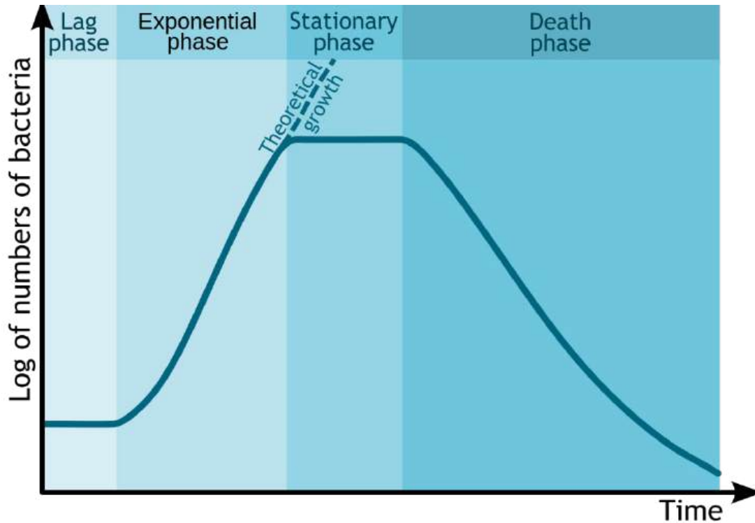
Figure 3.8 Phases of bacterial growth. Image: https://en.wikipedia.org/wiki/Bacterial_growth
