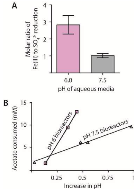
Figure 1.2 Example of the two-way interactions between microorganisms and their environment based on data from bioreactor experiments described by Paper et al. (2021). (Graph A) The pH of the environment helped steer microbial activity by affecting the proportion of iron to sulfate reduction in the experiments. (Graph B) In turn, the microbial reactions caused the pH of the bioreactor solutions to increase. Scatter points show averages for replicate reactors and lines are best-fit results of linear regressions.
