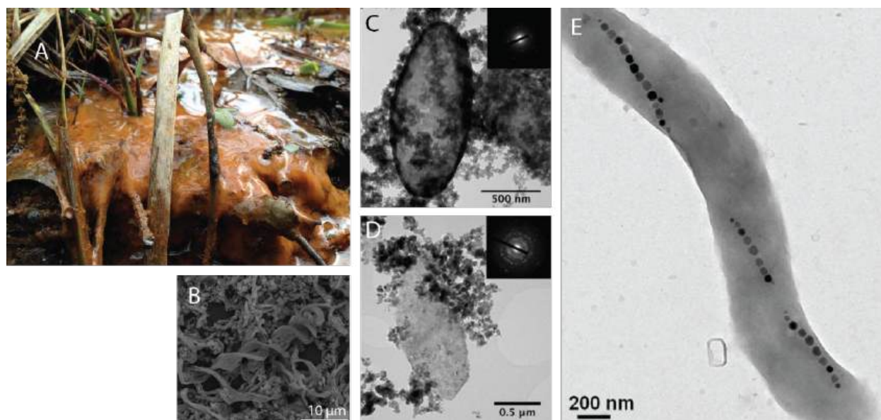
Figure 12.6 Examples of iron (oxyhydr)oxide biominerals: (A) unidentified (oxyhydr)oxides forming on biofilm (B) cell-stalk aggregates, (C) lepidocrocite and (D) magnetite (induced) encrustations on cells, and (E) magnetite magnetosomes (controlled) within a magnetotactic bacterium. The iron oxidizing biofilm shown in (A) exists at a location where groundwater discharges at the surface adjacent to a dam. Anoxic groundwater likely accumulates some ferrous iron along flow through the subsurface and, upon discharge at the surface, the ferrous iron is exposed to oxygen and can serve as an energy source for iron oxidizers. The twisted stalk visible in (B) formed in cultures of Mariprofundus sp. DIS-1. The (oxyhydr)oxides in (C) and (D) formed in cultures of the nitrate-reducing iron oxidizer Acidovorax sp. strain BoFeN1. Cells were grown under different conditions to promote development of different (oxyhydr)oxide phases. The small inset boxes show electron diffraction patterns used to identify the minerals. Image sources: (A) https://commons.wikimedia.org/wiki/File:Iron_oxyhydroxides.jpg ; (B) Koeksoy et al. (2021); (C) and (D) Miot et al. (2015); (E) Alphanbéry (2014).
