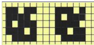
Figure 34. Five-harness satin weaves
