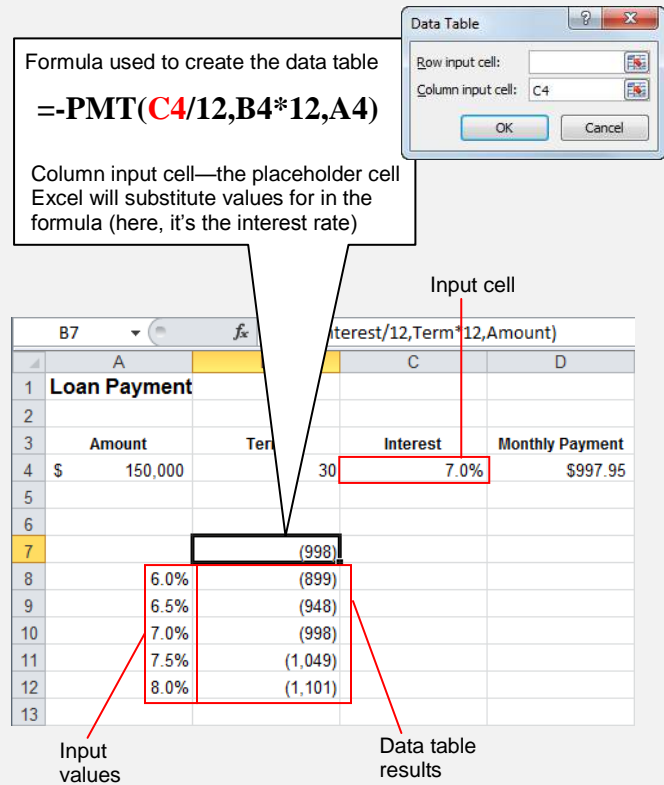
Figure 11-6: The Data Table dialog box and the resulting one-input data table showing different monthly payments at different interest rates.
