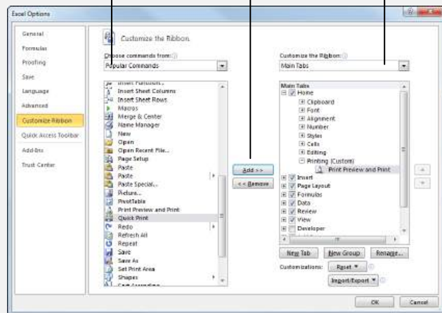
Figure 14-2: Adding commands to groups on the Ribbon.
