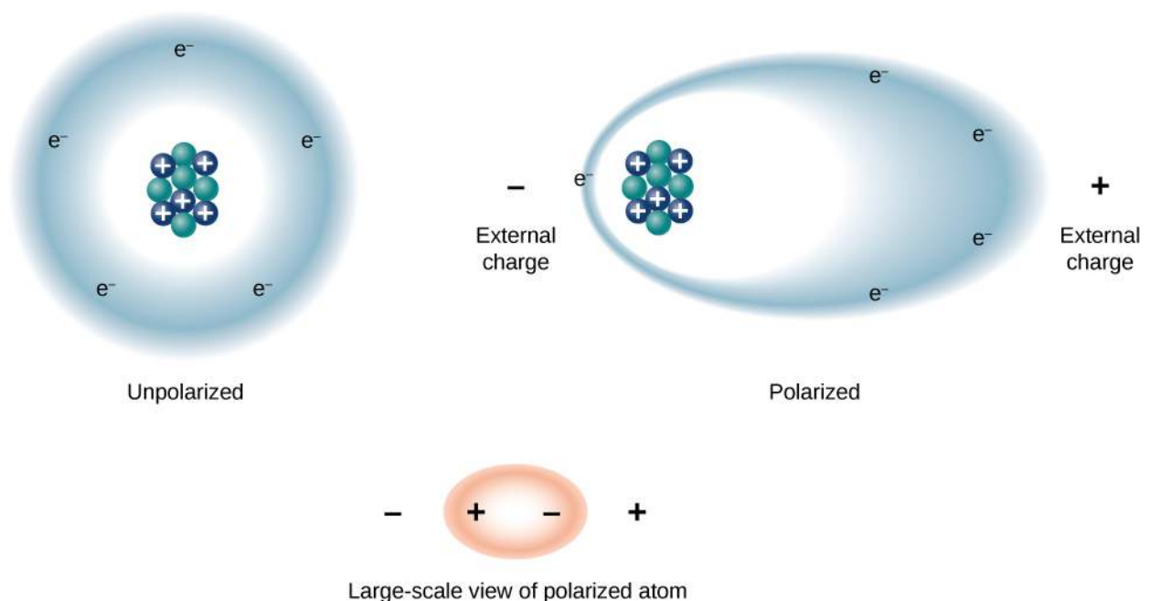
Large-scale view of polarized atom
