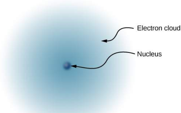
Figure 5.7 This simplified model of a hydrogen atom shows a positively charged nucleus (consisting, in the case of hydrogen, of a single proton), surrounded by an electron “cloud.” The charge of the electron cloud is equal (and opposite in sign) to the charge of the nucleus, but the electron does not have a definite location in space; hence, its representation here is as a cloud. Normal macroscopic amounts of matter contain immense numbers of atoms and molecules, and, hence, even greater numbers of individual negative and positive charges.
