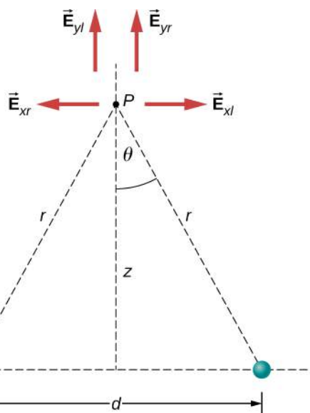
Figure 5.21 Note that the horizontal components of the electric fields from the two charges cancel each other out, while the vertical components add together.
