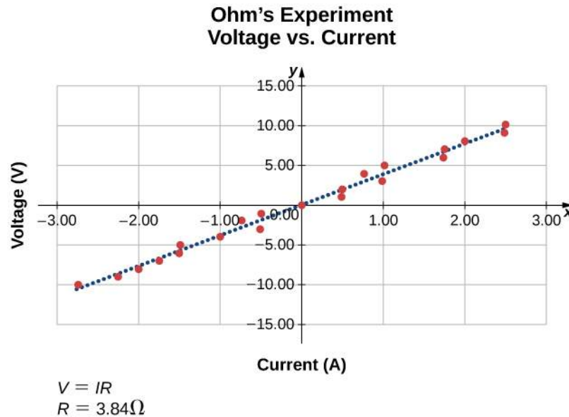
Figure 9.20 A resistor is placed in a circuit with a battery. The voltage applied varies from -10.00\text{ V} to +10.00\text{ V} , increased by 1.00\text{-V} increments. A plot shows values of the voltage versus the current typical of what a casual experimenter might find.
