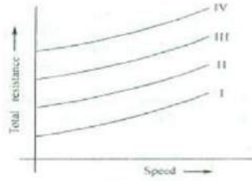
Fig. 5.8 (b) Total resistance V/s speed on different gradients.
