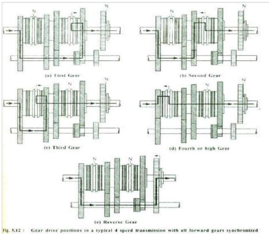
Fig. 5.12 : Gear drive positions in a typical 4 speed transmission with all forward gears synchronized
