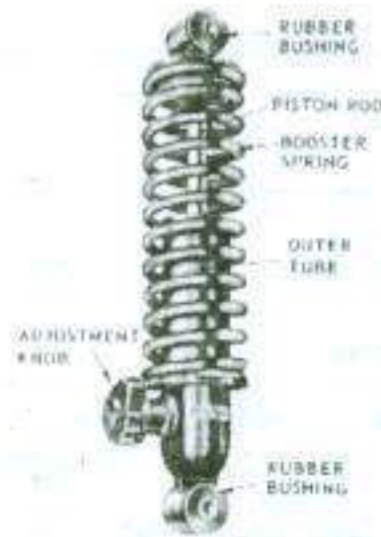
Fig. Shock absorber
