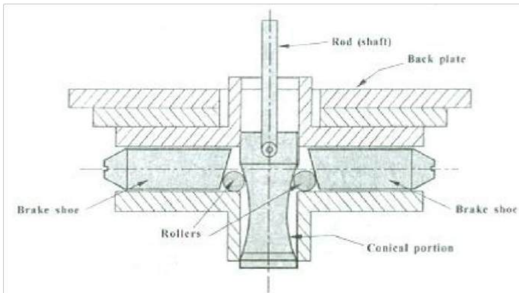
Fig Expander
