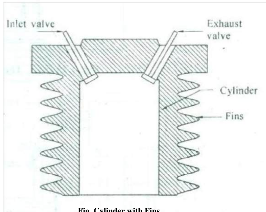
Fig. Cylinder with Fins
