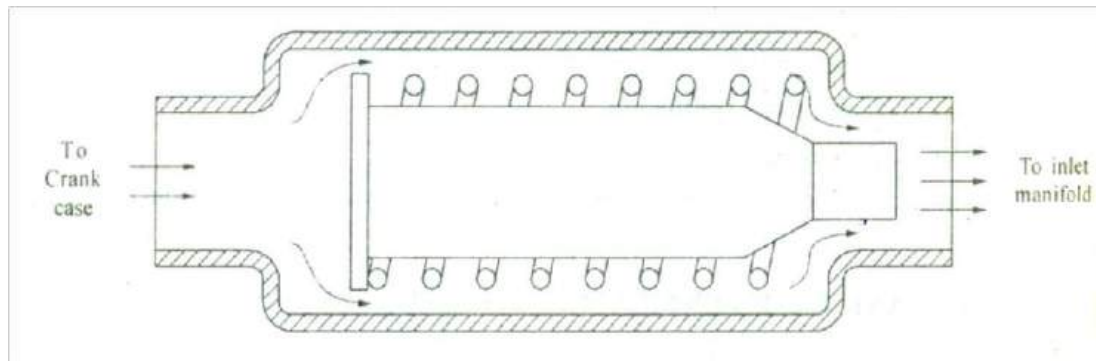
Fig.PCV Valve
