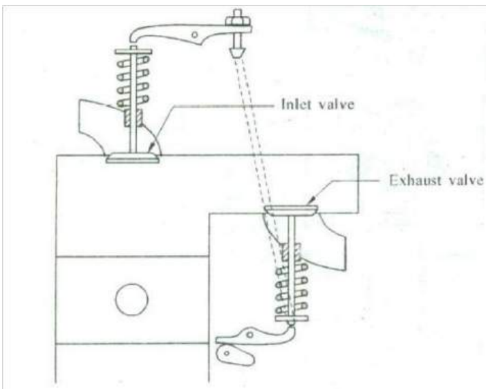
Fig. (c) Overhead inlet and side exhaust mechanism
