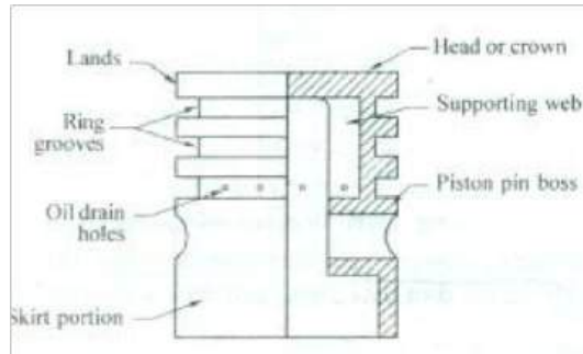
Fig. Typical I.C, engine piston
