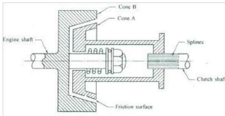
Fig.Cone clutch
