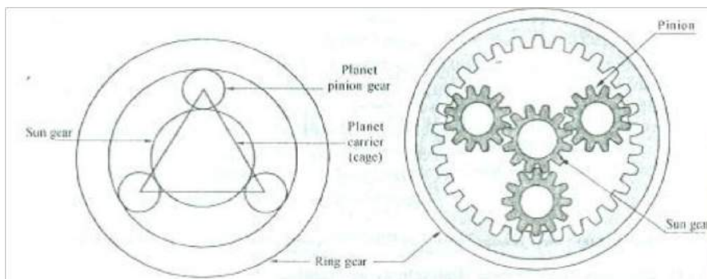
(a) Simplified view of planetary gear system
