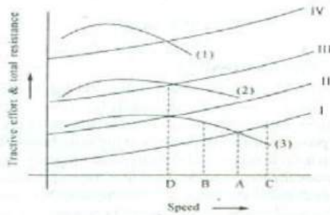
Fig. 5.8 (d) Total resistance and tractive effort curves at different gears.
