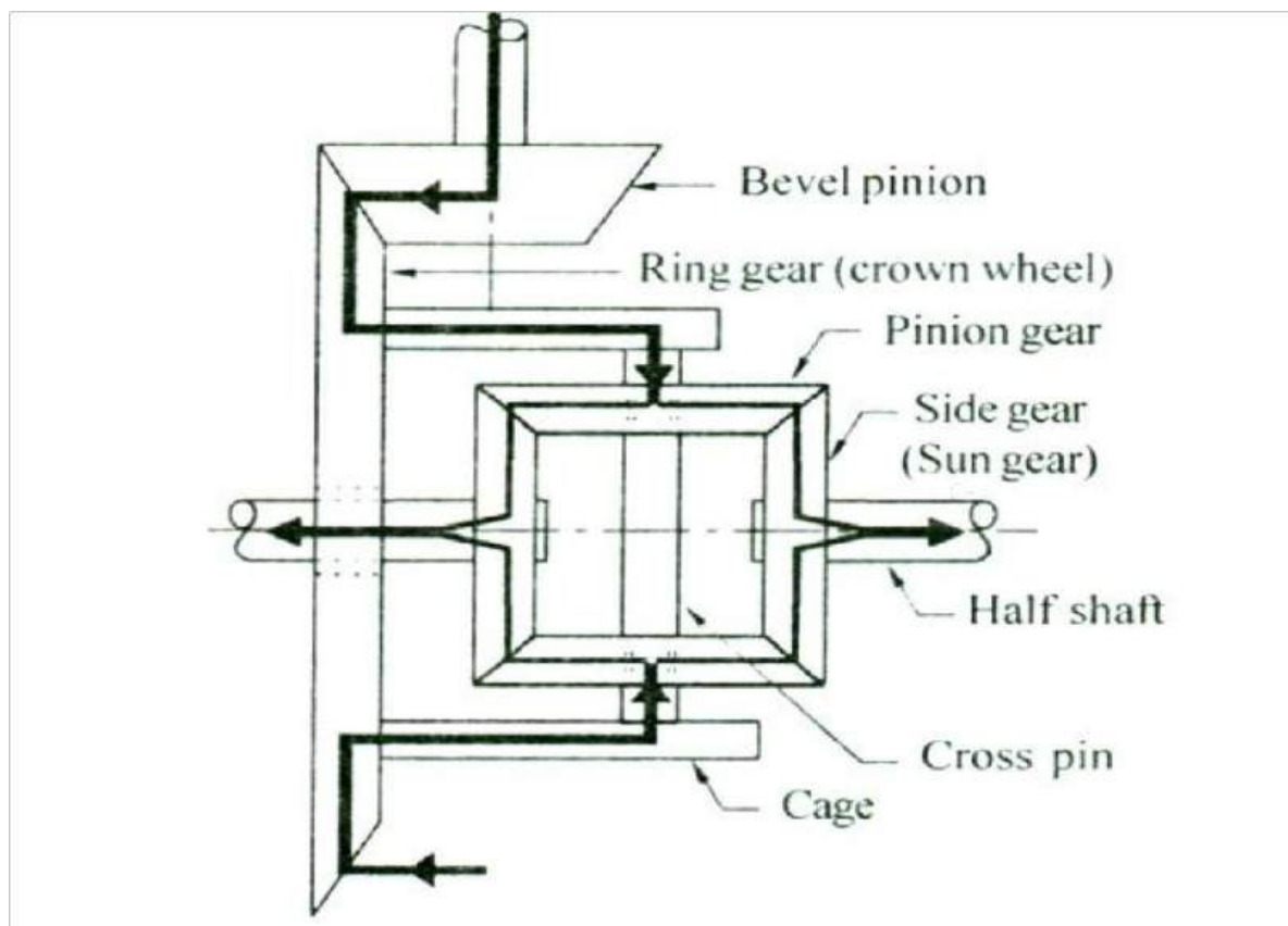
Fig (d) Axle side gear move forward at different speeds. Pinion gear (3) is turning
