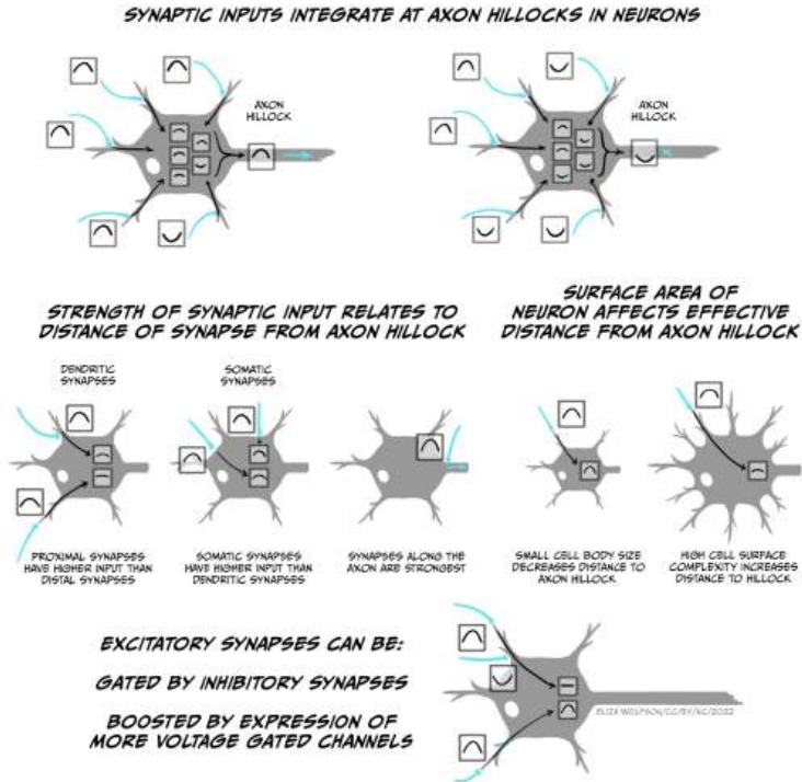
Fig 3.32 Synaptic integration
