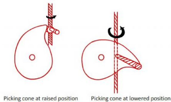
Figure 7.4: Adjusting the position of picking cone
