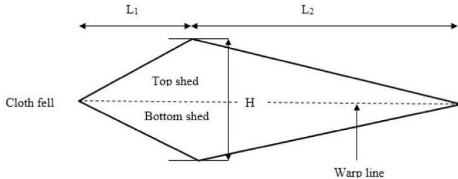
Figure 6.7: Geometry of shed
