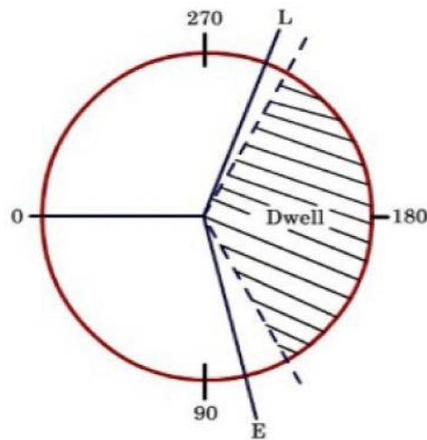
Figure 6.11: Timing for late shedding
