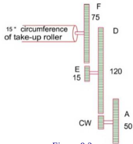
Figure 9.2: Five-wheel take-up motion
