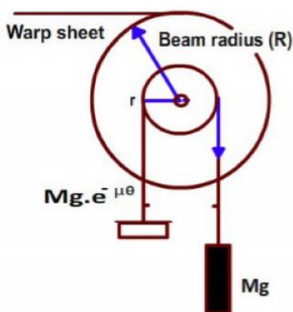
Figure 4.18: Warp tension control by dead weight system
