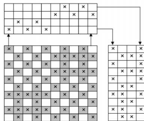
Figure 5.27: Design, drafting and lifting plan of Huck-a-back weave
