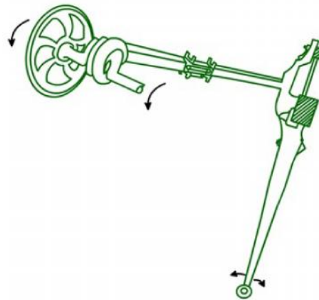
Figure 8.1: Sley motion
