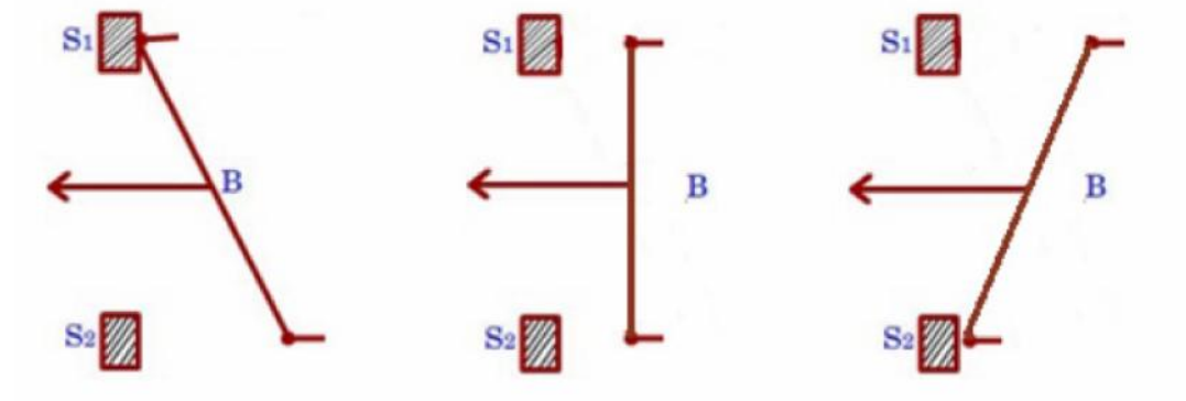
Figure 6.36: Open shed formation in Keighley dobby
