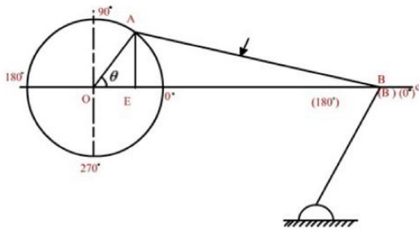
Figure 8.2: Schematic diagram of sley motion
