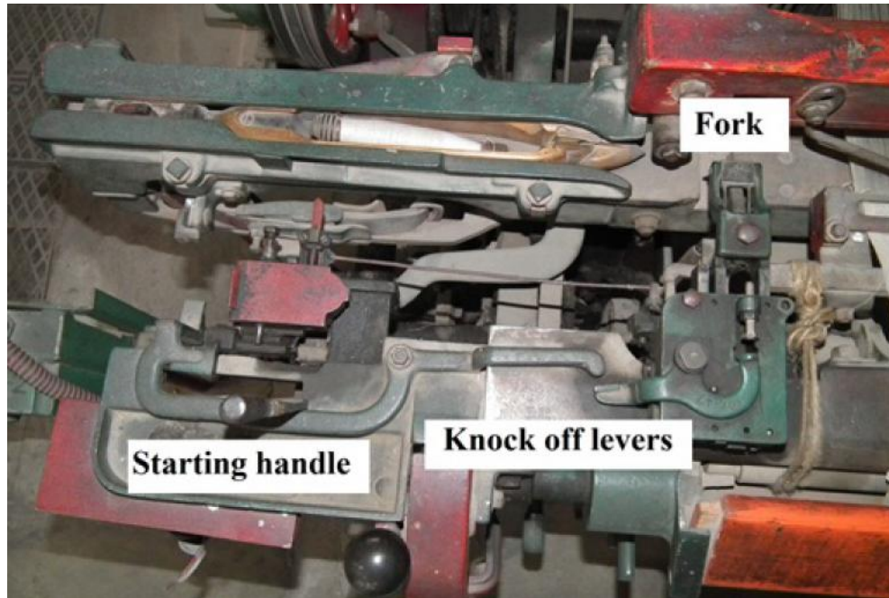
Figure 9.15: Top view of side weft fork motion
