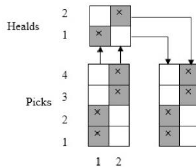
Figure 5.7: Design, drafting and lifting plan of warp rib
