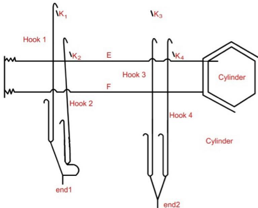
Figure 6.42: Side view of double-lift single-cylinder jacquard
