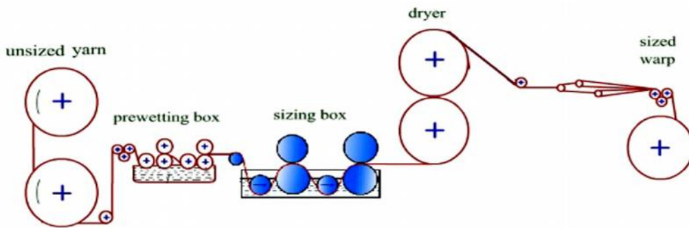
Figure 4.36: Simplified representation of pre-wetting process
