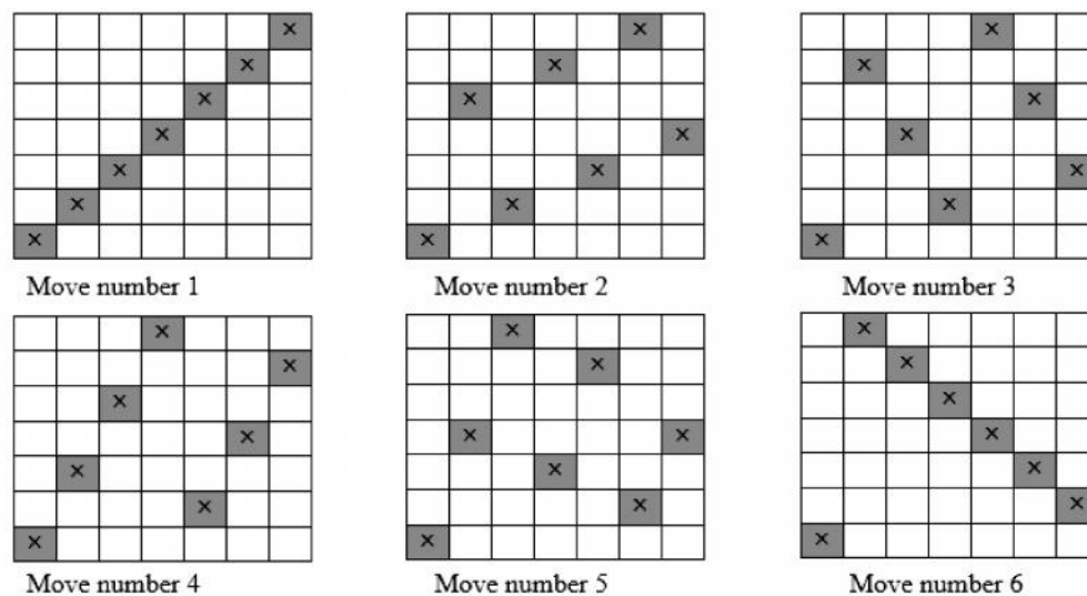
Figure 5.20: Seven-end sateen with various move numbers
