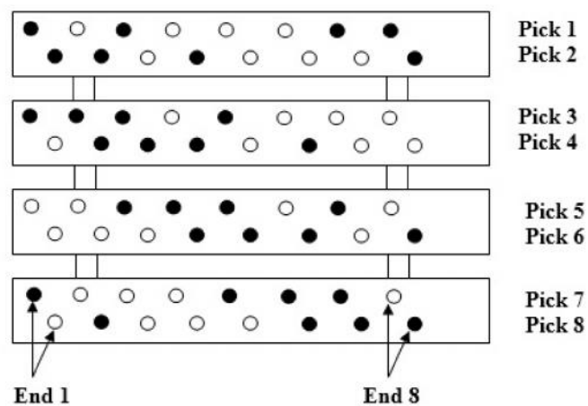
Figure 6.38: Peg plan for 3/3/1/1 twill weave
