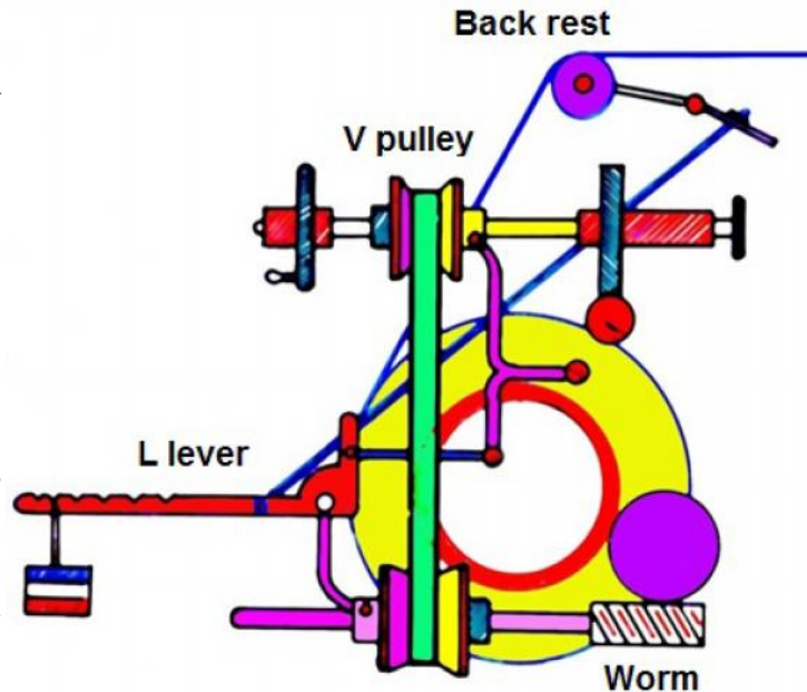
Figure 9.8: Hunt positive let-off motion
