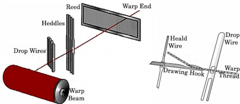
Fig: Schematic Diagram of Drawing in
