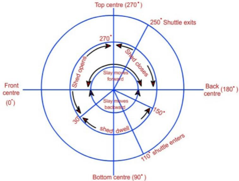
Figure 7.1: Loom timing diagram for shuttle loom (early shedding)
