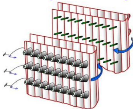
Figure 3.5: Swivelling creel
