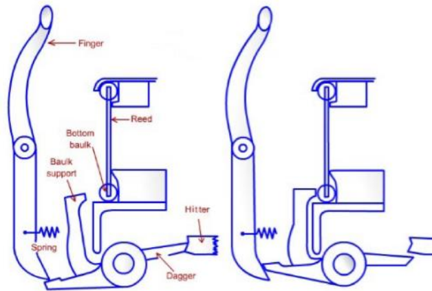
Figure 9.11: Loose-reed warp protector motion
