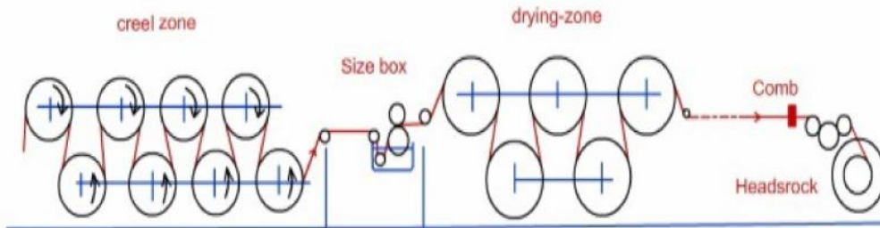
Figure 4.13: Zones of a sizing machine
