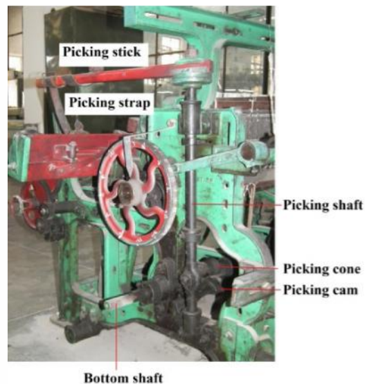
Figure 7.3: Cone over-pick mechanism on a loom
