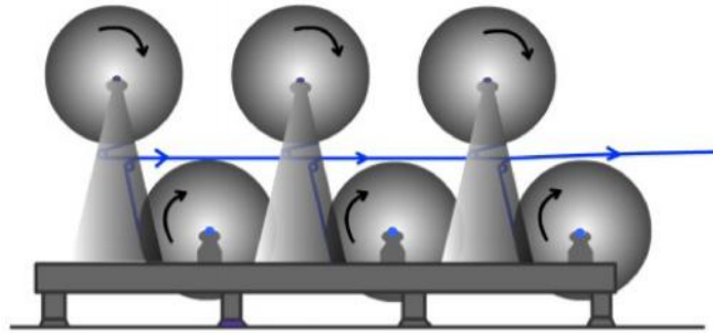
Figure 4.16: Equi-tension creel
