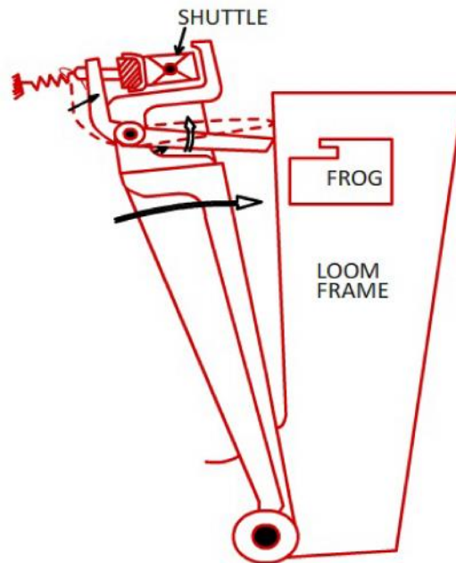
Figure 9.10: Fast-reed warp protector motion
