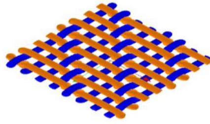
Figure 5.14: Interlacement pattern in 3/1 twill weave (warp: orange and weft: blue)
