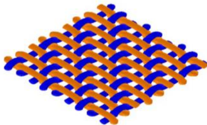
Figure 5.13: Interlacement pattern in 2/1 twill weave (warp: orange and weft: blue)
