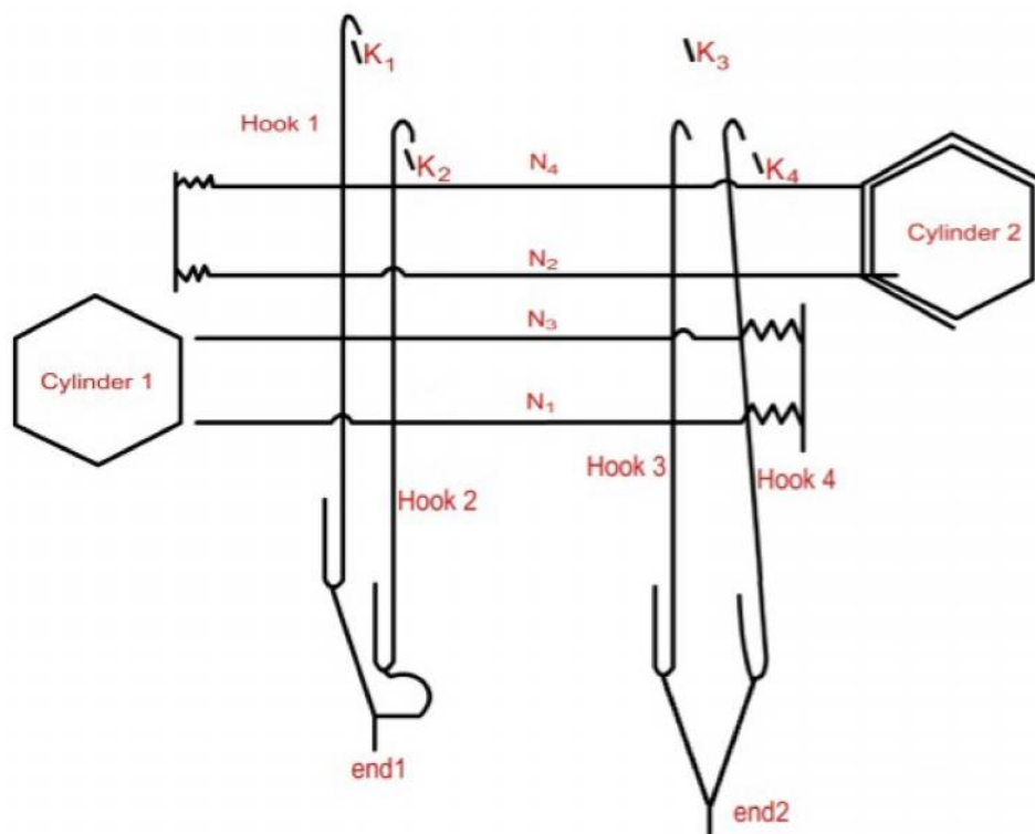
Figure 6.43: Side view of double-lift double-cylinder jacquard
