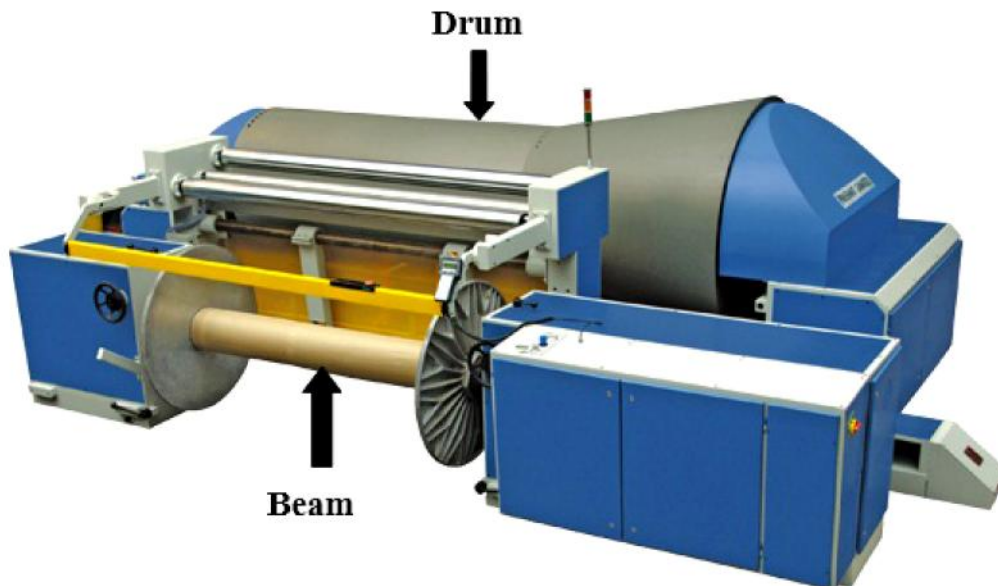
Figure 3.10: Sectional warping drum and beam
