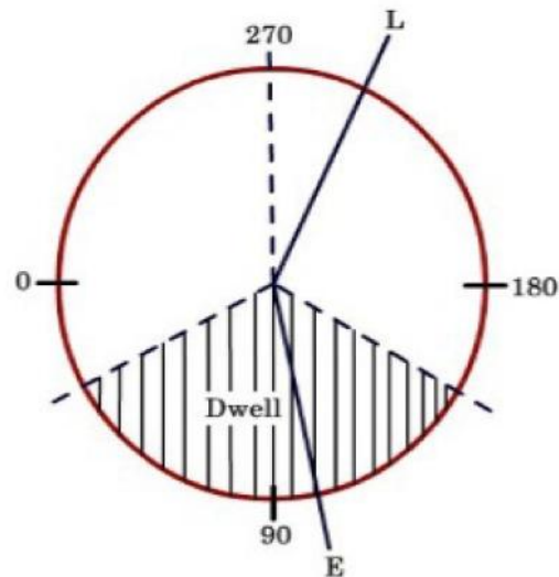
Figure 6.10: Timing for early shedding
