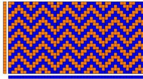
Figure 5.16: Extended view of pointed twill
