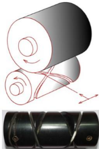
Figure 2.5: Drum-driven winder and grooved drum
