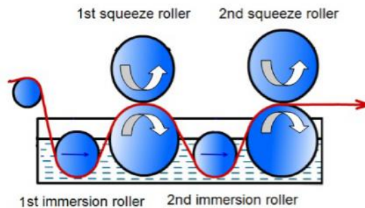
Figure 4.20: Two dip two nip size box
