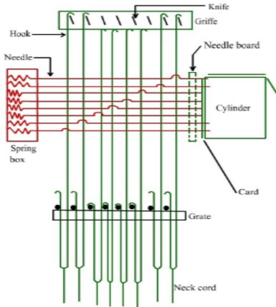
Figure 6.41: Side view of single-lift single-cylinder jacquard
