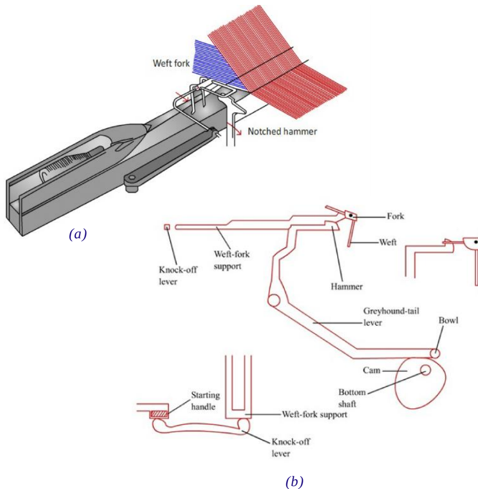
Figure 9.14: (a) Side fork and notched hammer (b) Side view of side weft fork motion
