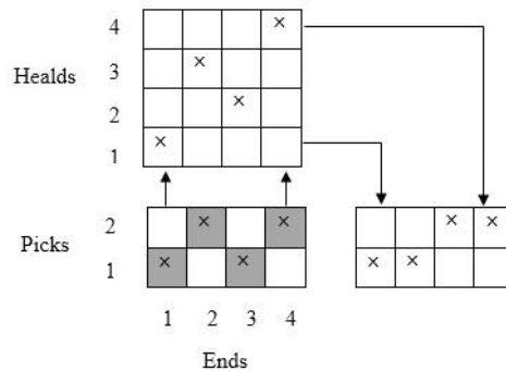
Figure 5.3: Skip draft
