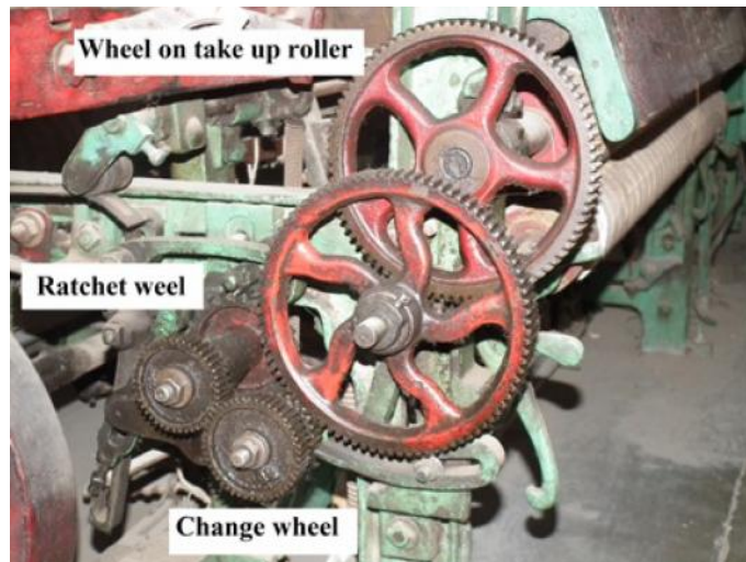
Figure 9.3: Seven-wheel take-up motion (a) Schematic (b) Mounted on loom
