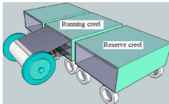
Figure 3.3: Single end truck creel
