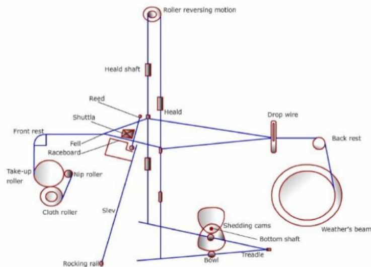
Figure 6.2: Cross-sectional view of loom
