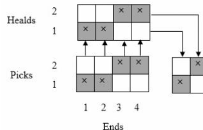
Figure 5.9: Design, drafting and lifting plan of weft rib
