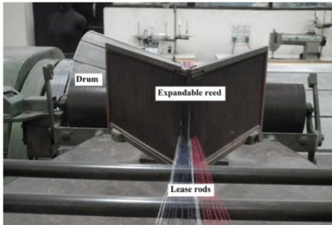
Figure 3.9: Expandable reed and lease rods
