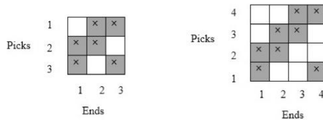
Figure 5.12: Warp faced (2/1) twill and balanced (2/2) twill
