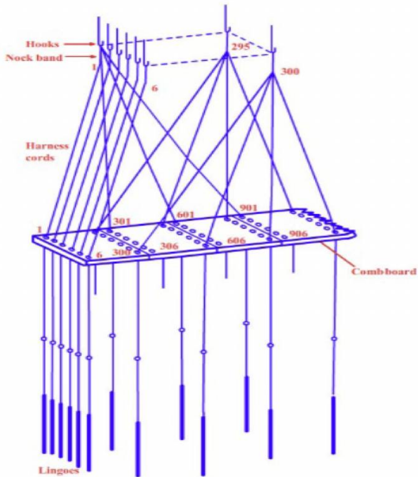
Figure 6.44: Jacquard harness
