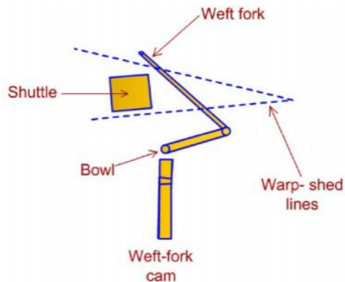
Figure 9.16: Center-weft fork
