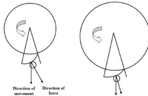
Figure 6.34: Influence of cam dimension on the steepness of cam contour
