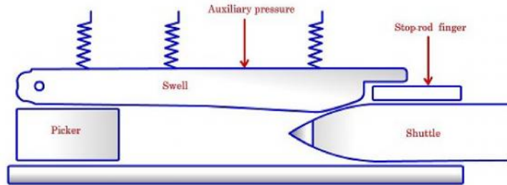
Figure 7.19: Checking of shuttle
