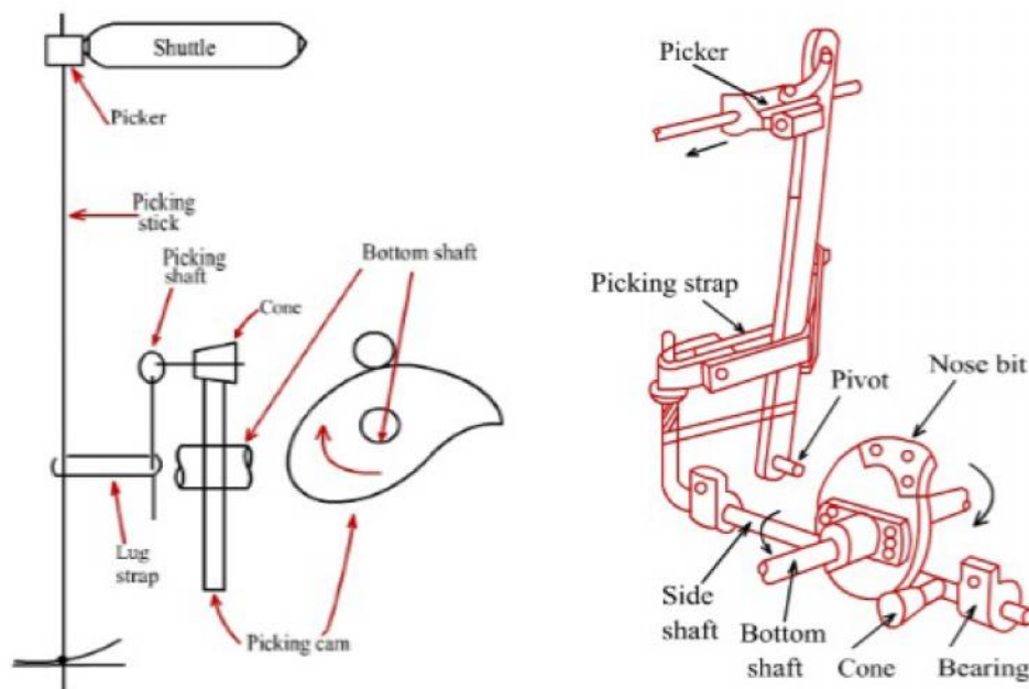
Figure 7.5: Cone under-pick mechanism
