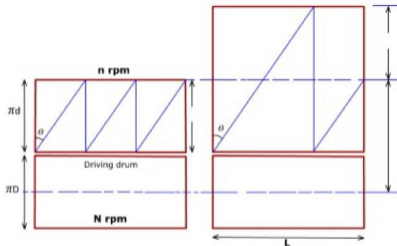
Figure 2.8: Principles of drum-driven winder
