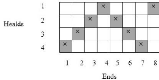
Figure 5.2: Pointed draft
