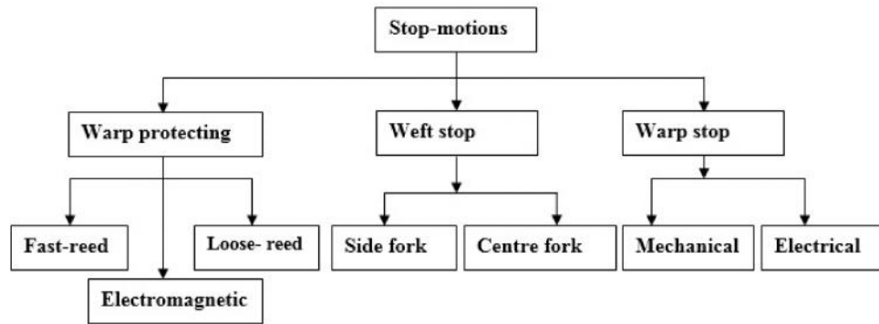
Figure 9.9: Classification of stop-motions
