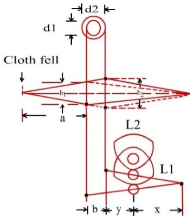
Figure 6.6: Lift of the cams and movement of the healds
