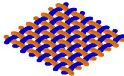
Figure 5.5: Interlacement pattern of plain weave (warp: orange and weft: blue)
