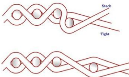
Figure 6.13. (a) Vertical displacement of newly inserted weft (b) Beat up at crossed shed
