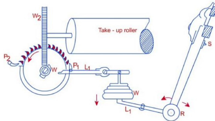
Figure 9.1: Negative take-up motion
