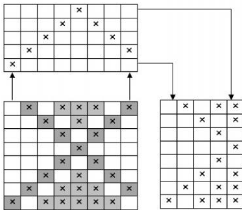
Figure 5.23: Design, drafting and lifting plan of Honeycomb weave
