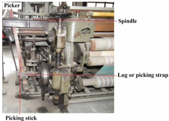
Figure 7.6: Cone under-pick mechanism on a loom
