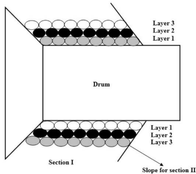
Figure 3.6: Schematic representation of sectional warping principle
