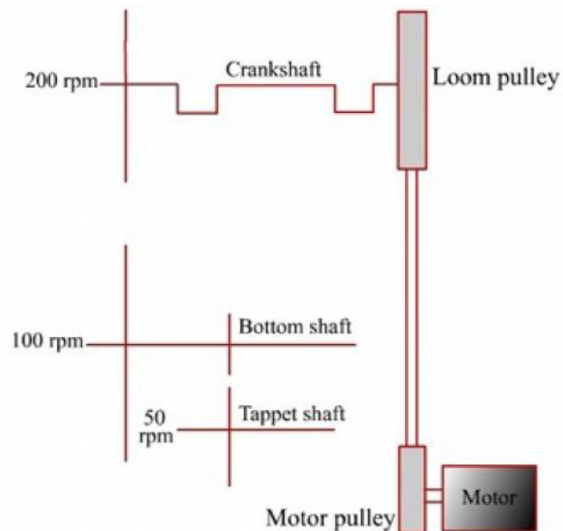
Figure 6.1: Transmission of motions in loom
