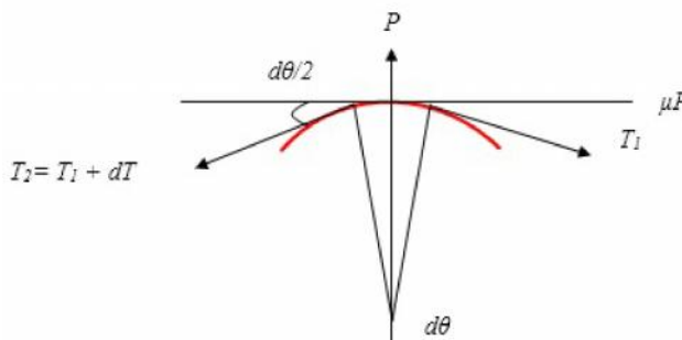
Figure 2.32: Schematic representation of yarn passing over a curved surface
