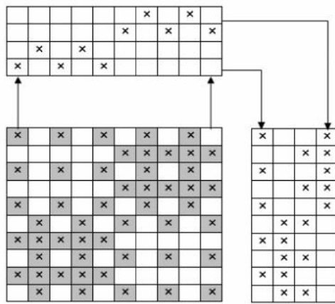
Figure 5.25: Design, drafting and lifting plan of Mock leno weave
