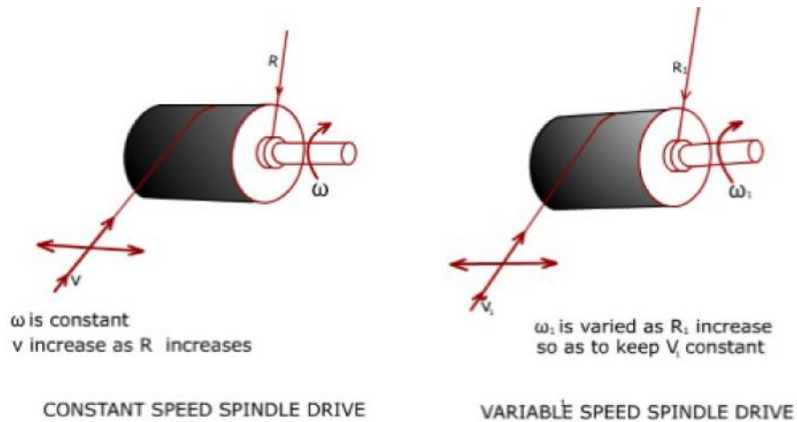
Figure 2.7: Spindle-driven winders
