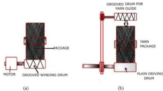
Figure 2.6: Types of drum-driven winder (a: grooved drum, b: plain drum)
