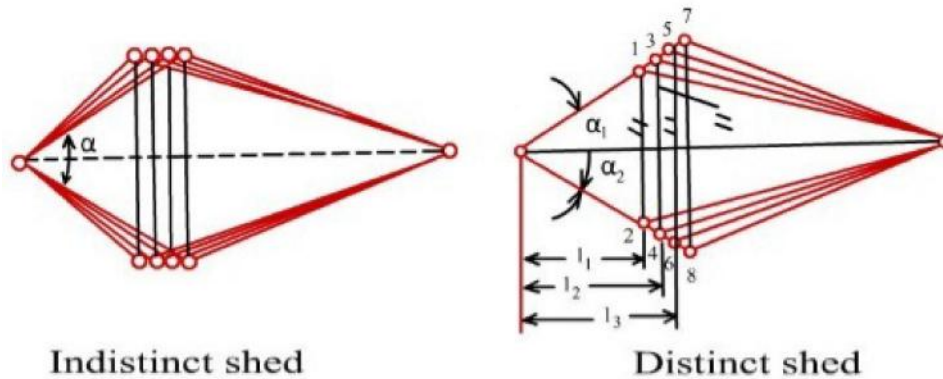
Figure 6.5: Indistinct (unclear) and distinct (clear) sheds
