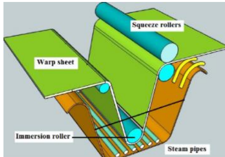
Figure 4.19: One dip one nip size box
