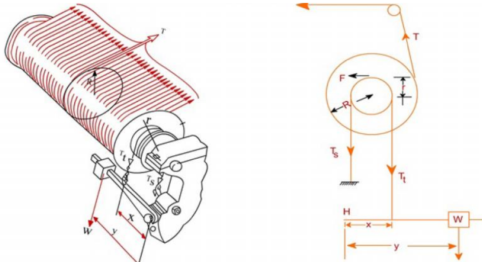
Figure 9.6: Negative let-off motion
