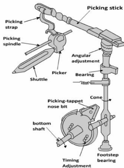
Figure 7.2: Cone over-pick mechanism
