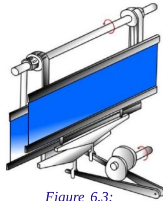
Figure 6.3: Cam shedding system
