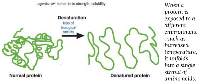
Figure 6.6 Protein Denaturation
