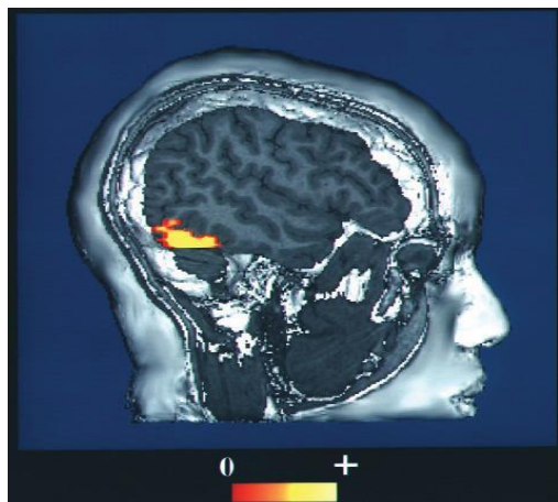
Figure 3.14 fMRI Image
