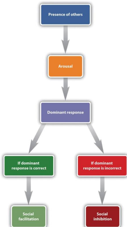
Figure 9.16 Drive-Arousal Model
