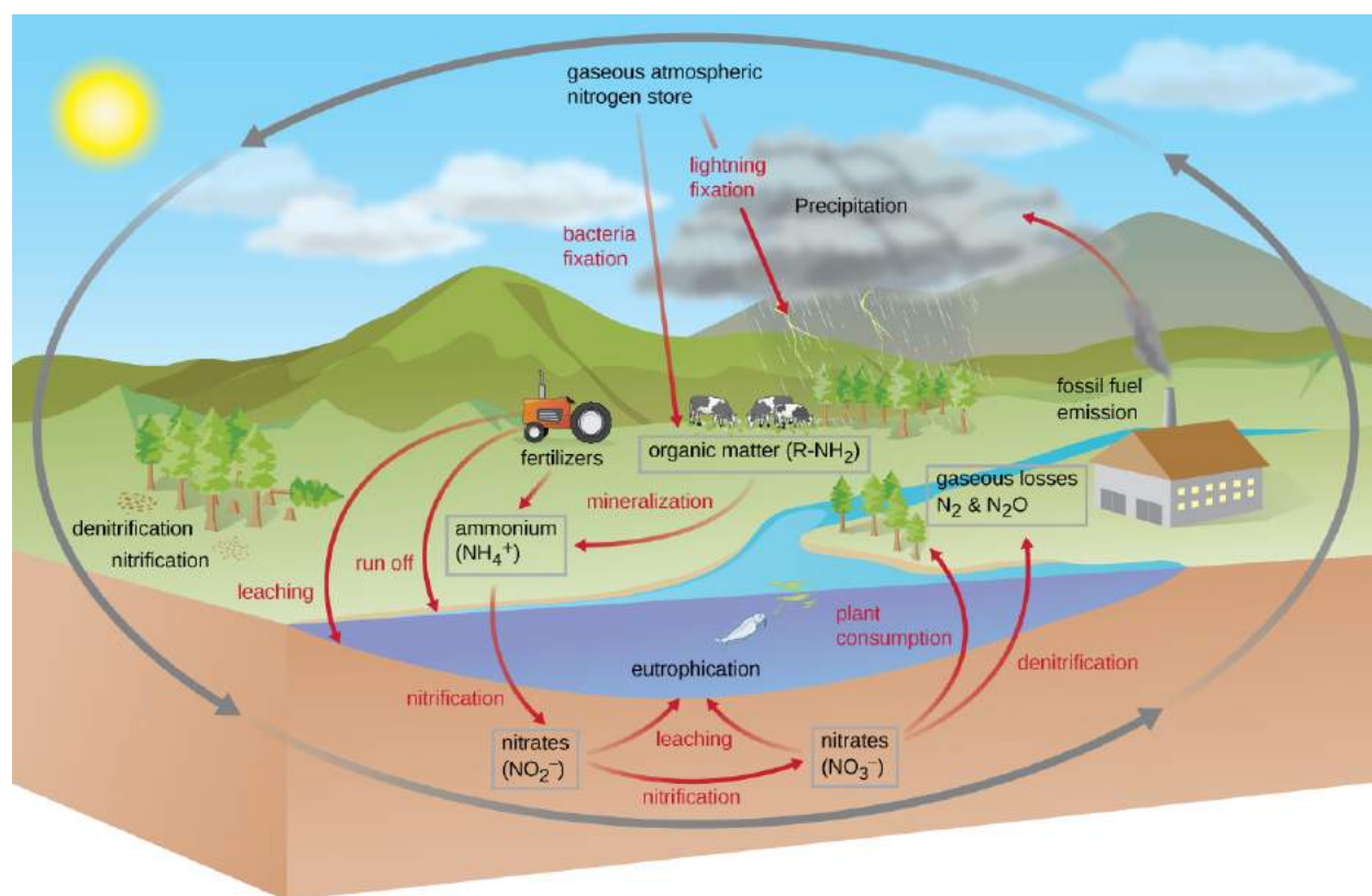
Nitrogen cycle
