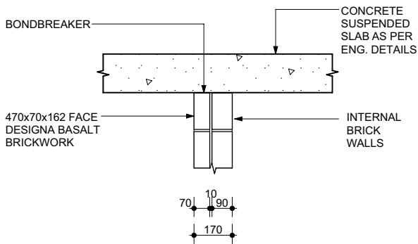
Figure 13 – Typical Internal Wall Suspended Slab Detail
