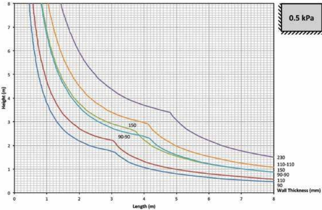
Chart 4 – Wall is laterally supported from one end only
