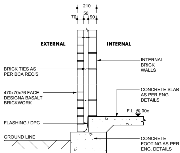
Figure 7 – Typical Footing Connection
