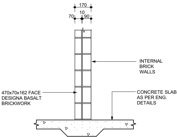
Figure 14 – Typical Internal Wall Detail
