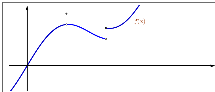
Figure 3.7: Upper semicontinuity.
