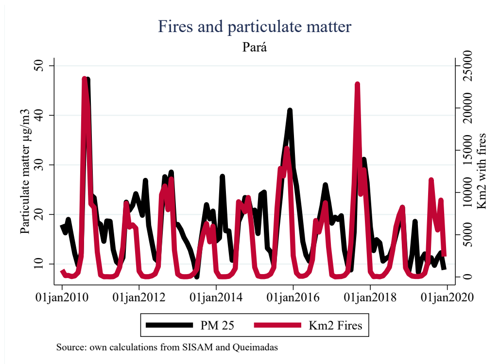
Figure 3: Fires are highly correlated with concentration of PM
