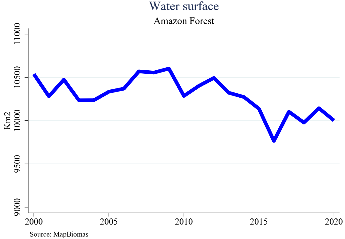
Figure 4: Water surface is 8% lower than the average pre-2010
