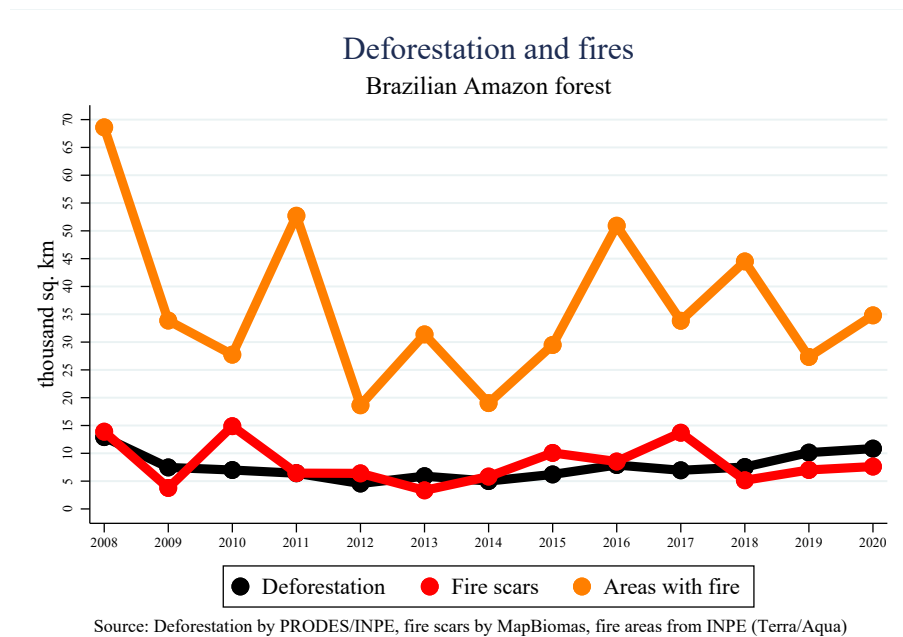
Figure 2: Degradation by fires
