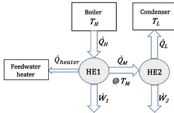
Figure 6.1.e2 Schematic of the two-stage heat engine
