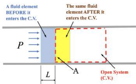
Figure 2.2.4 Flow work
