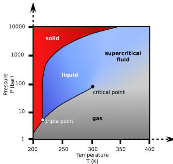
Figure 2.3.3 P - T diagram for CO 2
