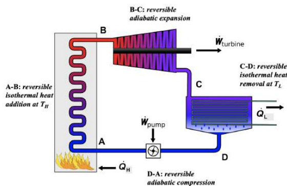
Figure 6.4.2 Carnot heat engine
