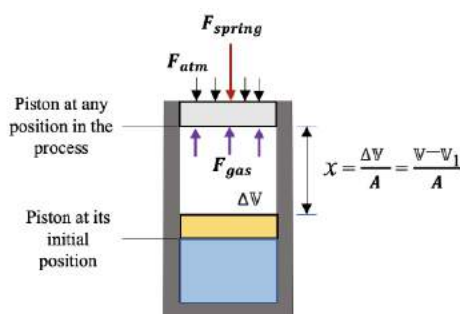
Figure 4.3.e6 Forces acting on the piston in equilibrium
