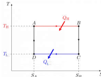
Figure 6.4.4 Carnot heat engine: T - S diagram
