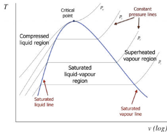
Figure 2.3.4 T-v diagram
