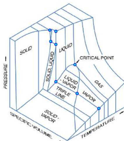
Figure 2.3.1 Pressure-specific volume-temperature (P-v-T) diagram
