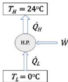
Figure 6.4.e2 Schematic of a heat pump
