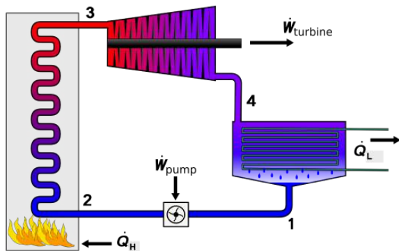
Figure 6.1.1 Rankine cycle
