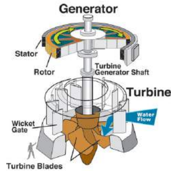
Figure 5.3.1 Hydraulic turbine
