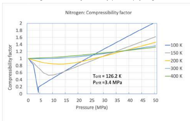
Figure 3.2.2 Compressibility factor of nitrogen
