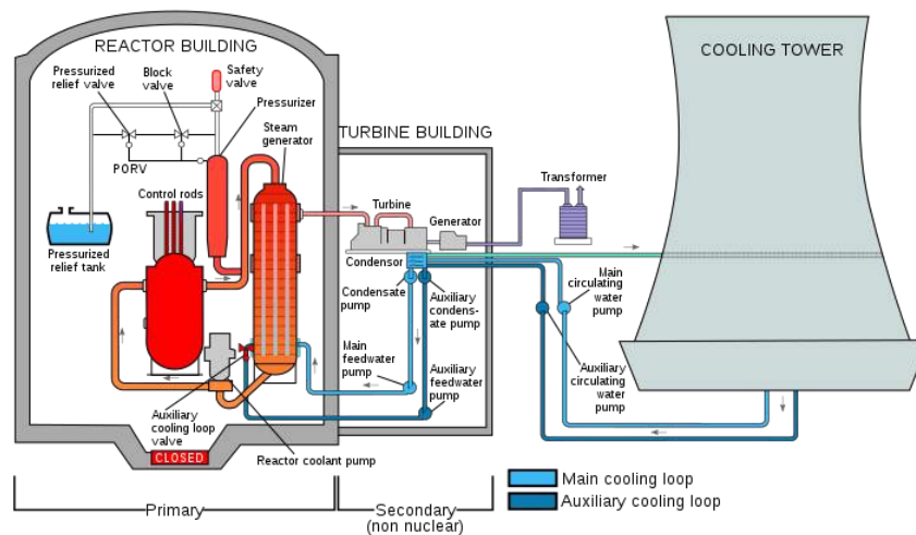
Figure 1.1.3 Nuclear Power Plant
