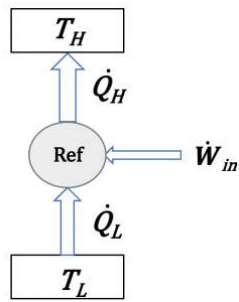
Figure 6.2.2 Schematic of a refrigerator (reproduced)
