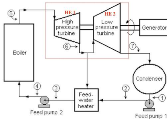
Figure 6.1.e1 Two-stage steam turbine with a feed-water heater
