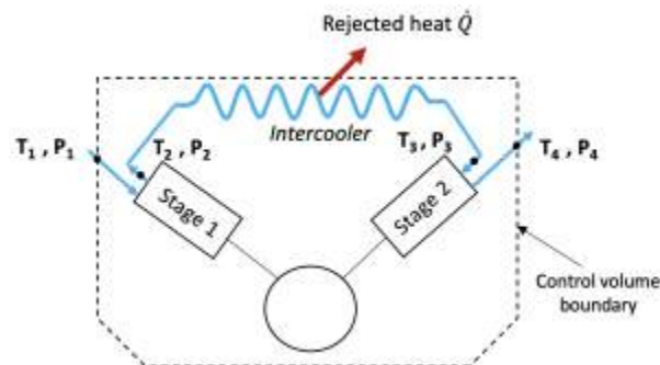
Figure 6.10.e4 Schematic of a two-stage compressor with an intercooler
