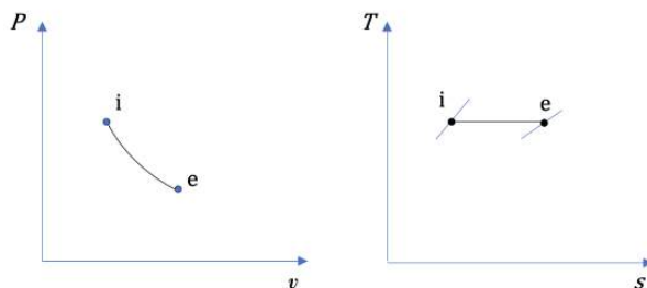
Figure 6.9.e1 T-s and P-v diagrams of a reversible process for an ideal gas
