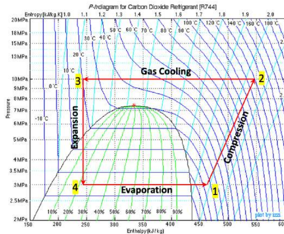
Figure 5.3.e1 P-h diagram for CO 2
