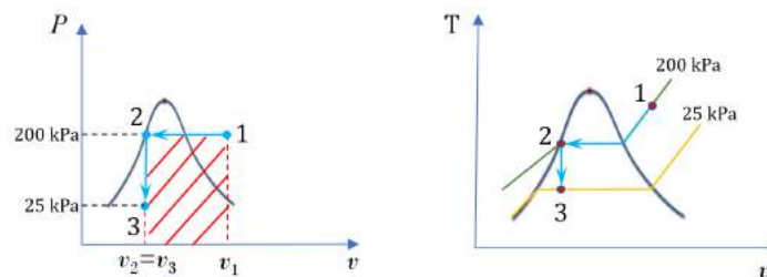
Figure 4.4.e5 P-v and T-v diagrams of the whole process
