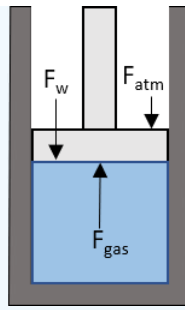
Figure 2.2.e1 Piston cylinder device showing acting forces
