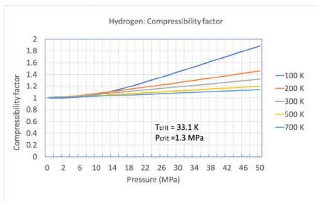
Figure 3.2.1 Compressibility factor of hydrogen
