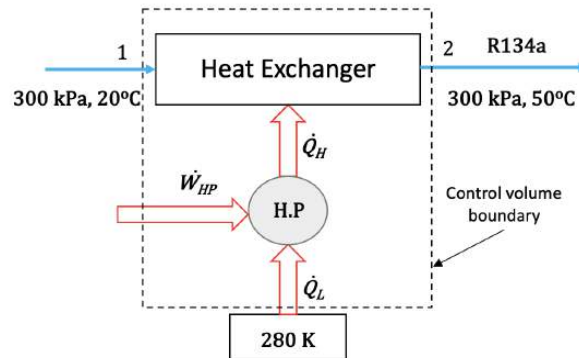
Figure 6.10.e2 A device consisting of a heat exchanger and a heat pump
