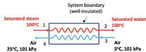
Figure 6.10.e1 Well-insulated heat exchanger
