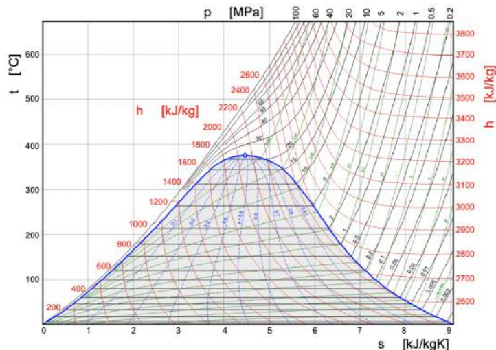
Figure 6.7.1 T-s diagram for water
