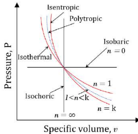
Figure 4.3.4 Different processes of an ideal gas
