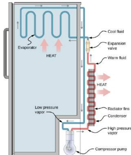
Figure 1.4.2 Refrigerator working on the vapour compression cycle
