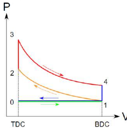
Figure 1.4.5 Four-stroke combustion engine
