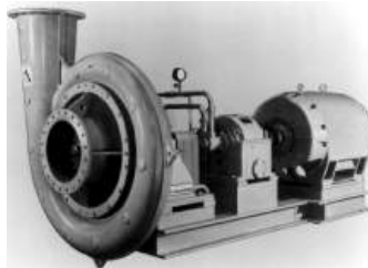
Figure 5.3.3 Centrifugal compressor
