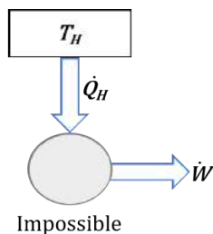
Figure 6.3.1 Schematic illustrating Kelvin-Planck statement
