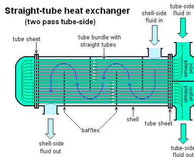
Figure 5.3.11 Schematic of a straight tube heat exchanger
