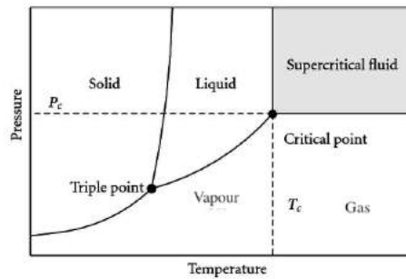
Figure 2.3.2 P - T diagram
