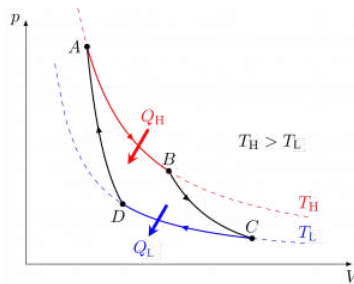
Figure 6.4.3 Carnot heat engine: P - V diagram
