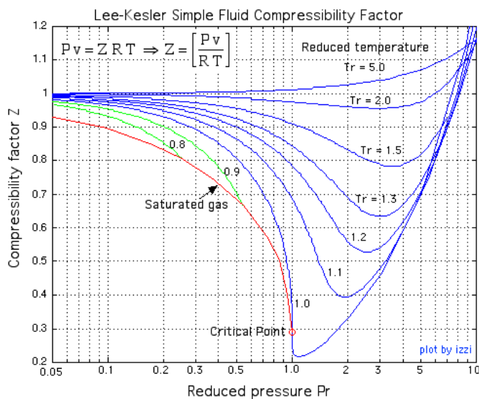
Figure 3.2.3 Lee-Kesler simple fluid compressibility factor
