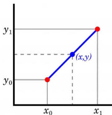
Figure 2.4.4 Linear interpolation
