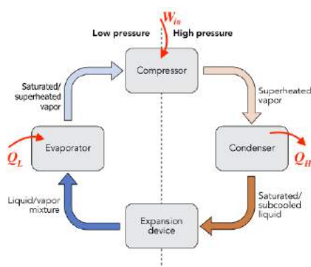
Figure 4.4.e1 Vapor compression refrigeration cycle consisting of a compressor, condenser, expansion device, and evaporator
