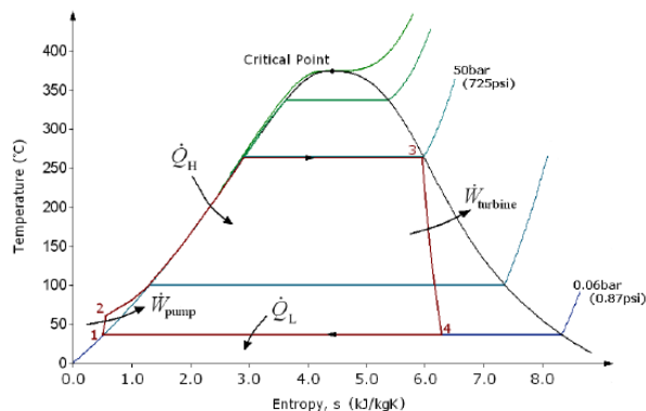
Figure 6.1.2 T - s diagram of a Rankine cycle
