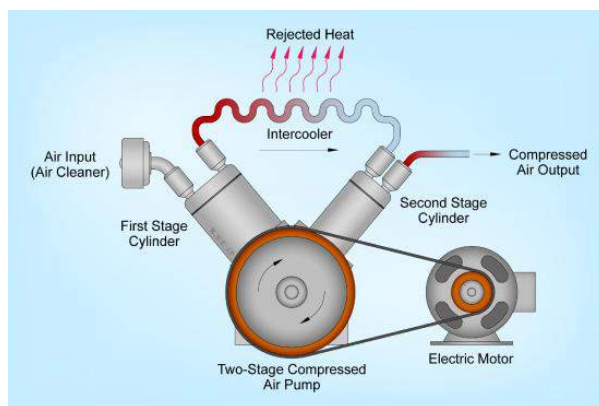
Figure 6.10.e3 Two stage compressor with an intercooler
