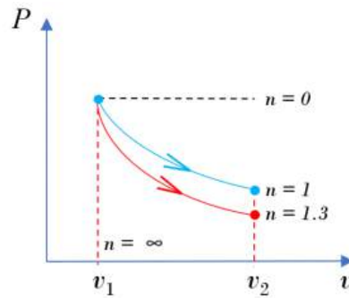
Figure 4.3.e4 Polytropic processes of an ideal gas illustrated on the P-v diagram
