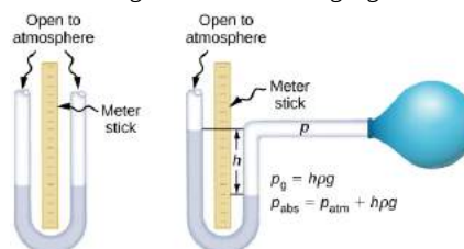
Figure 2.2.3 U-tube Manometer
