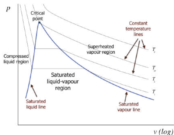
Figure 2.3.5 P-v diagram
