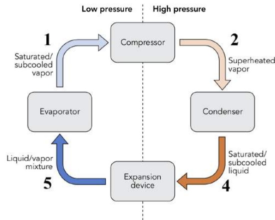
Figure 1.4.3 Vapour compression cycle
