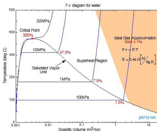
Figure 3.1.1 T-v diagram for water
