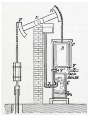
Figure 1.1.1 Watt's heat engine
