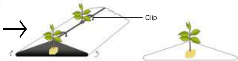
Figure 6: Basic structures of a NFT channel
