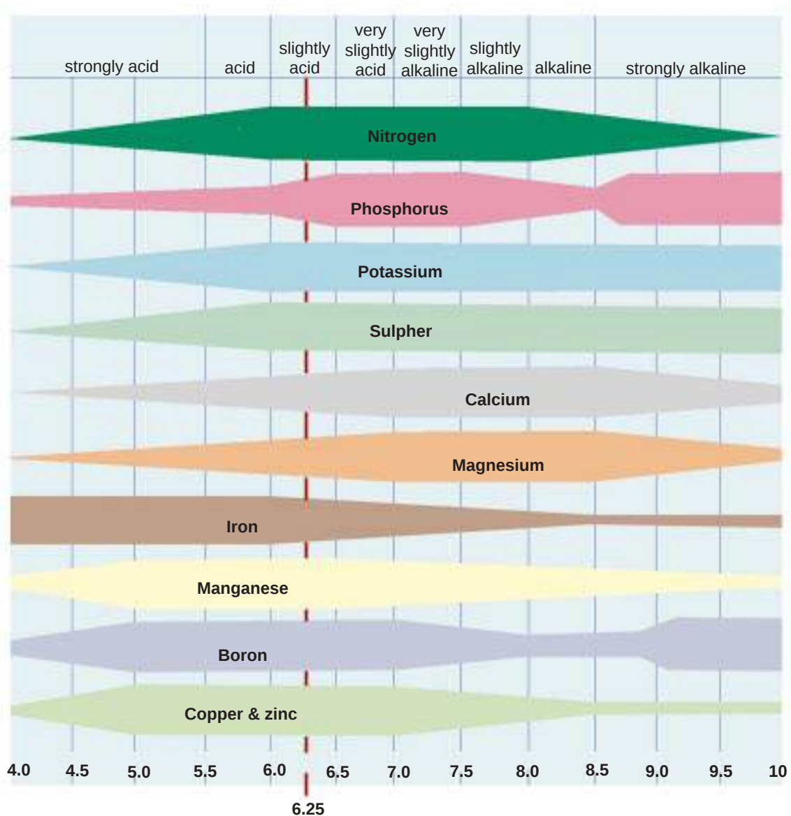
Figure 40: Chart showing the availability of nutrient elements at different pH levels.
