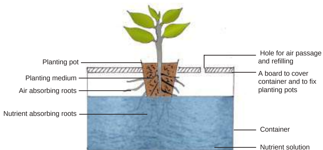
Figure 14: Diagrammatic view of a non-circulating hydroponics non-root tuber plant
