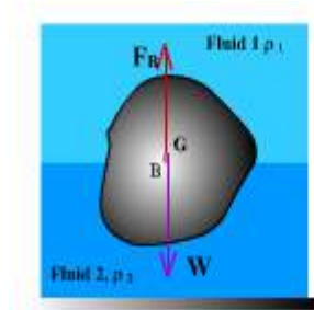
Fig. L-10.2: Buoyant force in a layered fluid
