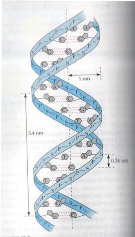
Figure 2. DNA Structure
