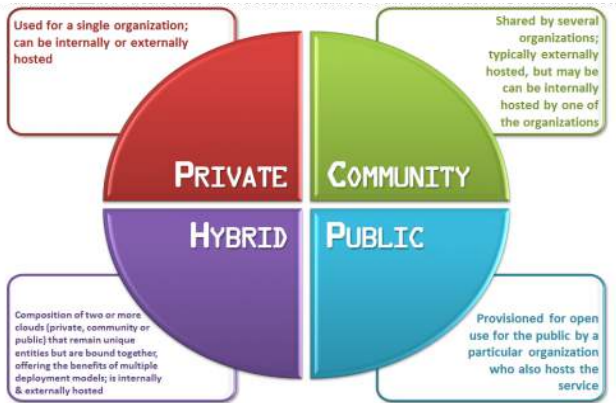
Figure 3: Deployment Models
