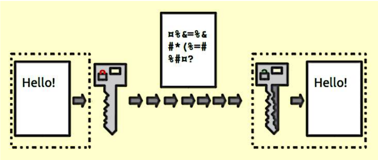
Figure 4: Encryption 2
