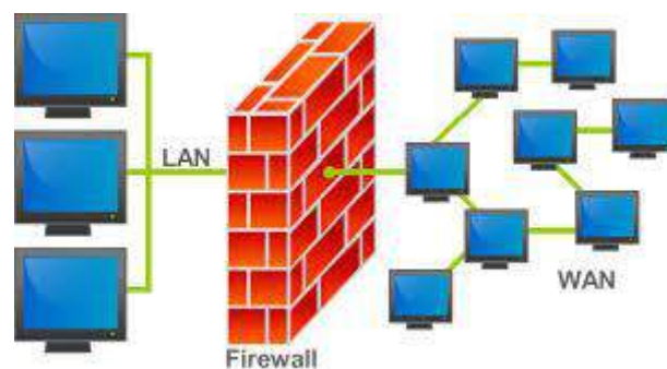
Figure 7: Firewall 5
